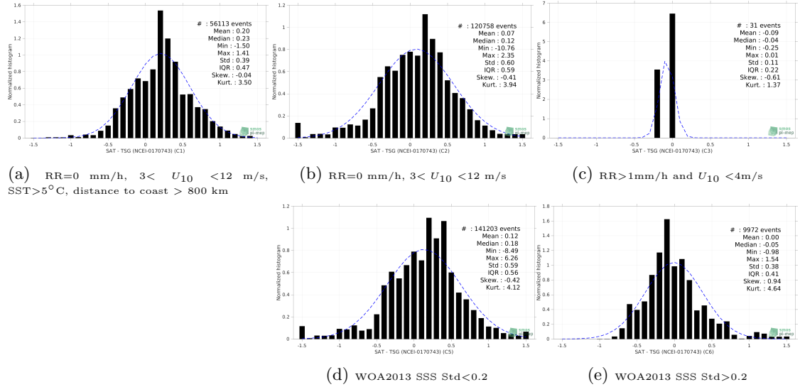
Figure 13: Normalized histogram of \Delta SSS (SMAP SSS L3 v5.0 - 8-Day running (JPL) - TSG (NCEI-0170743)) for 5 different subdatasets corresponding to: RR=0 mm/h, 3 < U_{10} < 12 m/s, SST > 5°C, distance to coast > 800 km (a), RR=0 mm/h, 3 < U_{10} < 12 m/s (b), RR > 1mm/h and U_{10} < 4 m/s (c), WOA2013 SSS Std < 0.2 (d), WOA2013 SSS Std > 0.2 (e).
