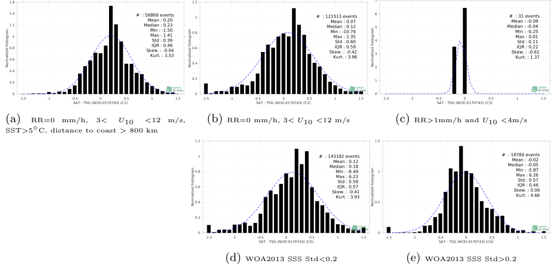
Figure 13: Normalized histogram of \Delta SSS (SMAP SSS L3 v5.0 - 8-Day running (JPL) - TSG (NCEI-0170743)) for 5 different subdatasets corresponding to: RR=0 mm/h, 3 < U_{10} < 12 m/s, SST>5°C, distance to coast > 800 km (a), RR=0 mm/h, 3 < U_{10} < 12 m/s (b), RR>1mm/h and U_{10} < 4 m/s (c), WOA2013 SSS Std<0.2 (d), WOA2013 SSS Std>0.2 (e).
