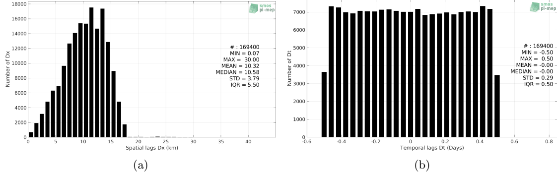
Figure 5: Histograms of the spatial (a) and temporal (b) lags between the location/time of the TSG (NCEI-0170743) measurement and the date of the corresponding SMAP SSS L3 v5.0 - 8-Day running (JPL) SSS pixel.
