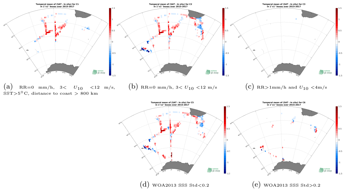
Figure 12: Temporal mean gridded over spatial boxes of size 1^\circ \times 1^\circ of \Delta\text{SSS} (SMAP SSS L3 v5.0 - 8-Day running (JPL) - TSG (NCEI-0170743)) for 5 different subdatasets corresponding to:RR=0 mm/h, 3 < U_{10} < 12 m/s, SST >5^\circ\text{C} , distance to coast > 800 km (a), RR=0 mm/h, 3 < U_{10} < 12 m/s (b), RR >1 mm/h and U_{10} < 4 m/s (c), WOA2013 SSS Std <0.2 (d), WOA2013 SSS Std >0.2 (e).
