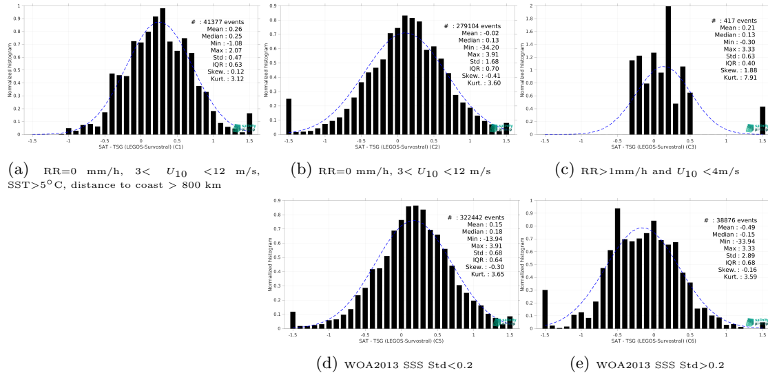
Figure 15: Normalized histogram of \Delta SSS (SMAP SSS L3 v5.0 - 8-Day running (JPL) - TSG (LEGOs-Survostral)) for 5 different subdatasets corresponding to: RR=0 mm/h, 3 < U_{10} < 12 m/s, SST > 5°C, distance to coast > 800 km (a), RR=0 mm/h, 3 < U_{10} < 12 m/s (b), RR > 1mm/h and U_{10} < 4 m/s (c), WOA2013 SSS Std < 0.2 (d), WOA2013 SSS Std > 0.2 (e).
