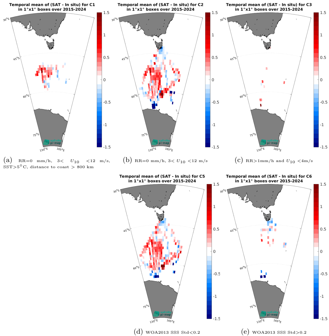
Figure 14: Temporal mean gridded over spatial boxes of size 1^\circ \times 1^\circ of \Delta SSS (SMAP SSS L3 v5.0 - 8-Day running (JPL) - TSG (LEGOS-Survostral)) for 5 different subdatasets corresponding to:RR=0 mm/h, 3 < U_{10} < 12 m/s, SST>5°C, distance to coast > 800 km (a), RR=0 mm/h, 3 < U_{10} < 12 m/s (b), RR>1mm/h and U_{10} < 4 m/s (c), WOA2013 SSS Std<0.2 (d), WOA2013 SSS Std>0.2 (e).
