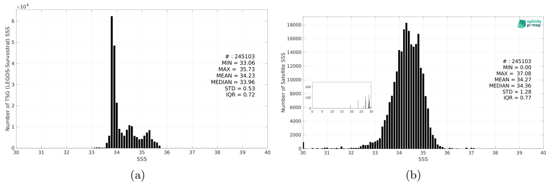
Figure 3: Histograms of SSS from TSG (LEGOS-Survostral) (a) and SMAP SSS L3 v5.0 - 8-Day running (JPL) (b) considering all match-up pairs per bins of 0.1 over the Global Ocean Pi-MEP region and for the full satellite product period.
