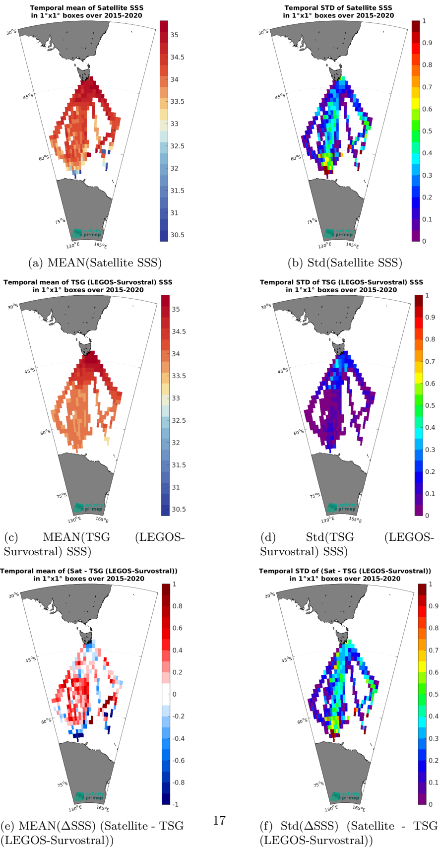
Figure 7: Temporal mean (left) and Std (right) of SSS from SMAP SSS L3 v5.0 - 8-Day running (JPL) (top), TSG (LEGOS-Survostral) (middle), and of \Delta SSS (Satellite - TSG (LEGOS-Survostral)). Only match-up pairs are used to generate these maps.
