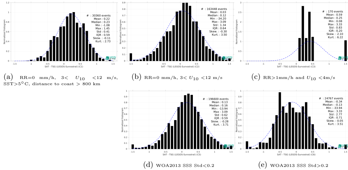
Figure 15: Normalized histogram of \Delta SSS (SMAP SSS L3 v5.0 - 8-Day running (JPL) - TSG (LEGOS-Survostral)) for 5 different subdatasets corresponding to: RR=0 mm/h, 3 < U_{10} < 12 m/s, SST>5°C, distance to coast > 800 km (a), RR=0 mm/h, 3 < U_{10} < 12 m/s (b), RR>1mm/h and U_{10} < 4 m/s (c), WOA2013 SSS Std<0.2 (d), WOA2013 SSS Std>0.2 (e).
