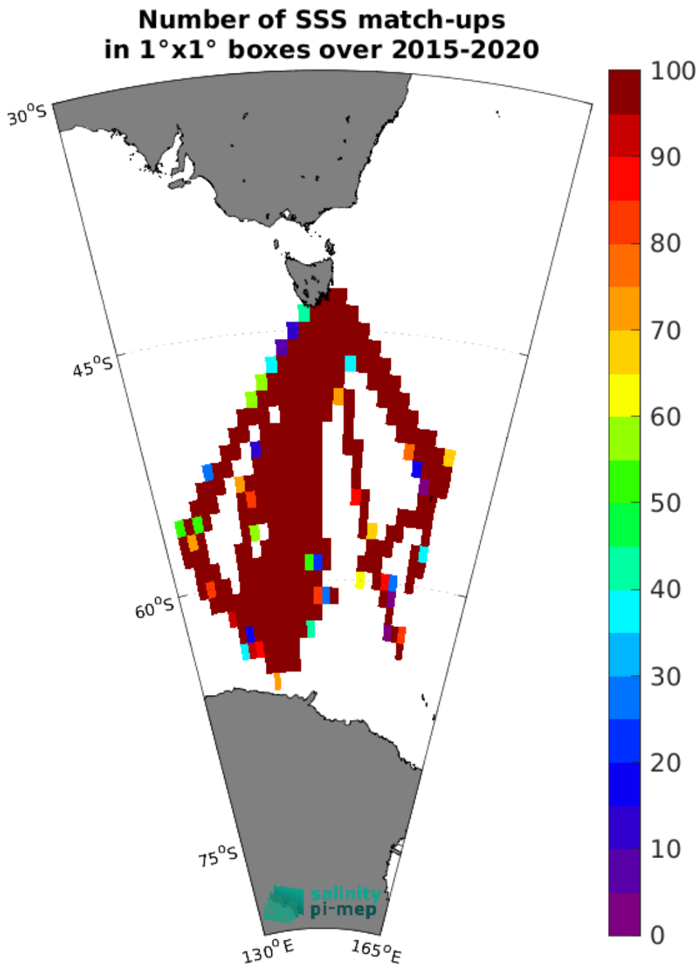
Figure 5: Number of SSS match-ups between TSG (LEGOS-Survostral) SSS and the SMAP SSS L3 v5.0 - 8-Day running (JPL) SSS product for the Global Ocean Pi-MEP region over 1°x1° boxes and for the full satellite product period.
