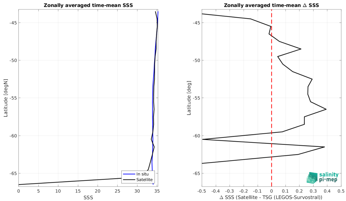
Figure 9: Left panel: Zonal mean SSS from SMAP SSS L3 v5.0 - 8-Day running (JPL) satellite product (black) and from TSG (LEGOS-Survostral) (blue). Right panel: Zonal mean of \Delta SSS (Satellite - TSG (LEGOS-Survostral)) for all the collected Pi-MEP match-up pairs estimated over the full satellite product period.
