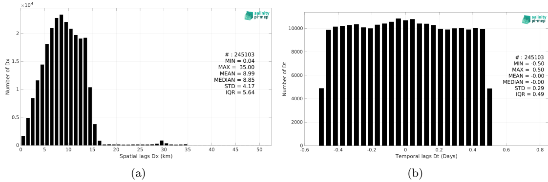
Figure 6: Histograms of the spatial (a) and temporal (b) lags between the location/time of the TSG (LEGOS-Survostral) measurement and the date of the corresponding SMAP SSS L3 v5.0 - 8-Day running (JPL) SSS pixel.
