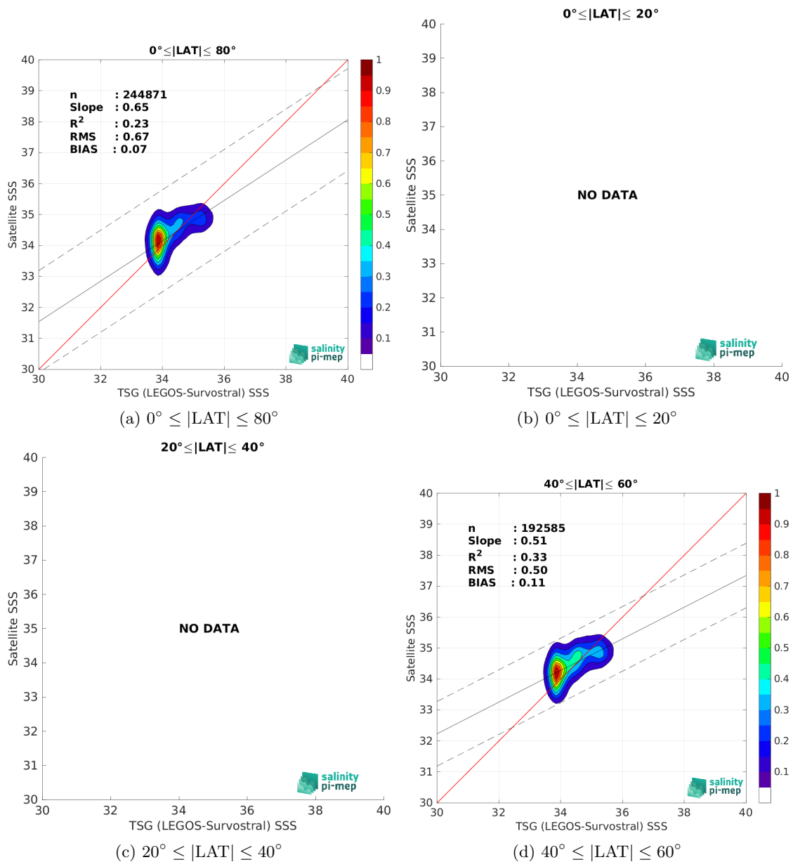
Figure 10: Contour maps of the concentration of SMAP SSS L3 v5.0 - 8-Day running (JPL) SSS (y-axis) versus TSG (LEGOS-Survostral) SSS (x-axis) at match-up pairs for different latitude bands. For each plot, the red line shows x=y . The black thin and dashed lines indicate a linear fit through the data cloud and the \pm 95\% confidence levels, respectively. The number match-up pairs n , the slope and R^2 coefficient of the linear fit, the root mean square (RMS) and the mean bias between satellite and in situ data are indicated for each latitude band in each plots.
