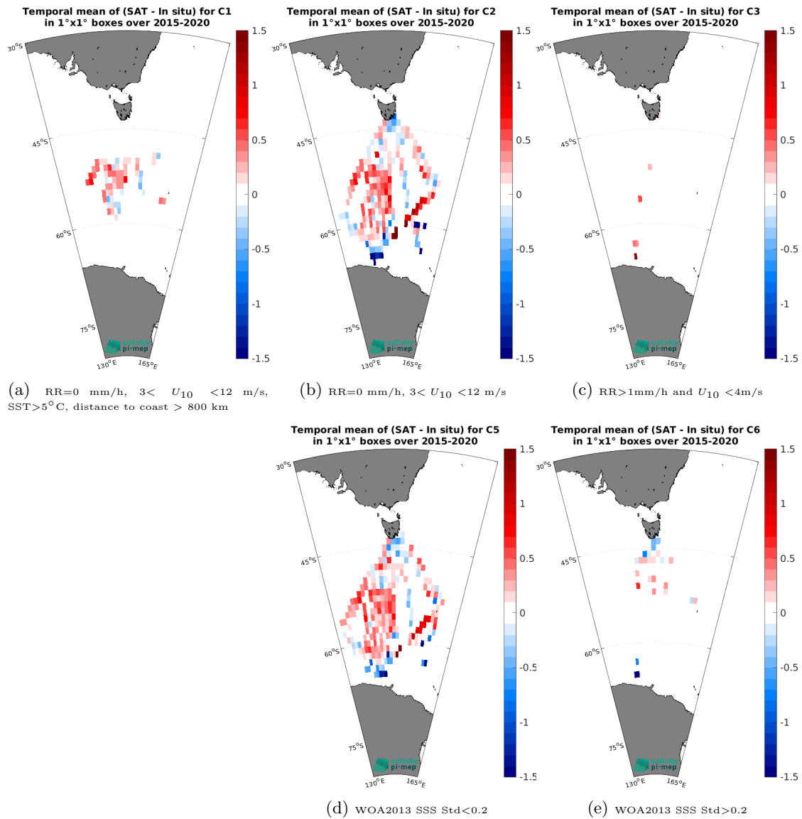
Figure 14: Temporal mean gridded over spatial boxes of size 1^\circ \times 1^\circ of \Delta\text{SSS} (SMAP SSS L3 v5.0 - 8-Day running (JPL) - TSG (LEGOS-Survostral)) for 5 different subdatasets corresponding to: RR=0 mm/h, 3 < U_{10} < 12 m/s, SST > 5^\circ\text{C} , distance to coast > 800 km (a), RR=0 mm/h, 3 < U_{10} < 12 m/s (b), RR > 1 mm/h and U_{10} < 4 m/s (c), WOA2013 SSS Std < 0.2 (d), WOA2013 SSS Std > 0.2 (e).
