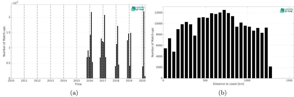
Figure 2: Number of match-ups between TSG (LEGOS-Survostral) and SMAP SSS L3 v5.0 - 8-Day running (JPL) SSS as a function of time (a) and as function of the distance to coast (b) over the Global Ocean Pi-MEP region and for the full satellite product period.
