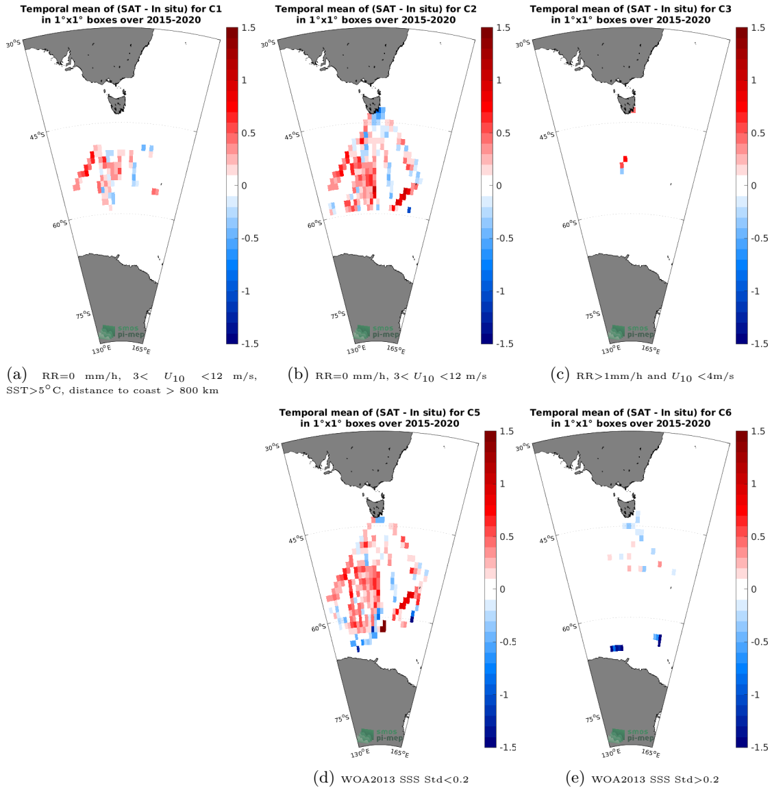
Figure 12: Temporal mean gridded over spatial boxes of size 1^\circ \times 1^\circ of \Delta SSS (SMAP SSS L3 v5.0 - 8-Day running (JPL) - TSG (LEGOS-Survostral)) for 5 different subdatasets corresponding to:RR=0 mm/h, 3 < U_{10} < 12 m/s, SST>5°C, distance to coast > 800 km (a), RR=0 mm/h, 3 < U_{10} < 12 m/s (b), RR>1mm/h and U_{10} < 4 m/s (c), WOA2013 SSS Std<0.2 (d), WOA2013 SSS Std>0.2 (e).
