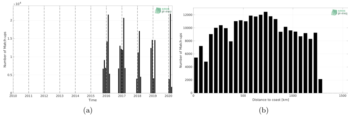
Figure 1: Number of match-ups between TSG (LEGOS-Survostral) and SMAP SSS L3 v5.0 - 8-Day running (JPL) SSS as a function of time (a) and as function of the distance to coast (b) over the Global Ocean Pi-MEP region and for the full satellite product period.
