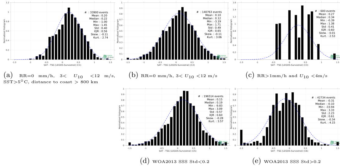
Figure 13: Normalized histogram of \Delta SSS (SMAP SSS L3 v5.0 - 8-Day running (JPL) - TSG (LEGOS-Survostral)) for 5 different subdatasets corresponding to: RR=0 mm/h, 3 < U_{10} < 12 m/s, SST > 5°C, distance to coast > 800 km (a), RR=0 mm/h, 3 < U_{10} < 12 m/s (b), RR > 1mm/h and U_{10} < 4 m/s (c), WOA2013 SSS Std < 0.2 (d), WOA2013 SSS Std > 0.2 (e).
