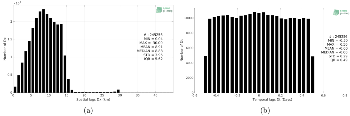
Figure 5: Histograms of the spatial (a) and temporal (b) lags between the location/time of the TSG (LEGOS-Survostral) measurement and the date of the corresponding SMAP SSS L3 v5.0 - 8-Day running (JPL) SSS pixel.
