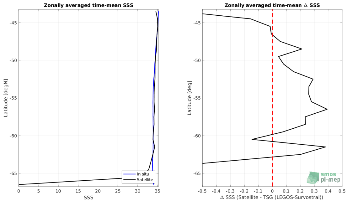
Figure 8: Left panel: Zonal mean SSS from SMAP SSS L3 v5.0 - 8-Day running (JPL) satellite product (black) and from TSG (LEGOS-Survostral) (blue). Right panel: Zonal mean of \Delta SSS (Satellite - TSG (LEGOS-Survostral)) for all the collected Pi-MEP match-up pairs estimated over the full satellite product period.
