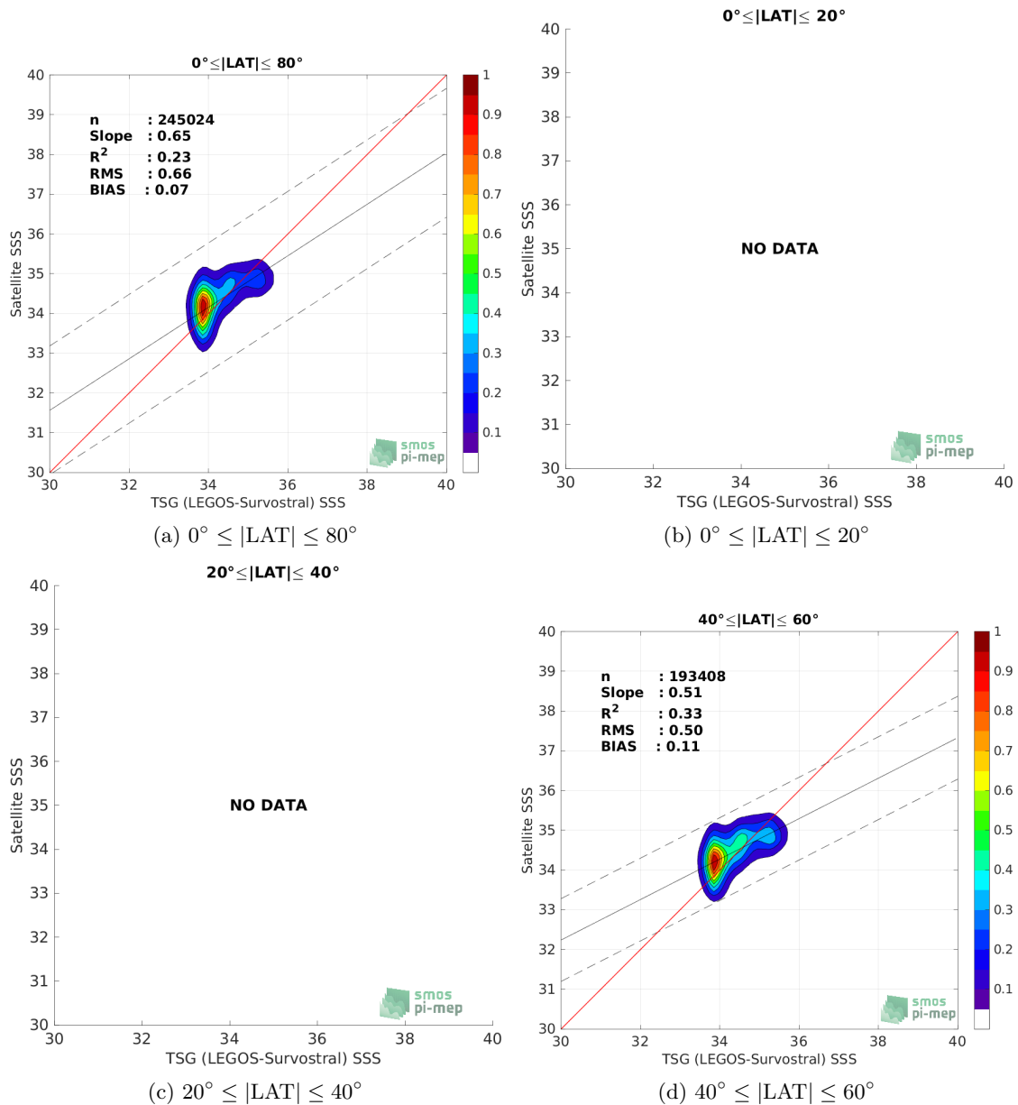
Figure 9: Contour maps of the concentration of SMAP SSS L3 v5.0 - 8-Day running (JPL) SSS (y-axis) versus TSG (LEGOS-Survostral) SSS (x-axis) at match-up pairs for different latitude bands. For each plot, the red line shows x=y . The black thin and dashed lines indicate a linear fit through the data cloud and the \pm 95\% confidence levels, respectively. The number match-up pairs n , the slope and R^2 coefficient of the linear fit, the root mean square (RMS) and the mean bias between satellite and in situ data are indicated for each latitude band in each plots.
