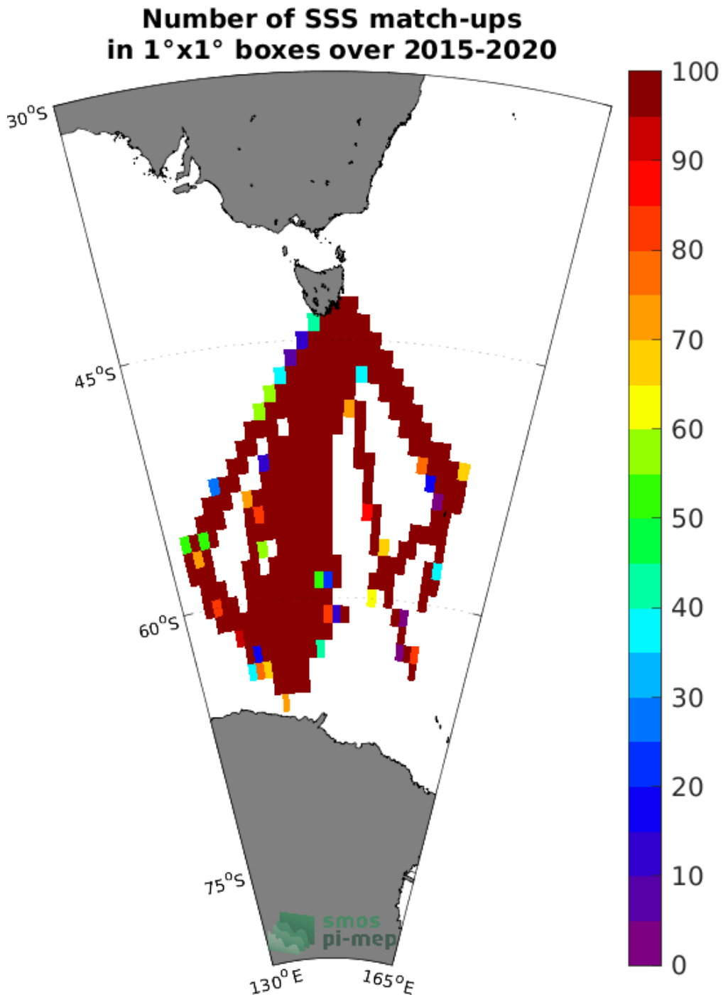
Figure 4: Number of SSS match-ups between TSG (LEGOS-Survostral) SSS and the SMAP SSS L3 v5.0 - 8-Day running (JPL) SSS product for the Global Ocean Pi-MEP region over 1°x1° boxes and for the full satellite product period.
