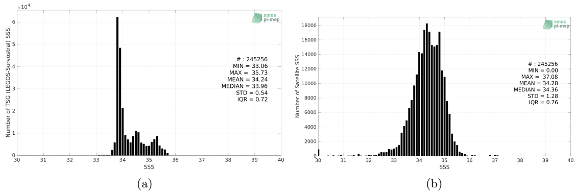
Figure 2: Histograms of SSS from TSG (LEGOS-Survostral) (a) and SMAP SSS L3 v5.0 - 8-Day running (JPL) (b) considering all match-up pairs per bins of 0.1 over the Global Ocean Pi-MEP region and for the full satellite product period.
