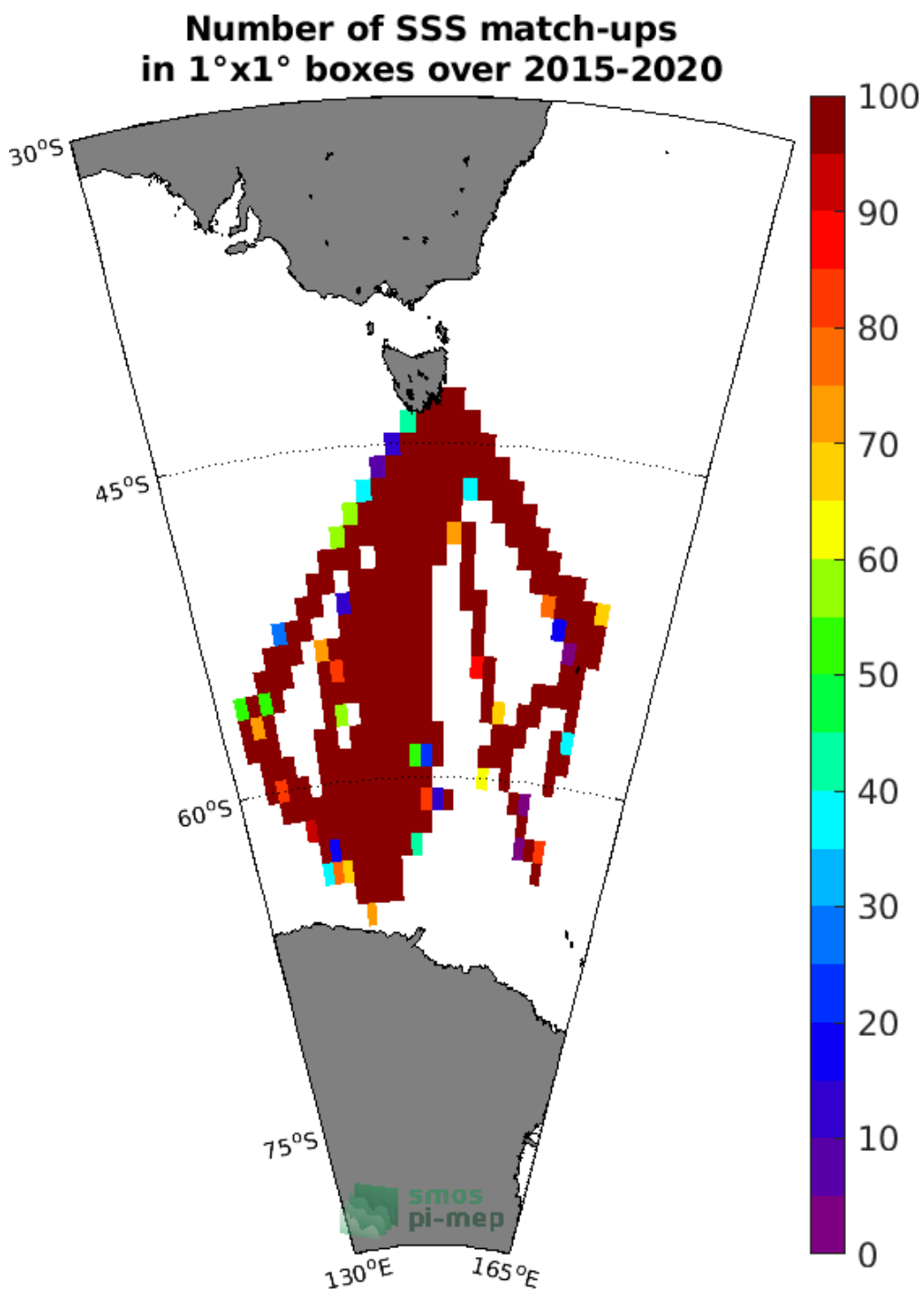
Figure 4: Number of SSS match-ups between TSG (LEGOS-Survostral) SSS and the SMAP SSS L3 v5.0 - 8-Day running (JPL) SSS product for the Global Ocean Pi-MEP region over 1°x1° boxes and for the full satellite product period.
