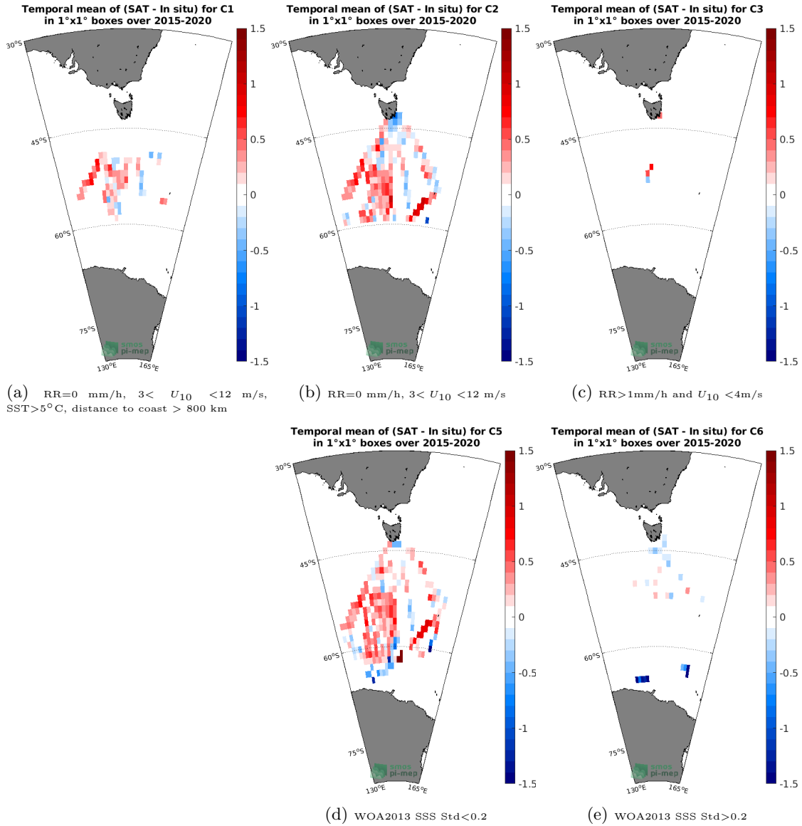
Figure 12: Temporal mean gridded over spatial boxes of size 1^\circ \times 1^\circ of \Delta SSS (SMAP SSS L3 v5.0 - 8-Day running (JPL) - TSG (LEGOS-Survostral)) for 5 different subdatasets corresponding to: RR=0 mm/h, 3 < U_{10} < 12 m/s, SST>5°C, distance to coast > 800 km (a), RR=0 mm/h, 3 < U_{10} < 12 m/s (b), RR>1mm/h and U_{10} < 4 m/s (c), WOA2013 SSS Std<0.2 (d), WOA2013 SSS Std>0.2 (e).
