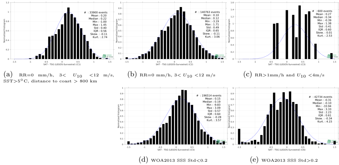
Figure 13: Normalized histogram of \Delta SSS (SMAP SSS L3 v5.0 - 8-Day running (JPL) - TSG (LEGOS-Survostral)) for 5 different subdatasets corresponding to: RR=0 mm/h, 3 < U_{10} < 12 m/s, SST>5°C, distance to coast > 800 km (a), RR=0 mm/h, 3 < U_{10} < 12 m/s, SST>5°C, distance to coast > 800 km (a), RR=0 mm/h, 3 < U_{10} < 12 m/s (b), RR>1mm/h and U_{10} < 4 m/s (c), WOA2013 SSS Std<0.2 (d), WOA2013 SSS Std>0.2 (e).
