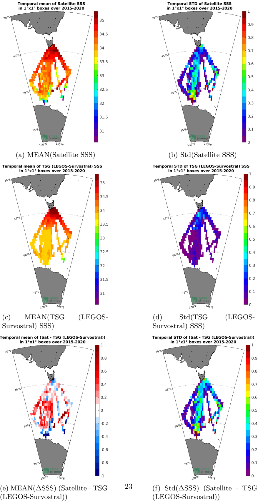
Figure 6: Temporal mean (left) and Std (right) of SSS from SMAP SSS L3 v5.0 - 8-Day running (JPL) (top), TSG (LEGOS-Survostral) (middle), and of \Delta SSS (Satellite - TSG (LEGOS-Survostral)). Only match-up pairs are used to generate these maps.
