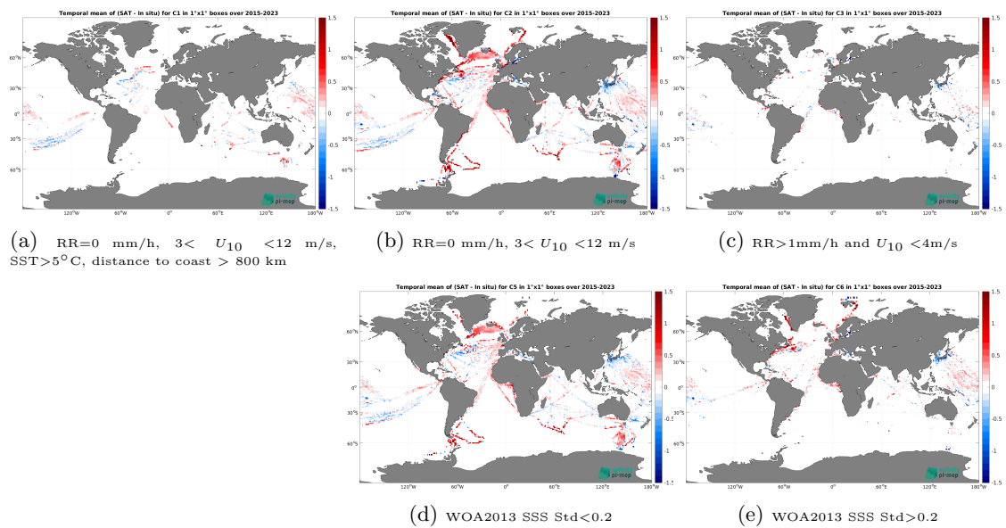
Figure 14: Temporal mean gridded over spatial boxes of size 1^\circ \times 1^\circ of \Delta SSS (SMAP SSS L3 v5.0 - 8-Day running (JPL) - TSG (LEGOS-DM)) for 5 different subdatasets corresponding to:RR=0 mm/h, 3 < U_{10} < 12 m/s, SST >5^\circ C, distance to coast > 800 km (a), RR=0 mm/h, 3 < U_{10} < 12 m/s (b), RR >1 mm/h and U_{10} < 4 m/s (c), WOA2013 SSS Std <0.2 (d), WOA2013 SSS Std >0.2 (e).
