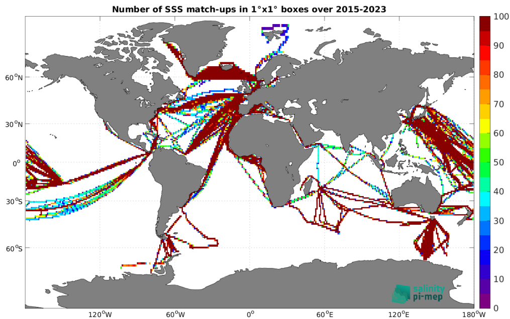
Figure 5: Number of SSS match-ups between TSG (LEGOS-DM) SSS and the SMAP SSS L3 v5.0 - 8-Day running (JPL) SSS product for the Global Ocean Pi-MEP region over 1^\circ \times 1^\circ boxes and for the full satellite product period.
