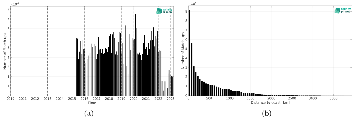
Figure 2: Number of match-ups between TSG (LEGOS-DM) and SMAP SSS L3 v5.0 - 8-Day running (JPL) SSS as a function of time (a) and as function of the distance to coast (b) over the Global Ocean Pi-MEP region and for the full satellite product period.
