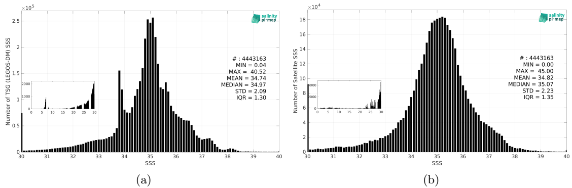
Figure 3: Histograms of SSS from TSG (LEGOS-DM) (a) and SMAP SSS L3 v5.0 - 8-Day running (JPL) (b) considering all match-up pairs per bins of 0.1 over the Global Ocean Pi-MEP region and for the full satellite product period.
