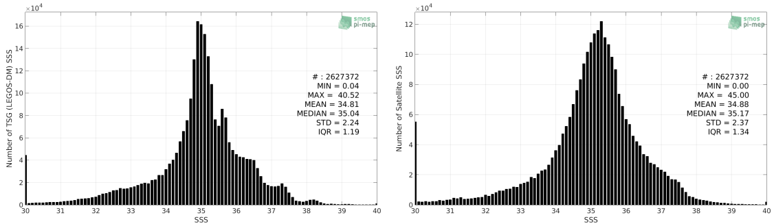
Figure 2: Histograms of SSS from TSG (LEGOS-DM) (a) and SMAP SSS L3 v5.0 - 8-Day running (JPL) (b) considering all match-up pairs per bins of 0.1 over the Global Ocean Pi-MEP region and for the full satellite product period.
