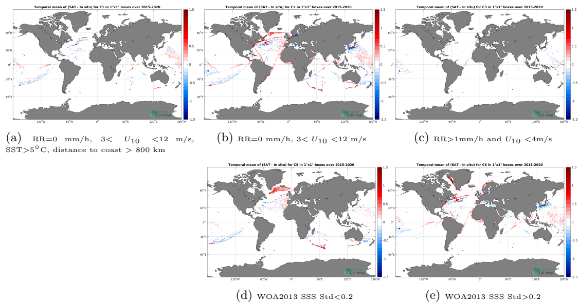
Figure 12: Temporal mean gridded over spatial boxes of size 1^\circ \times 1^\circ of \Delta\text{SSS} (SMAP SSS L3 v5.0 - 8-Day running (JPL) - TSG (LEGOS-DM)) for 5 different subdatasets corresponding to:RR=0 mm/h, 3 < U_{10} < 12 m/s, SST >5^\circ\text{C} , distance to coast > 800 km (a), RR=0 mm/h, 3 < U_{10} < 12 m/s (b), RR >1 mm/h and U_{10} < 4 m/s (c), WOA2013 SSS Std <0.2 (d), WOA2013 SSS Std >0.2 (e).
