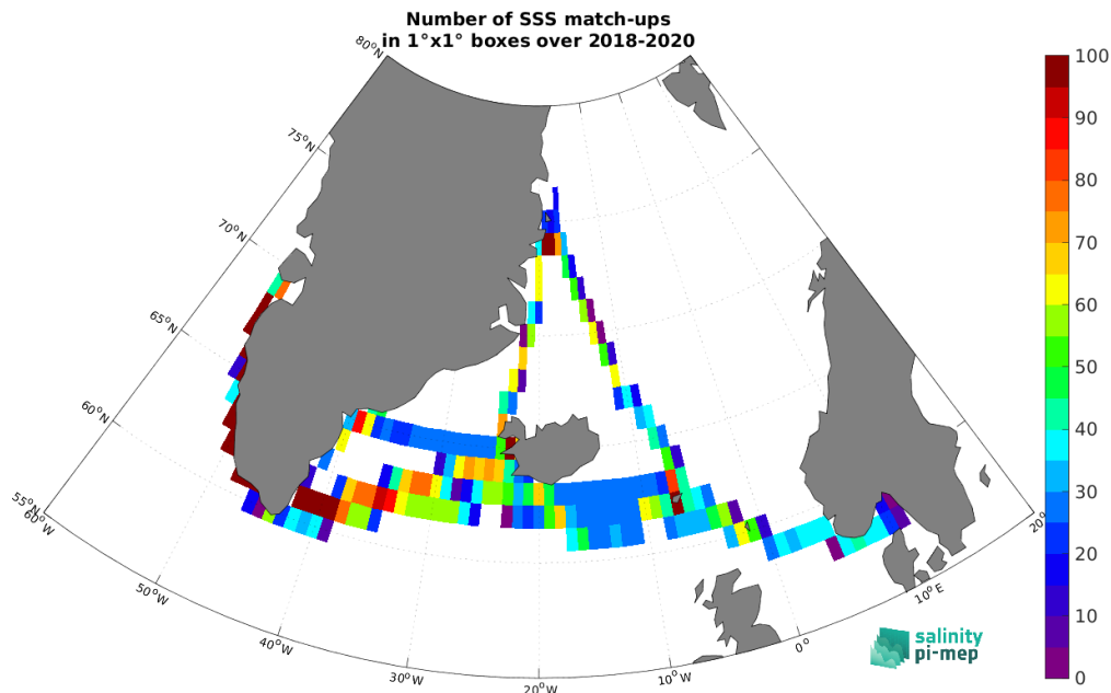
Figure 5: Number of SSS match-ups between TSG (Lauge-Koch) SSS and the SMAP SSS L3 v5.0 - 8-Day running (JPL) SSS product for the Global Ocean Pi-MEP region over 1^\circ \times 1^\circ boxes and for the full satellite product period.
