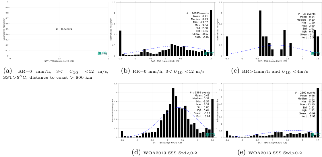
Figure 15: Normalized histogram of \Delta SSS (SMAP SSS L3 v5.0 - 8-Day running (JPL) - TSG (Lauge-Koch)) for 5 different subdatasets corresponding to: RR=0 mm/h, 3 < U_{10} < 12 m/s, SST > 5°C, distance to coast > 800 km (a), RR=0 mm/h, 3 < U_{10} < 12 m/s (b), RR > 1mm/h and U_{10} < 4 m/s (c), WOA2013 SSS Std < 0.2 (d), WOA2013 SSS Std > 0.2 (e).
