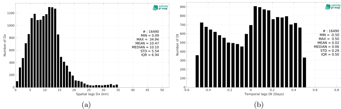
Figure 6: Histograms of the spatial (a) and temporal (b) lags between the location/time of the TSG (Lauge-Koch) measurement and the date of the corresponding SMAP SSS L3 v5.0 - 8-Day running (JPL) SSS pixel.
