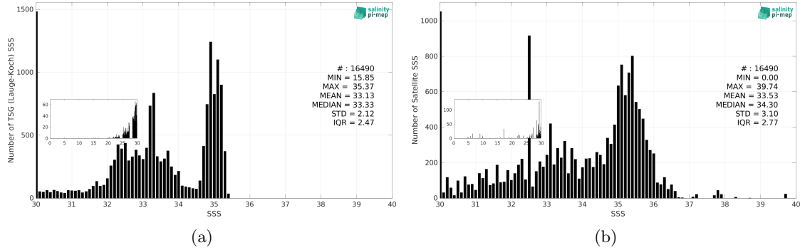
Figure 3: Histograms of SSS from TSG (Lauge-Koch) (a) and SMAP SSS L3 v5.0 - 8-Day running (JPL) (b) considering all match-up pairs per bins of 0.1 over the Global Ocean Pi-MEP region and for the full satellite product period.
