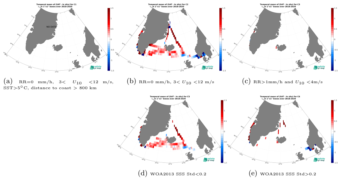
Figure 14: Temporal mean gridded over spatial boxes of size 1^\circ \times 1^\circ of \Delta SSS (SMAP SSS L3 v5.0 - 8-Day running (JPL) - TSG (Lauge-Koch)) for 5 different subdatasets corresponding to:RR=0 mm/h, 3 < U_{10} < 12 m/s, SST >5^\circ C, distance to coast > 800 km (a), RR=0 mm/h, 3 < U_{10} < 12 m/s (b), RR >1 mm/h and U_{10} < 4 m/s (c), WOA2013 SSS Std <0.2 (d), WOA2013 SSS Std >0.2 (e).
