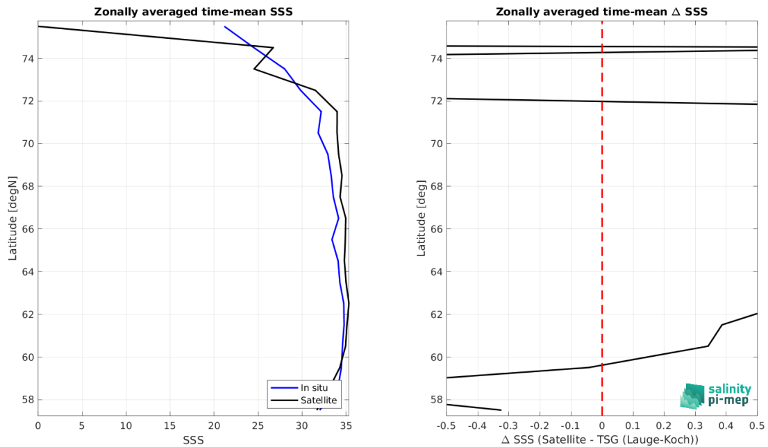
Figure 9: Left panel: Zonal mean SSS from SMAP SSS L3 v5.0 - 8-Day running (JPL) satellite product (black) and from TSG (Lauge-Koch) (blue). Right panel: Zonal mean of \Delta SSS (Satellite - TSG (Lauge-Koch)) for all the collected Pi-MEP match-up pairs estimated over the full satellite product period.
