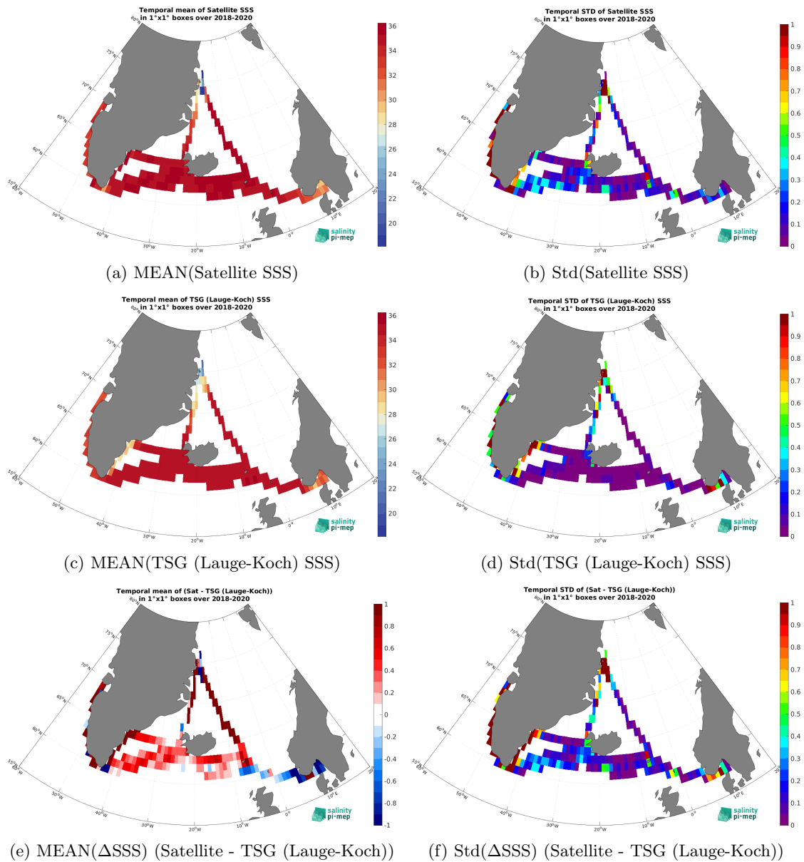
Figure 7: Temporal mean (left) and Std (right) of SSS from SMAP SSS L3 v5.0 - 8-Day running (JPL) (top), TSG (Lauge-Koch) (middle), and of \Delta SSS (Satellite - TSG (Lauge-Koch)). Only match-up pairs are used to generate these maps.
