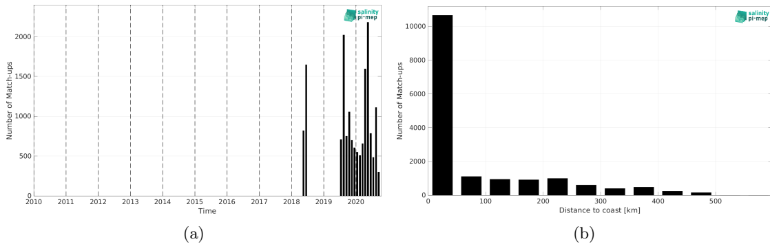
Figure 2: Number of match-ups between TSG (Lauge-Koch) and SMAP SSS L3 v5.0 - 8-Day running (JPL) SSS as a function of time (a) and as function of the distance to coast (b) over the Global Ocean Pi-MEP region and for the full satellite product period.
