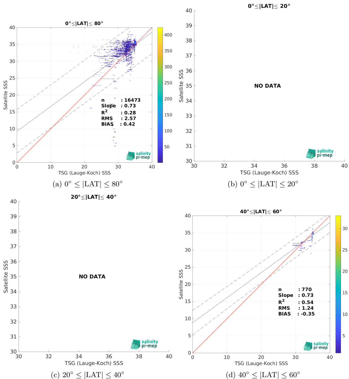
Figure 10: Contour maps of the concentration of SMAP SSS L3 v5.0 - 8-Day running (JPL) SSS (y-axis) versus TSG (Lauge-Koch) SSS (x-axis) at match-up pairs for different latitude bands. For each plot, the red line shows x=y . The black thin and dashed lines indicate a linear fit through the data cloud and the \pm 95\% confidence levels, respectively. The number match-up pairs n , the slope and R^2 coefficient of the linear fit, the root mean square (RMS) and the mean bias between satellite and in situ data are indicated for each latitude band in each plots.
