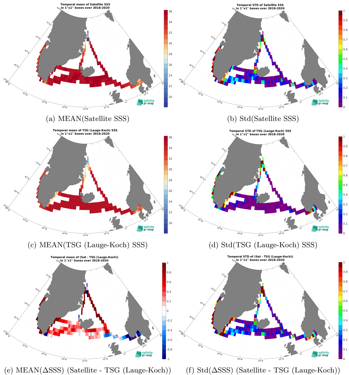
Figure 6: Temporal mean (left) and Std (right) of SSS from SMAP SSS L3 v5.0 - 8-Day running (JPL) (top), TSG (Lauge-Koch) (middle), and of \Delta SSS (Satellite - TSG (Lauge-Koch)). Only match-up pairs are used to generate these maps.
