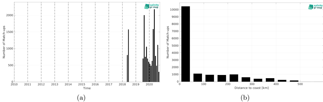
Figure 1: Number of match-ups between TSG (Lauge-Koch) and SMAP SSS L3 v5.0 - 8-Day running (JPL) SSS as a function of time (a) and as function of the distance to coast (b) over the Global Ocean Pi-MEP region and for the full satellite product period.
