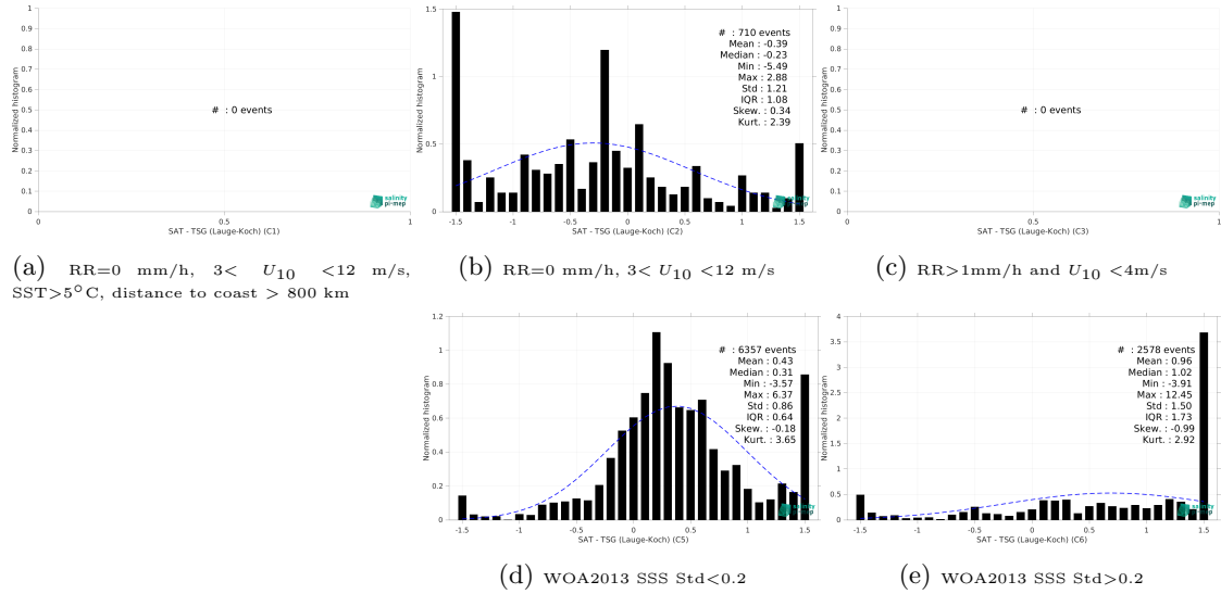
Figure 13: Normalized histogram of \Delta SSS (SMAP SSS L3 v5.0 - 8-Day running (JPL) - TSG (Lauge-Koch)) for 5 different subdatasets corresponding to: RR=0 mm/h, 3 < U_{10} < 12 m/s, SST > 5°C, distance to coast > 800 km (a), RR=0 mm/h, 3 < U_{10} < 12 m/s (b), RR > 1mm/h and U_{10} < 4 m/s (c), WOA2013 SSS Std < 0.2 (d), WOA2013 SSS Std > 0.2 (e).
