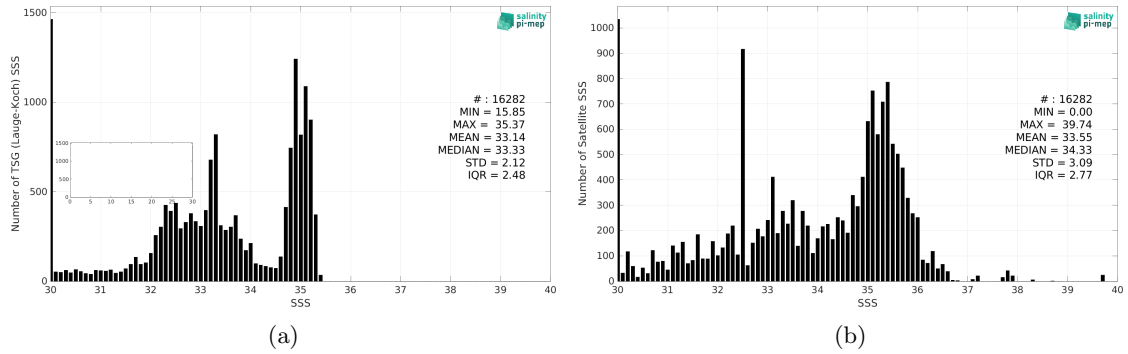
Figure 2: Histograms of SSS from TSG (Lauge-Koch) (a) and SMAP SSS L3 v5.0 - 8-Day running (JPL) (b) considering all match-up pairs per bins of 0.1 over the Global Ocean Pi-MEP region and for the full satellite product period.
