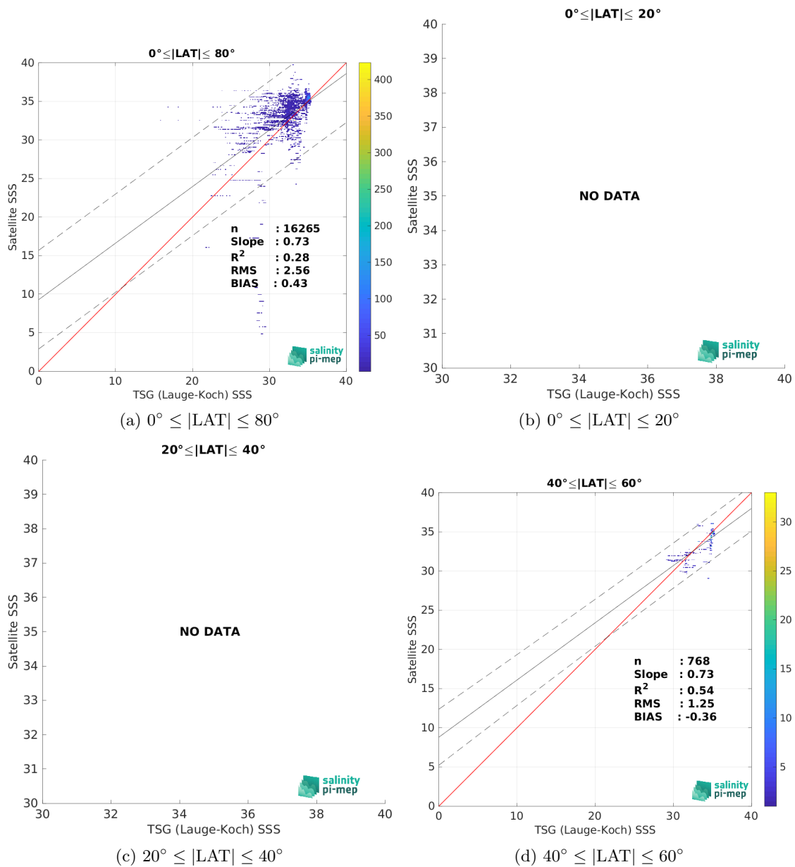
Figure 9: Contour maps of the concentration of SMAP SSS L3 v5.0 - 8-Day running (JPL) SSS (y-axis) versus TSG (Lauge-Koch) SSS (x-axis) at match-up pairs for different latitude bands. For each plot, the red line shows x=y . The black thin and dashed lines indicate a linear fit through the data cloud and the \pm 95\% confidence levels, respectively. The number match-up pairs n , the slope and R^2 coefficient of the linear fit, the root mean square (RMS) and the mean bias between satellite and in situ data are indicated for each latitude band in each plots.
