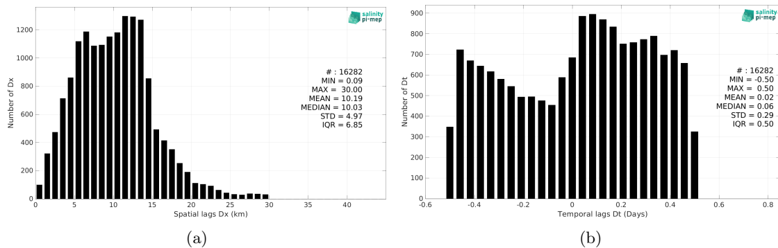
Figure 5: Histograms of the spatial (a) and temporal (b) lags between the location/time of the TSG (Lauge-Koch) measurement and the date of the corresponding SMAP SSS L3 v5.0 - 8-Day running (JPL) SSS pixel.
