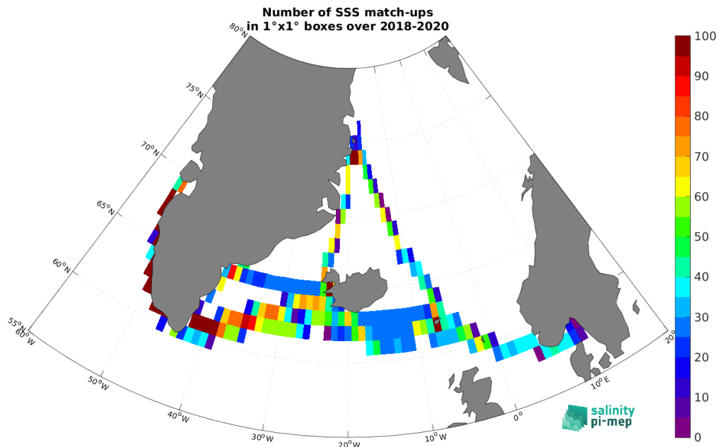
Figure 4: Number of SSS match-ups between TSG (Lauge-Koch) SSS and the SMAP SSS L3 v5.0 - 8-Day running (JPL) SSS product for the Global Ocean Pi-MEP region over 1^\circ \times 1^\circ boxes and for the full satellite product period.
