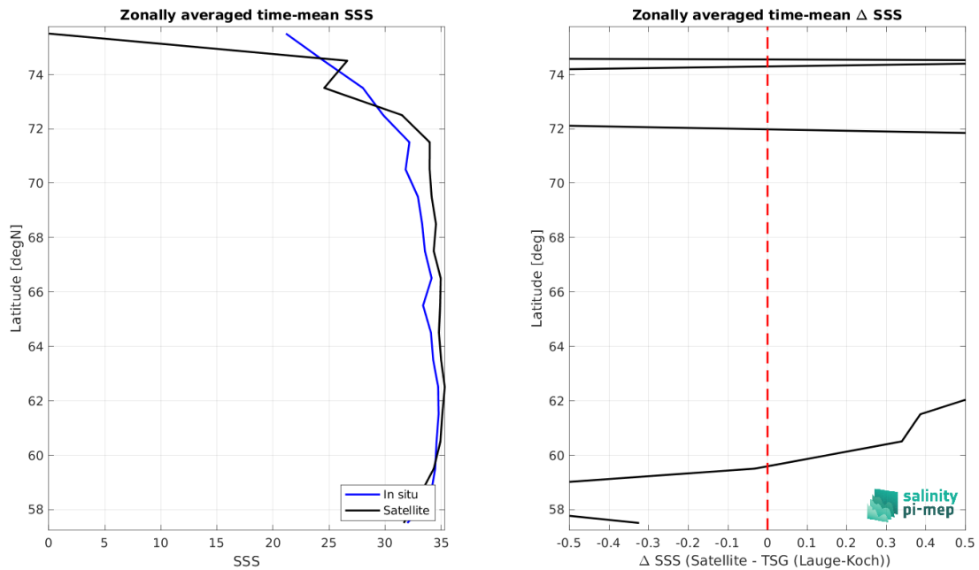
Figure 8: Left panel: Zonal mean SSS from SMAP SSS L3 v5.0 - 8-Day running (JPL) satellite product (black) and from TSG (Lauge-Koch) (blue). Right panel: Zonal mean of \Delta SSS (Satellite - TSG (Lauge-Koch)) for all the collected Pi-MEP match-up pairs estimated over the full satellite product period.
