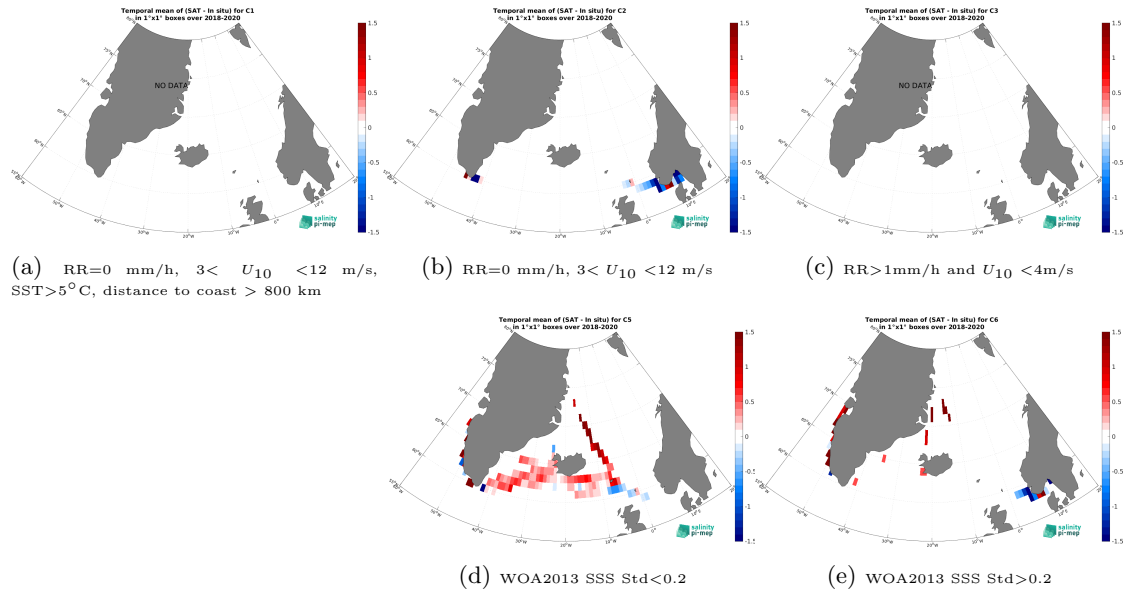
Figure 12: Temporal mean gridded over spatial boxes of size 1^{\circ}\times 1^{\circ} of \Delta\text{SSS} (SMAP SSS L3 v5.0 - 8-Day running (JPL) - TSG (Lauge-Koch)) for 5 different subdatasets corresponding to:RR=0 mm/h, 3 < U_{10} < 12 m/s, SST > 5^{\circ}\text{C} , distance to coast > 800 km (a), RR=0 mm/h, 3 < U_{10} < 12 m/s (b), RR > 1 mm/h and U_{10} < 4 m/s (c), WOA2013 SSS Std < 0.2 (d), WOA2013 SSS Std > 0.2 (e).
