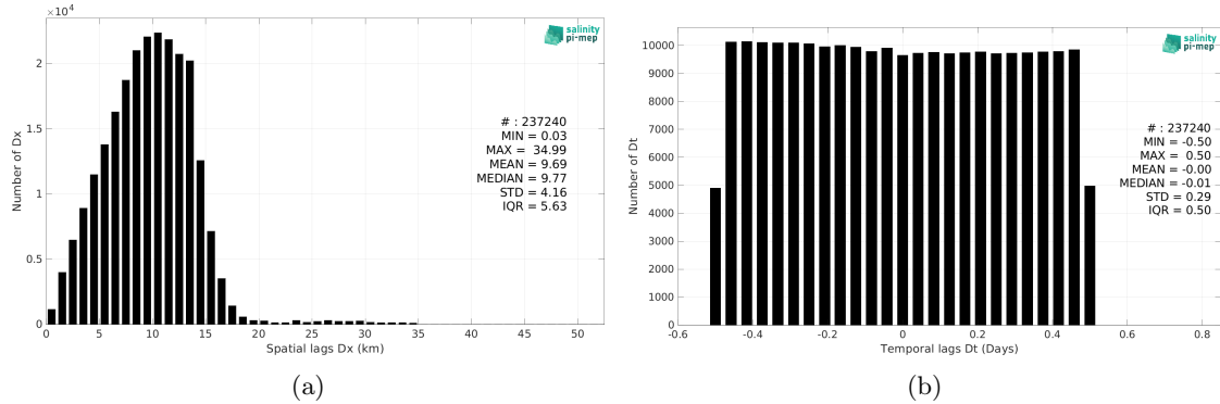
Figure 6: Histograms of the spatial (a) and temporal (b) lags between the location/time of the TSG (GOSUD-Sailing-ship) measurement and the date of the corresponding SMAP SSS L3 v5.0 - 8-Day running (JPL) SSS pixel.
