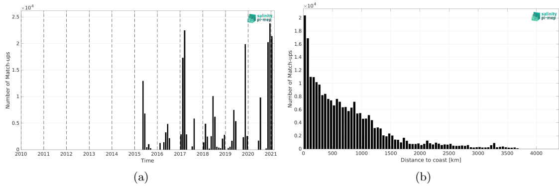
Figure 2: Number of match-ups between TSG (GOSUD-Sailing-ship) and SMAP SSS L3 v5.0 - 8-Day running (JPL) SSS as a function of time (a) and as function of the distance to coast (b) over the Global Ocean Pi-MEP region and for the full satellite product period.
