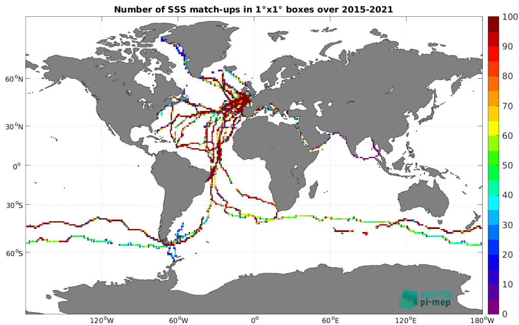
Figure 5: Number of SSS match-ups between TSG (GOSUD-Sailing-ship) SSS and the SMAP SSS L3 v5.0 - 8-Day running (JPL) SSS product for the Global Ocean Pi-MEP region over 1^\circ \times 1^\circ boxes and for the full satellite product period.
