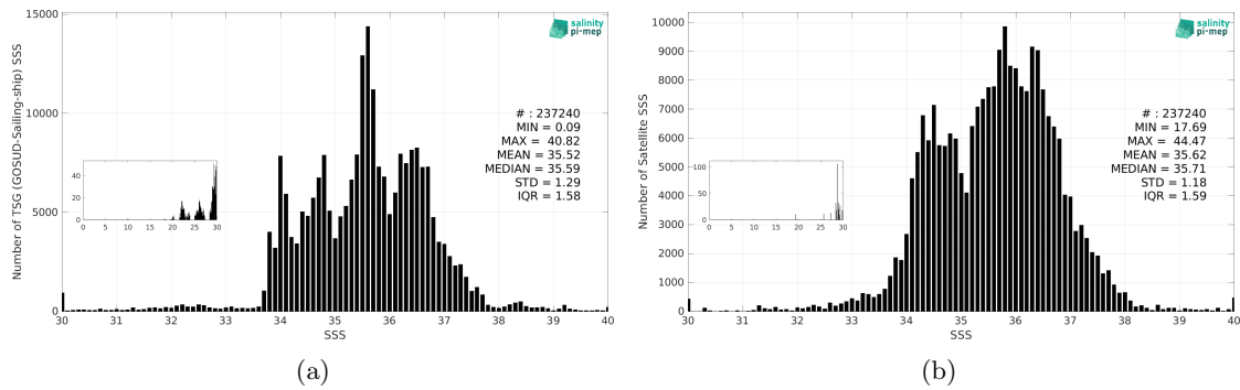
Figure 3: Histograms of SSS from TSG (GOSUD-Sailing-ship) (a) and SMAP SSS L3 v5.0 - 8-Day running (JPL) (b) considering all match-up pairs per bins of 0.1 over the Global Ocean Pi-MEP region and for the full satellite product period.
