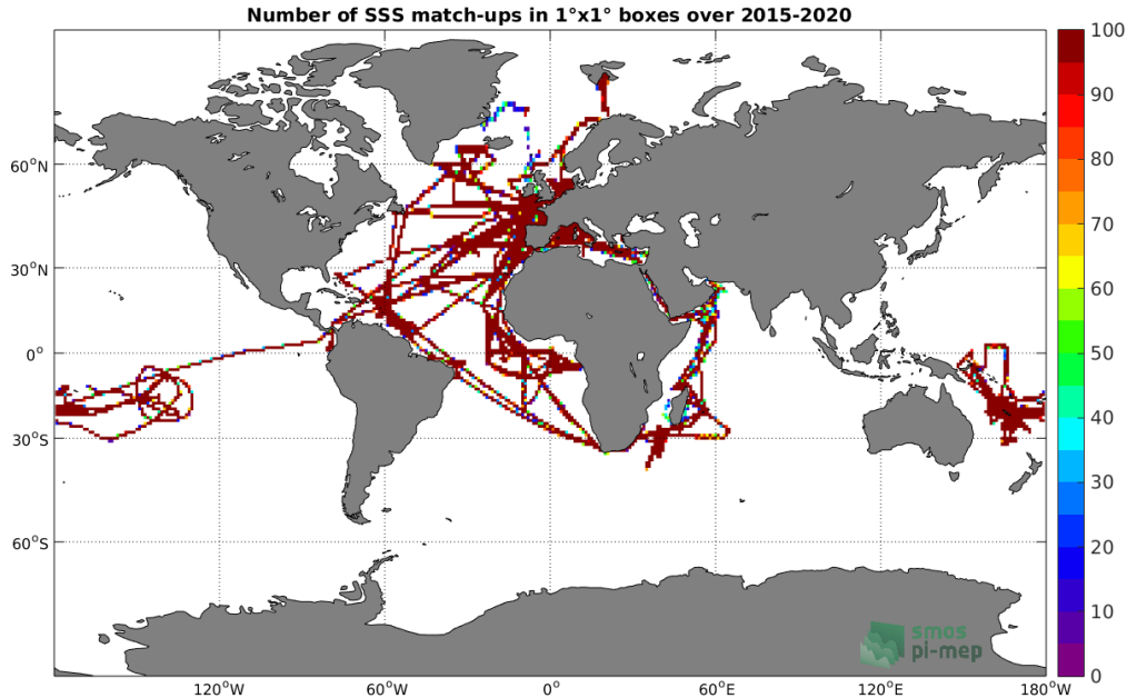
Figure 4: Number of SSS match-ups between TSG (GOSUD-Research-vessel) SSS and the SMAP SSS L3 v5.0 - 8-Day running (JPL) SSS product for the Global Ocean Pi-MEP region over 1^\circ \times 1^\circ boxes and for the full satellite product period.
