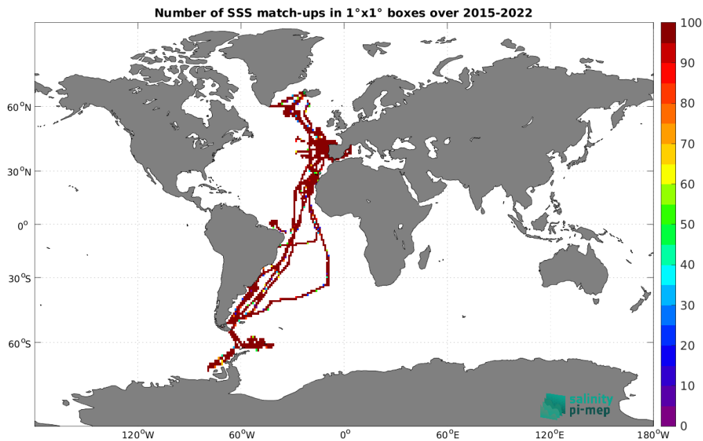
Figure 5: Number of SSS match-ups between TSG (CSIC-UTM) SSS and the SMAP SSS L3 v5.0 - 8-Day running (JPL) SSS product for the Global Ocean Pi-MEP region over 1^\circ \times 1^\circ boxes and for the full satellite product period.
