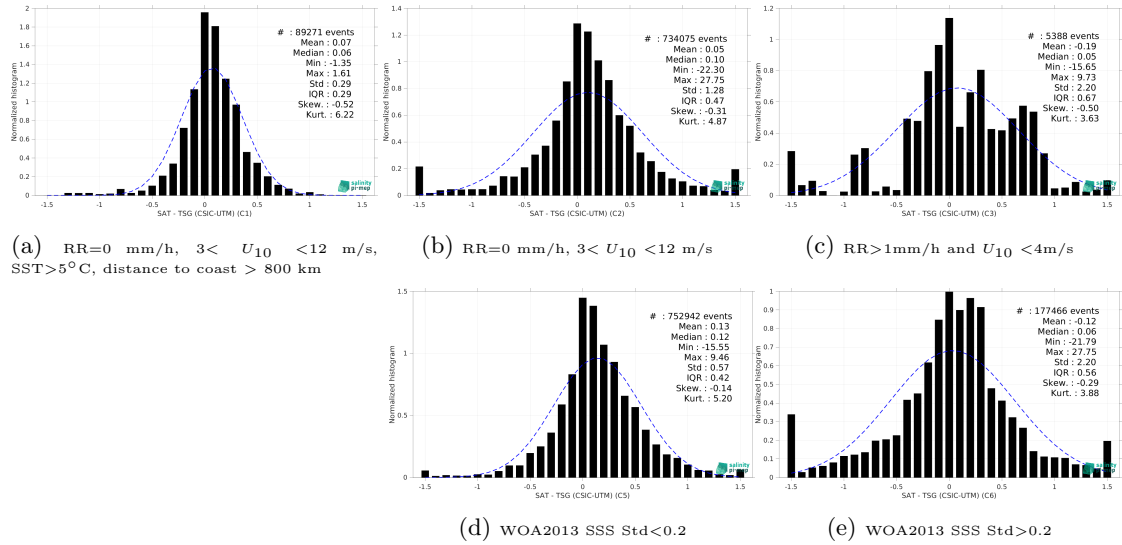
Figure 15: Normalized histogram of \Delta SSS (SMAP SSS L3 v5.0 - 8-Day running (JPL) - TSG (CSIC-UTM)) for 5 different subdatasets corresponding to: RR=0 mm/h, 3 < U_{10} < 12 m/s, SST > 5°C, distance to coast > 800 km (a), RR=0 mm/h, 3 < U_{10} < 12 m/s (b), RR > 1mm/h and U_{10} < 4 m/s (c), WOA2013 SSS Std < 0.2 (d), WOA2013 SSS Std > 0.2 (e).
