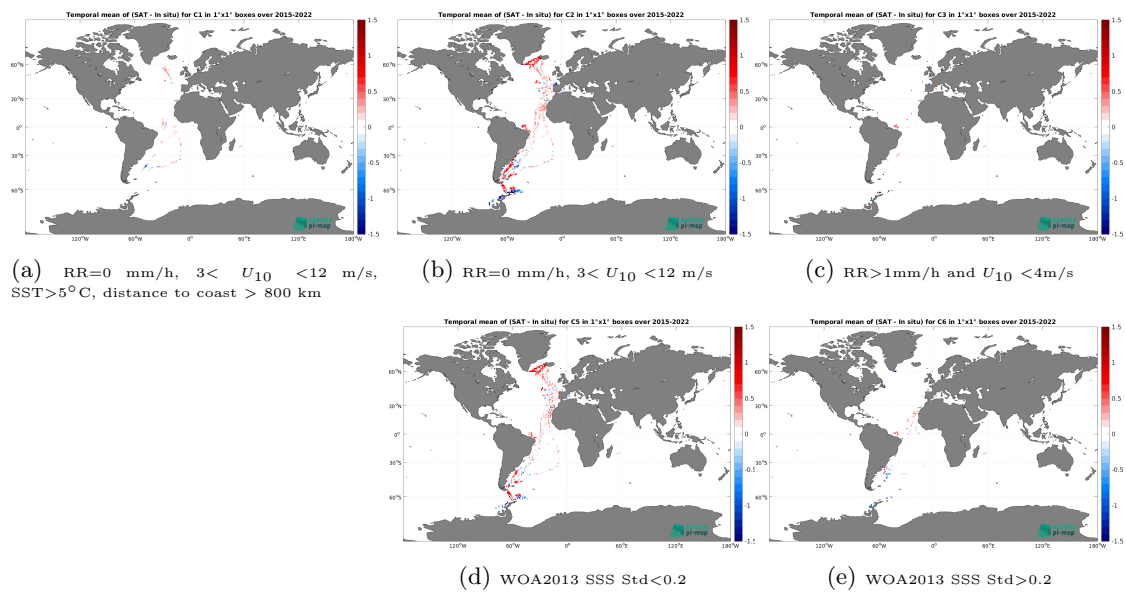
Figure 14: Temporal mean gridded over spatial boxes of size 1^\circ \times 1^\circ of \Delta SSS (SMAP SSS L3 v5.0 - 8-Day running (JPL) - TSG (CSIC-UTM)) for 5 different subdatasets corresponding to:RR=0 mm/h, 3 < U_{10} < 12 m/s, SST > 5^\circ\text{C} , distance to coast > 800 km (a), RR=0 mm/h, 3 < U_{10} < 12 m/s (b), RR > 1 mm/h and U_{10} < 4 m/s (c), WOA2013 SSS Std < 0.2 (d), WOA2013 SSS Std > 0.2 (e).
