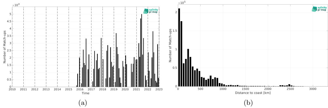
Figure 2: Number of match-ups between TSG (CSIC-UTM) and SMAP SSS L3 v5.0 - 8-Day running (JPL) SSS as a function of time (a) and as function of the distance to coast (b) over the Global Ocean Pi-MEP region and for the full satellite product period.
