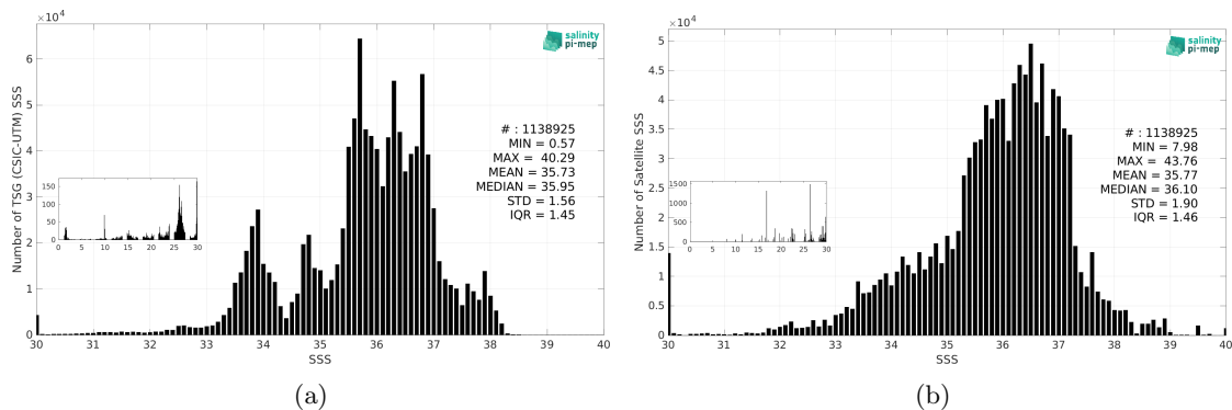
Figure 3: Histograms of SSS from TSG (CSIC-UTM) (a) and SMAP SSS L3 v5.0 - 8-Day running (JPL) (b) considering all match-up pairs per bins of 0.1 over the Global Ocean Pi-MEP region and for the full satellite product period.
