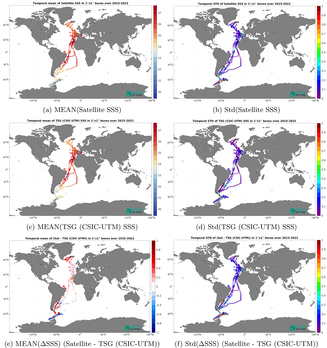
Figure 7: Temporal mean (left) and Std (right) of SSS from SMAP SSS L3 v5.0 - 8-Day running (JPL) (top), TSG (CSIC-UTM) (middle), and of \Delta SSS (Satellite - TSG (CSIC-UTM)). Only match-up pairs are used to generate these maps.
