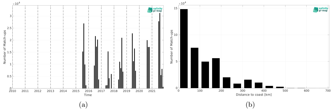
Figure 2: Number of match-ups between TSG (Amundsen) and SMAP SSS L3 v5.0 - 8-Day running (JPL) SSS as a function of time (a) and as function of the distance to coast (b) over the Global Ocean Pi-MEP region and for the full satellite product period.
