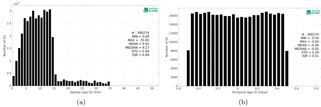
Figure 6: Histograms of the spatial (a) and temporal (b) lags between the location/time of the TSG (Amundsen) measurement and the date of the corresponding SMAP SSS L3 v5.0 - 8-Day running (JPL) SSS pixel.
