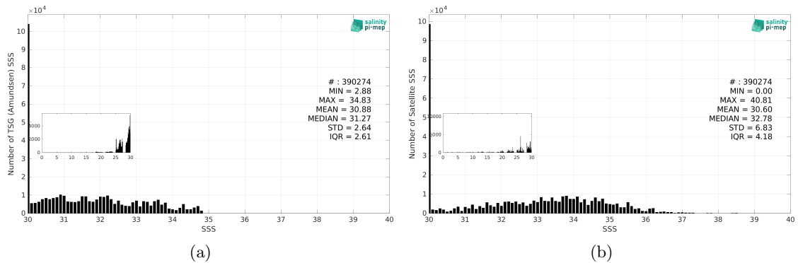
Figure 3: Histograms of SSS from TSG (Amundsen) (a) and SMAP SSS L3 v5.0 - 8-Day running (JPL) (b) considering all match-up pairs per bins of 0.1 over the Global Ocean Pi-MEP region and for the full satellite product period.
