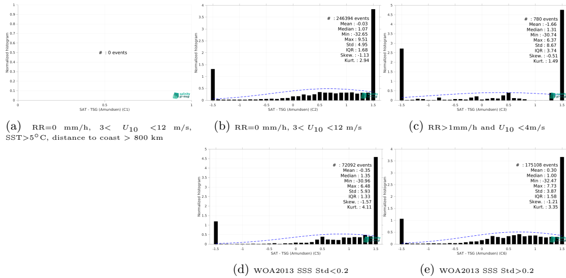
Figure 15: Normalized histogram of \Delta SSS (SMAP SSS L3 v5.0 - 8-Day running (JPL) - TSG (Amundsen)) for 5 different subdatasets corresponding to: RR=0 mm/h, 3 < U_{10} < 12 m/s, SST > 5°C, distance to coast > 800 km (a), RR=0 mm/h, 3 < U_{10} < 12 m/s (b), RR > 1mm/h and U_{10} < 4 m/s (c), WOA2013 SSS Std < 0.2 (d), WOA2013 SSS Std > 0.2 (e).
