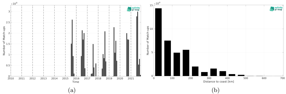
Figure 1: Number of match-ups between TSG (Amundsen) and SMAP SSS L3 v5.0 - 8-Day running (JPL) SSS as a function of time (a) and as function of the distance to coast (b) over the Global Ocean Pi-MEP region and for the full satellite product period.
