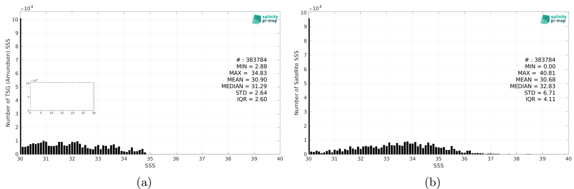
Figure 2: Histograms of SSS from TSG (Amundsen) (a) and SMAP SSS L3 v5.0 - 8-Day running (JPL) (b) considering all match-up pairs per bins of 0.1 over the Global Ocean Pi-MEP region and for the full satellite product period.
