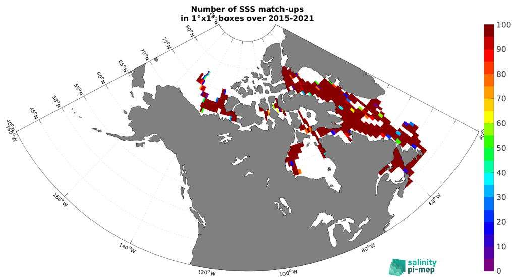
Figure 4: Number of SSS match-ups between TSG (Amundsen) SSS and the SMAP SSS L3 v5.0 - 8-Day running (JPL) SSS product for the Global Ocean Pi-MEP region over 1^\circ \times 1^\circ boxes and for the full satellite product period.
