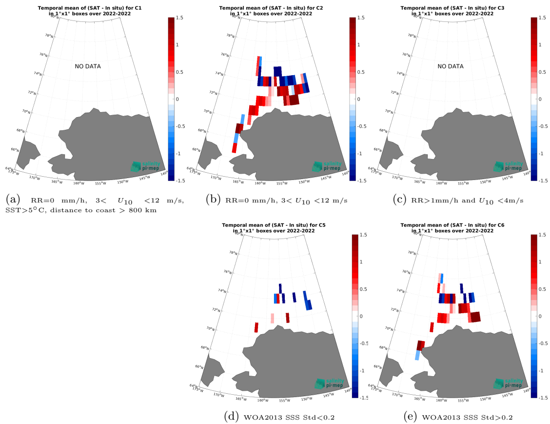
Figure 14: Temporal mean gridded over spatial boxes of size 1^\circ \times 1^\circ of \Delta\text{SSS} (SMAP SSS L3 v5.0 - 8-Day running (JPL) - SASSIE) for 5 different subdatasets corresponding to:RR=0 mm/h, 3 < U_{10} < 12 m/s, SST>5°C, distance to coast > 800 km (a), RR=0 mm/h, 3 < U_{10} < 12 m/s (b), RR>1mm/h and U_{10} < 4 m/s (c), WOA2013 SSS Std<0.2 (d), WOA2013 SSS Std>0.2 (e).
