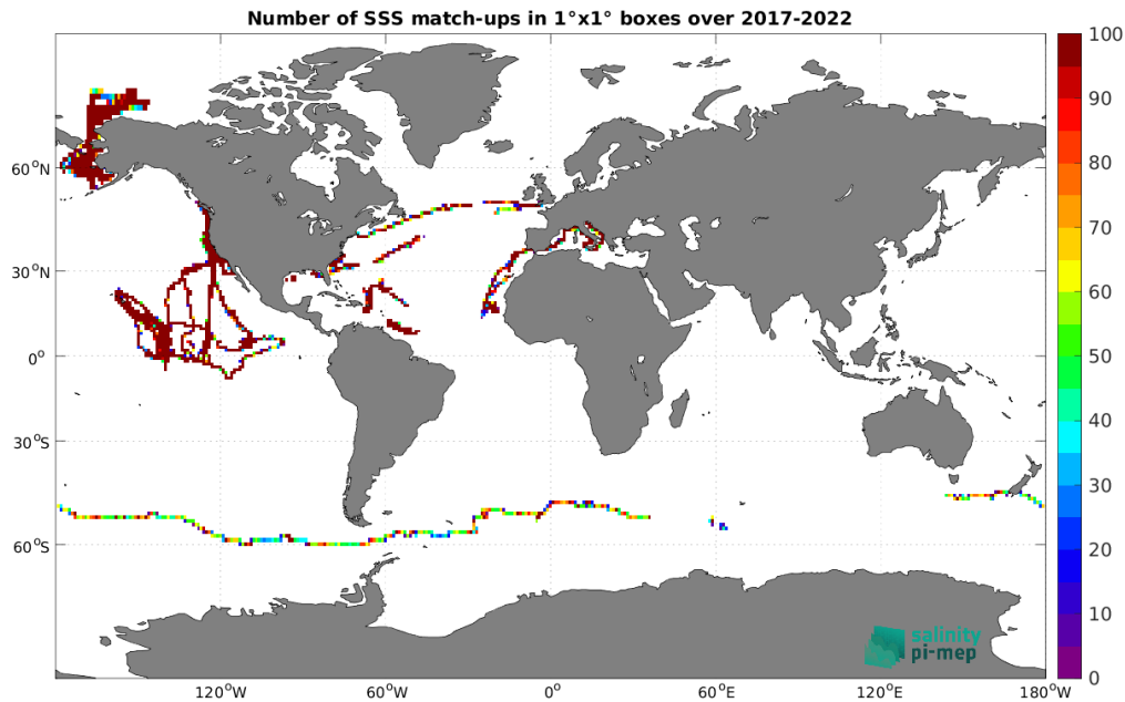
Figure 5: Number of SSS match-ups between Saildrone SSS and the SMAP SSS L3 v5.0 - 8-Day running (JPL) SSS product for the Global Ocean Pi-MEP region over 1^\circ \times 1^\circ boxes and for the full satellite product period.
