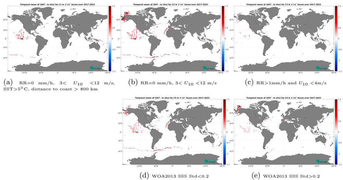
Figure 14: Temporal mean gridded over spatial boxes of size 1^\circ \times 1^\circ of \Delta SSS (SMAP SSS L3 v5.0 - 8-Day running (JPL) - Sairdrone) for 5 different subdatasets corresponding to:RR=0 mm/h, 3 < U_{10} < 12 m/s, SST > 5°C, distance to coast > 800 km (a), RR=0 mm/h, 3 < U_{10} < 12 m/s (b), RR > 1mm/h and U_{10} < 4 m/s (c), WOA2013 SSS Std < 0.2 (d), WOA2013 SSS Std > 0.2 (e).
