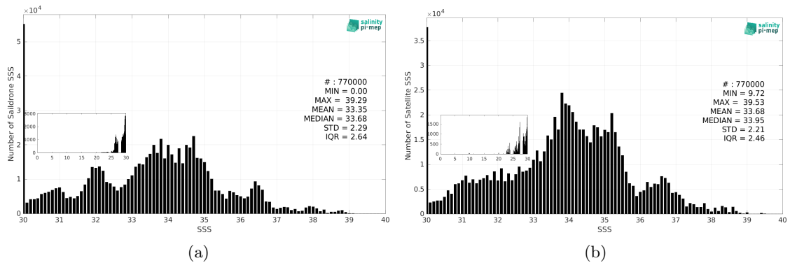
Figure 3: Histograms of SSS from Sairdrone (a) and SMAP SSS L3 v5.0 - 8-Day running (JPL) (b) considering all match-up pairs per bins of 0.1 over the Global Ocean Pi-MEP region and for the full satellite product period.
