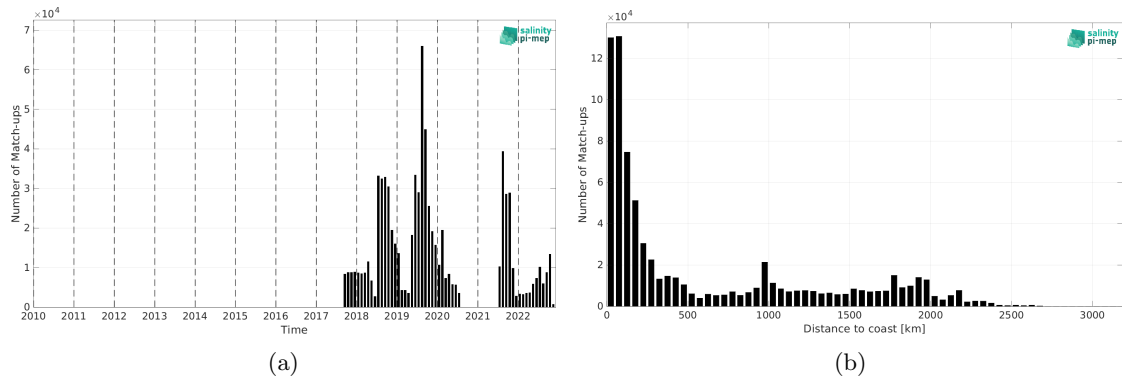
Figure 2: Number of match-ups between Sairdrone and SMAP SSS L3 v5.0 - 8-Day running (JPL) SSS as a function of time (a) and as function of the distance to coast (b) over the Global Ocean Pi-MEP region and for the full satellite product period.
