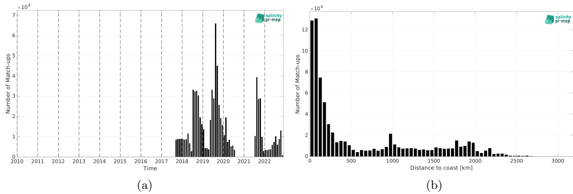
Figure 1: Number of match-ups between Sairdrone and SMAP SSS L3 v5.0 - 8-Day running (JPL) SSS as a function of time (a) and as function of the distance to coast (b) over the Global Ocean Pi-MEP region and for the full satellite product period.
