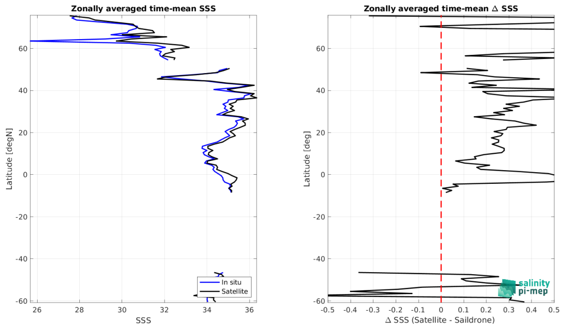
Figure 8: Left panel: Zonal mean SSS from SMAP SSS L3 v5.0 - 8-Day running (JPL) satellite product (black) and from Sairdrone (blue). Right panel: Zonal mean of \Delta SSS (Satellite - Sairdrone) for all the collected Pi-MEP match-up pairs estimated over the full satellite product period.
