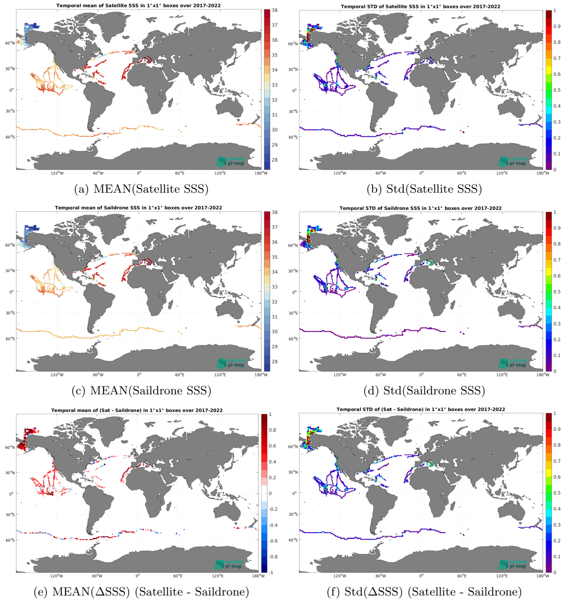
Figure 6: Temporal mean (left) and Std (right) of SSS from SMAP SSS L3 v5.0 - 8-Day running (JPL) (top), Saildrone (middle), and of \Delta SSS (Satellite - Saildrone). Only match-up pairs are used to generate these maps.
