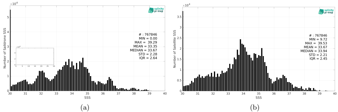
Figure 2: Histograms of SSS from Sairdrone (a) and SMAP SSS L3 v5.0 - 8-Day running (JPL) (b) considering all match-up pairs per bins of 0.1 over the Global Ocean Pi-MEP region and for the full satellite product period.
