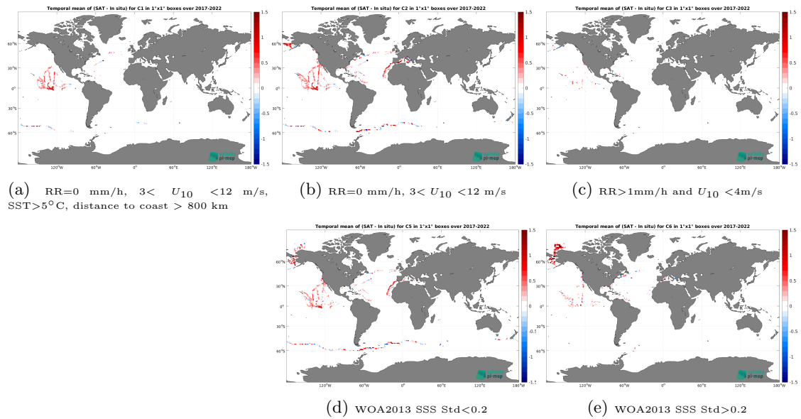
Figure 12: Temporal mean gridded over spatial boxes of size 1^\circ \times 1^\circ of \Delta SSS (SMAP SSS L3 v5.0 - 8-Day running (JPL) - Sailability) for 5 different subdatasets corresponding to:RR=0 mm/h, 3 < U_{10} < 12 m/s, SST > 5^\circ\text{C} , distance to coast > 800 km (a), RR=0 mm/h, 3 < U_{10} < 12 m/s (b), RR > 1 mm/h and U_{10} < 4 m/s (c), WOA2013 SSS Std < 0.2 (d), WOA2013 SSS Std > 0.2 (e).
