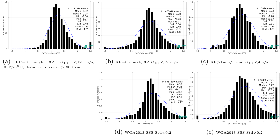
Figure 13: Normalized histogram of \Delta\text{SSS} (SMAP SSS L3 v5.0 - 8-Day running (JPL) - Saiclone) for 5 different subdatasets corresponding to: RR=0 mm/h, 3 < U_{10} < 12 m/s, SST>5°C, distance to coast > 800 km (a), RR=0 mm/h, 3 < U_{10} < 12 m/s (b), RR>1mm/h and U_{10} < 4 m/s (c), WOA2013 SSS Std<0.2 (d), WOA2013 SSS Std>0.2 (e).
