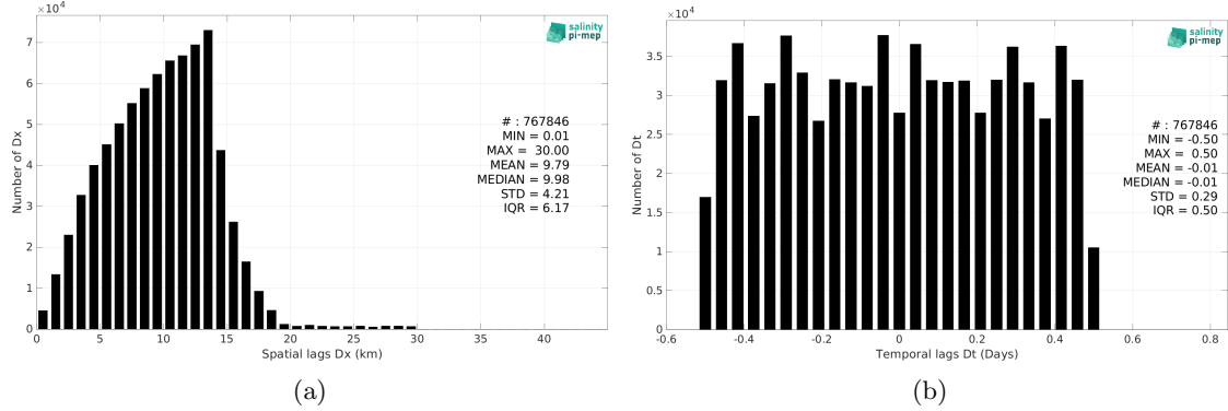
Figure 5: Histograms of the spatial (a) and temporal (b) lags between the location/time of the Saildrone measurement and the date of the corresponding SMAP SSS L3 v5.0 - 8-Day running (JPL) SSS pixel.
