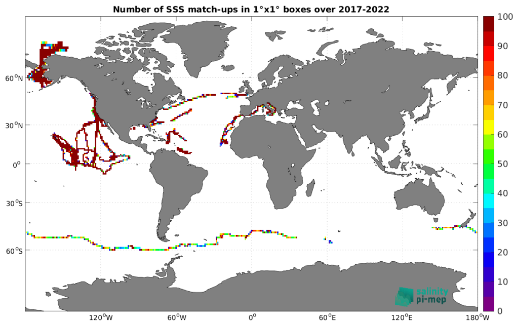
Figure 4: Number of SSS match-ups between Saildrone SSS and the SMAP SSS L3 v5.0 - 8-Day running (JPL) SSS product for the Global Ocean Pi-MEP region over 1^\circ \times 1^\circ boxes and for the full satellite product period.
