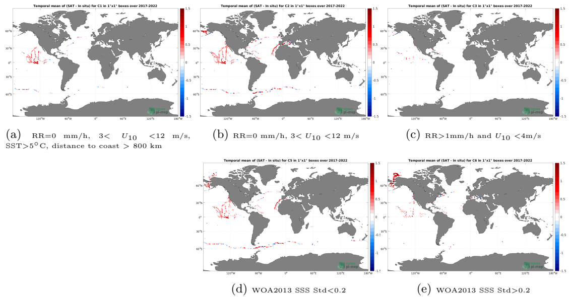
Figure 12: Temporal mean gridded over spatial boxes of size 1^\circ \times 1^\circ of \Delta SSS (SMAP SSS L3 v5.0 - 8-Day running (JPL) - Sairdrone) for 5 different subdatasets corresponding to:RR=0 mm/h, 3 < U_{10} < 12 m/s, SST > 5^\circ\text{C} , distance to coast > 800 km (a), RR=0 mm/h, 3 < U_{10} < 12 m/s (b), RR > 1 mm/h and U_{10} < 4 m/s (c), WOA2013 SSS Std < 0.2 (d), WOA2013 SSS Std > 0.2 (e).
