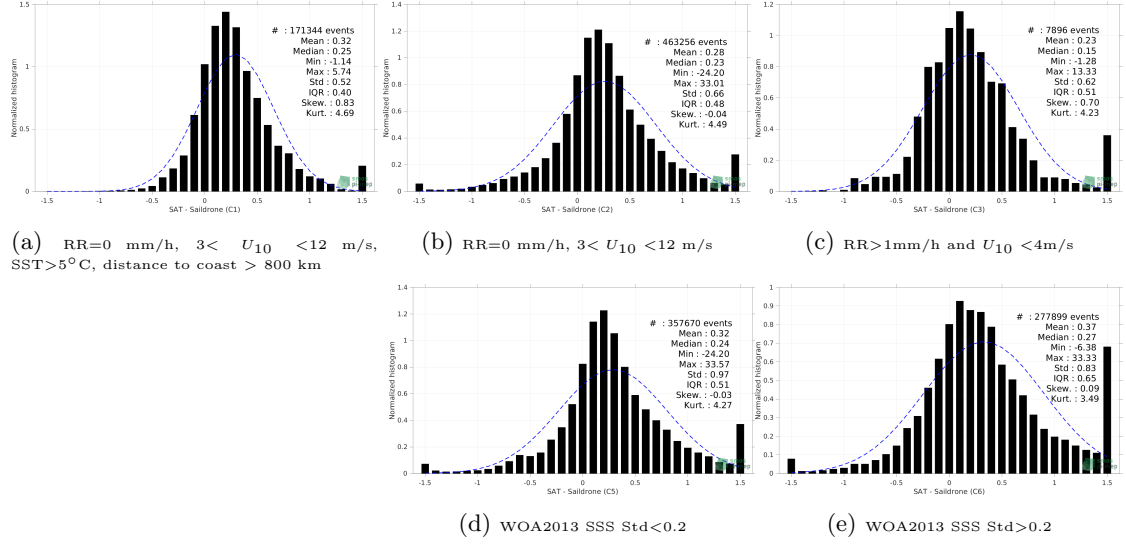
Figure 13: Normalized histogram of \Delta SSS (SMAP SSS L3 v5.0 - 8-Day running (JPL) - Sairdron) for 5 different subdatasets corresponding to: RR=0 mm/h, 3 < U_{10} < 12 m/s, SST > 5°C, distance to coast > 800 km (a), RR=0 mm/h, 3 < U_{10} < 12 m/s (b), RR > 1mm/h and U_{10} < 4 m/s (c), WOA2013 SSS Std < 0.2 (d), WOA2013 SSS Std > 0.2 (e).
