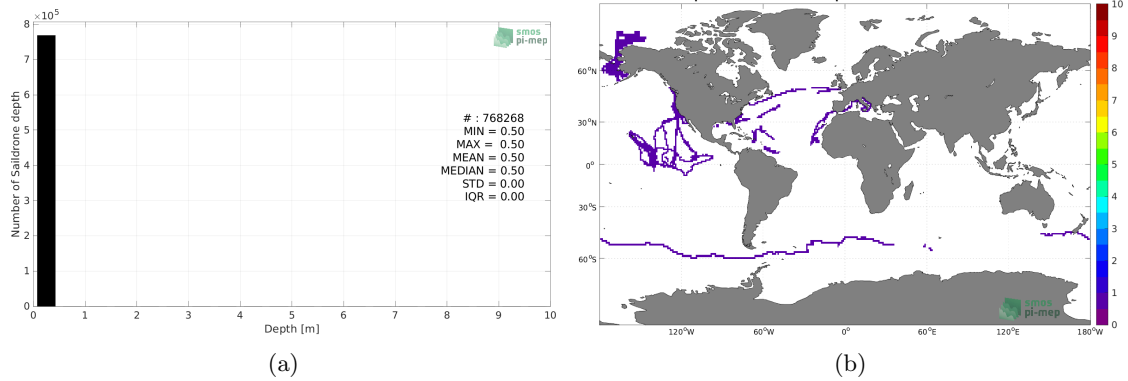
Figure 3: Histograms of the depth of the upper level SSS measurements from Saildrone in the Match-up DataBase for the Global Ocean Pi-MEP region (a) and temporal mean spatial distribution of pressure of the in situ SSS data over 1^\circ \times 1^\circ boxes and for the full satellite product period (b).
