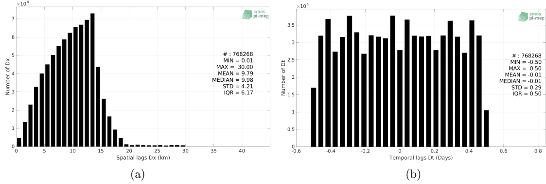
Figure 5: Histograms of the spatial (a) and temporal (b) lags between the location/time of the Sairdrone measurement and the date of the corresponding SMAP SSS L3 v5.0 - 8-Day running (JPL) SSS pixel.
