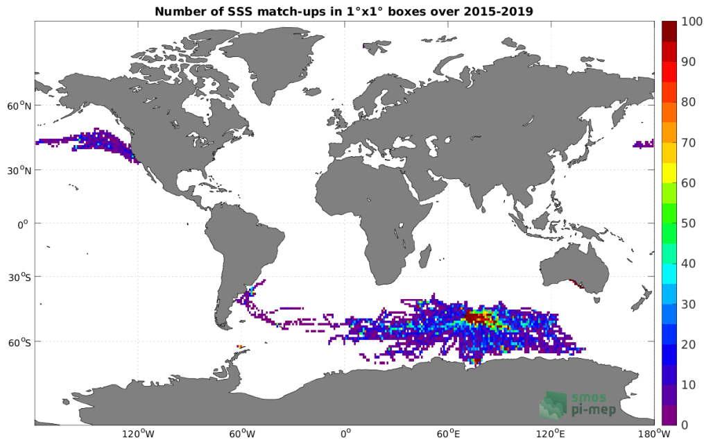
Figure 4: Number of SSS match-ups between Marine mammals SSS and the SMAP SSS L3 v5.0 - 8-Day running (JPL) SSS product for the Global Ocean Pi-MEP region over 1^\circ \times 1^\circ boxes and for the full satellite product period.
