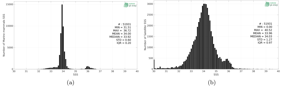
Figure 2: Histograms of SSS from Marine mammals (a) and SMAP SSS L3 v5.0 - 8-Day running (JPL) (b) considering all match-up pairs per bins of 0.1 over the Global Ocean Pi-MEP region and for the full satellite product period.
