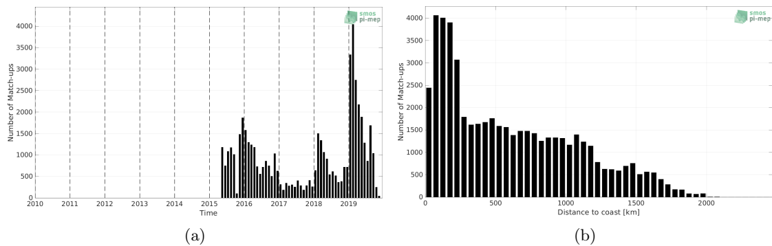
Figure 1: Number of match-ups between Marine mammals and SMAP SSS L3 v5.0 - 8-Day running (JPL) SSS as a function of time (a) and as function of the distance to coast (b) over the Global Ocean Pi-MEP region and for the full satellite product period.
