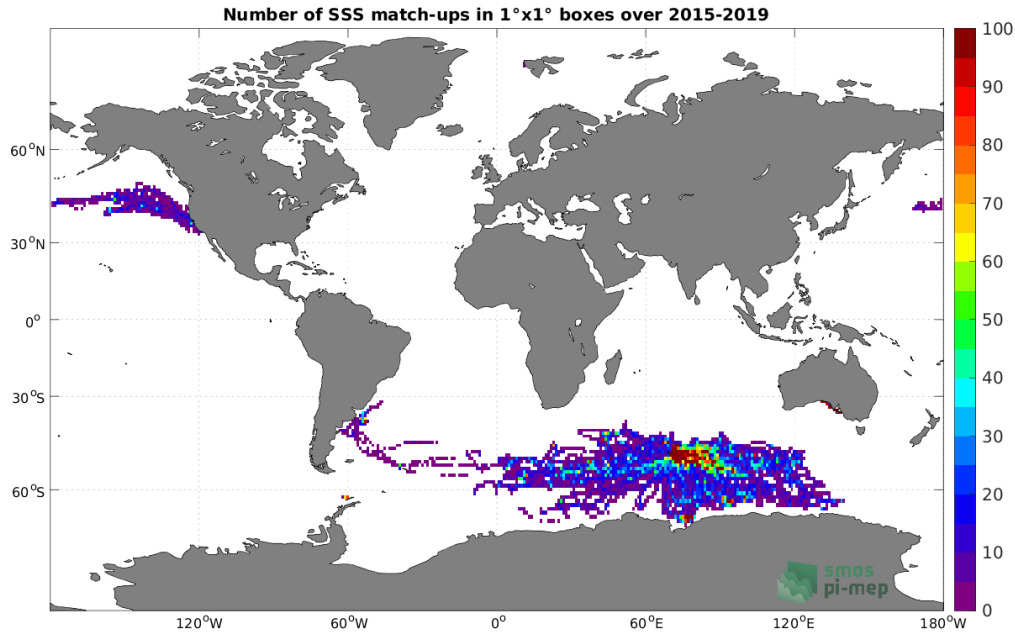
Figure 4: Number of SSS match-ups between Marine mammals SSS and the SMAP SSS L3 v5.0 - 8-Day running (JPL) SSS product for the Global Ocean Pi-MEP region over 1°x1° boxes and for the full satellite product period.
