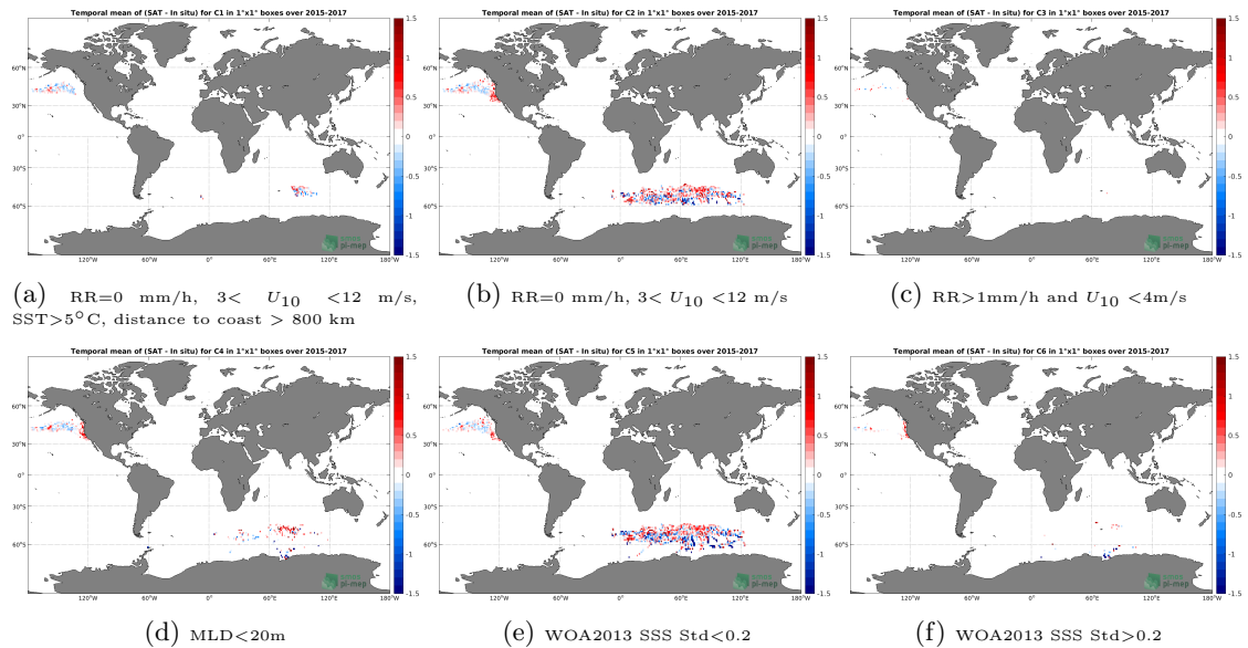
Figure 12: Temporal mean gridded over spatial boxes of size 1°x1° of \Delta SSS (SMAP SSS L3 v5.0 - 8-Day running (JPL) - Sea mammals) for 6 different subdatasets corresponding to:RR=0 mm/h, 3 < U_{10} < 12 m/s, SST>5°C, distance to coast > 800 km (a), RR=0 mm/h, 3 < U_{10} < 12 m/s (b), RR>1mm/h and U_{10} < 4 m/s (c),MLD<20m (d),WOA2013 SSS Std<0.2 (e),WOA2013 SSS Std>0.2 (f).
