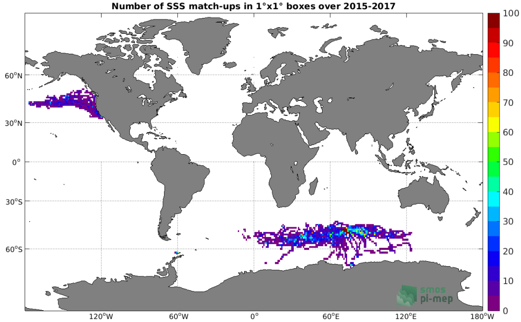
Figure 4: Number of SSS match-ups between Sea mammals SSS and the SMAP SSS L3 v5.0 - 8-Day running (JPL) SSS product for the Global Ocean Pi-MEP region over 1°x1° boxes and for the full satellite product period.
