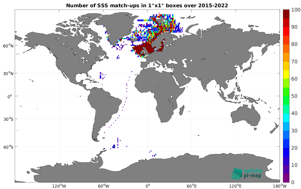
Figure 4: Number of SSS match-ups between ICES SSS and the SMAP SSS L3 v5.0 - 8-Day running (JPL) SSS product for the Global Ocean Pi-MEP region over 1^\circ \times 1^\circ boxes and for the full satellite product period.
