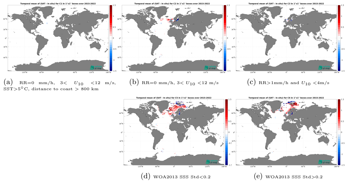
Figure 12: Temporal mean gridded over spatial boxes of size 1^\circ \times 1^\circ of \Delta SSS (SMAP SSS L3 v5.0 - 8-Day running (JPL) - ICES) for 5 different subdatasets corresponding to:RR=0 mm/h, 3 < U_{10} < 12 m/s, SST >5^\circ C, distance to coast > 800 km (a), RR=0 mm/h, 3 < U_{10} < 12 m/s (b), RR >1 mm/h and U_{10} < 4 m/s (c), WOA2013 SSS Std <0.2 (d), WOA2013 SSS Std >0.2 (e).
