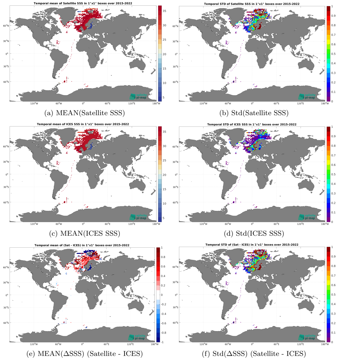
Figure 6: Temporal mean (left) and Std (right) of SSS from SMAP SSS L3 v5.0 - 8-Day running (JPL) (top), ICES (middle), and of \Delta SSS (Satellite - ICES). Only match-up pairs are used to generate these maps.
