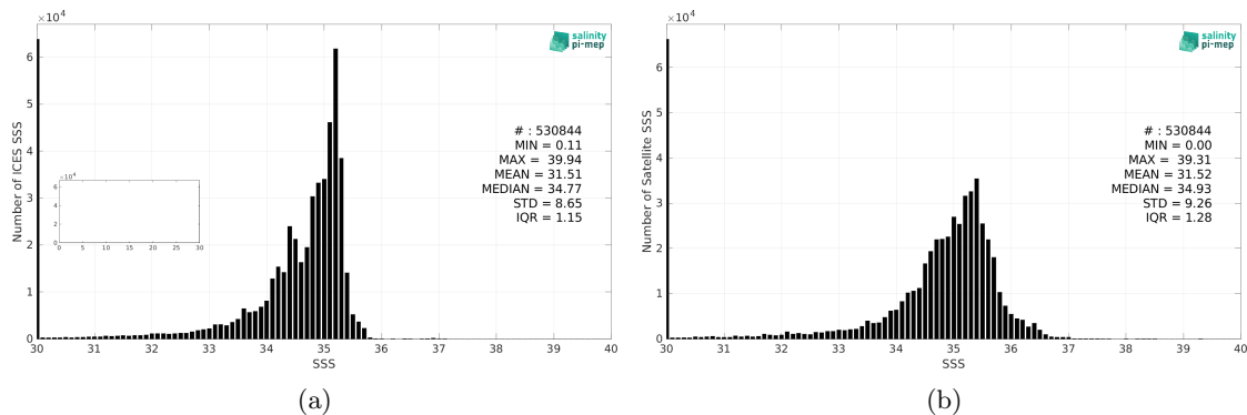
Figure 2: Histograms of SSS from ICES (a) and SMAP SSS L3 v5.0 - 8-Day running (JPL) (b) considering all match-up pairs per bins of 0.1 over the Global Ocean Pi-MEP region and for the full satellite product period.
