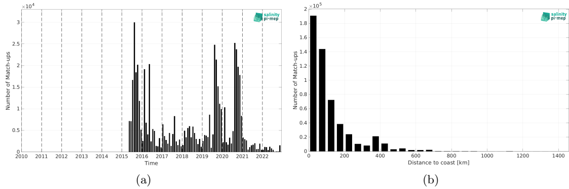
Figure 1: Number of match-ups between ICES and SMAP SSS L3 v5.0 - 8-Day running (JPL) SSS as a function of time (a) and as function of the distance to coast (b) over the Global Ocean Pi-MEP region and for the full satellite product period.
