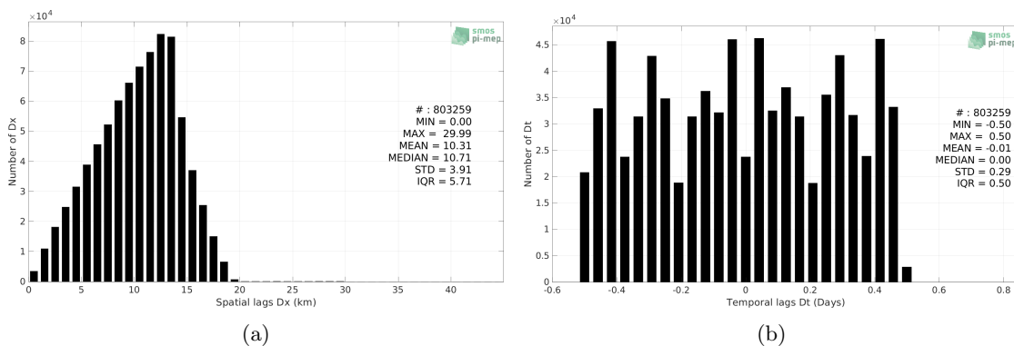
Figure 4: Histograms of the spatial (a) and temporal (b) lags between the location/time of the Surface drifters measurement and the date of the corresponding SMAP SSS L3 v5.0 - 8-Day running (JPL) SSS pixel.
