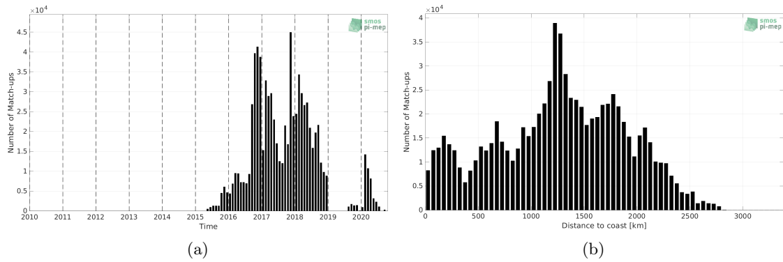
Figure 1: Number of match-ups between Surface drifters and SMAP SSS L3 v5.0 - 8-Day running (JPL) SSS as a function of time (a) and as function of the distance to coast (b) over the Global Ocean Pi-MEP region and for the full satellite product period.
