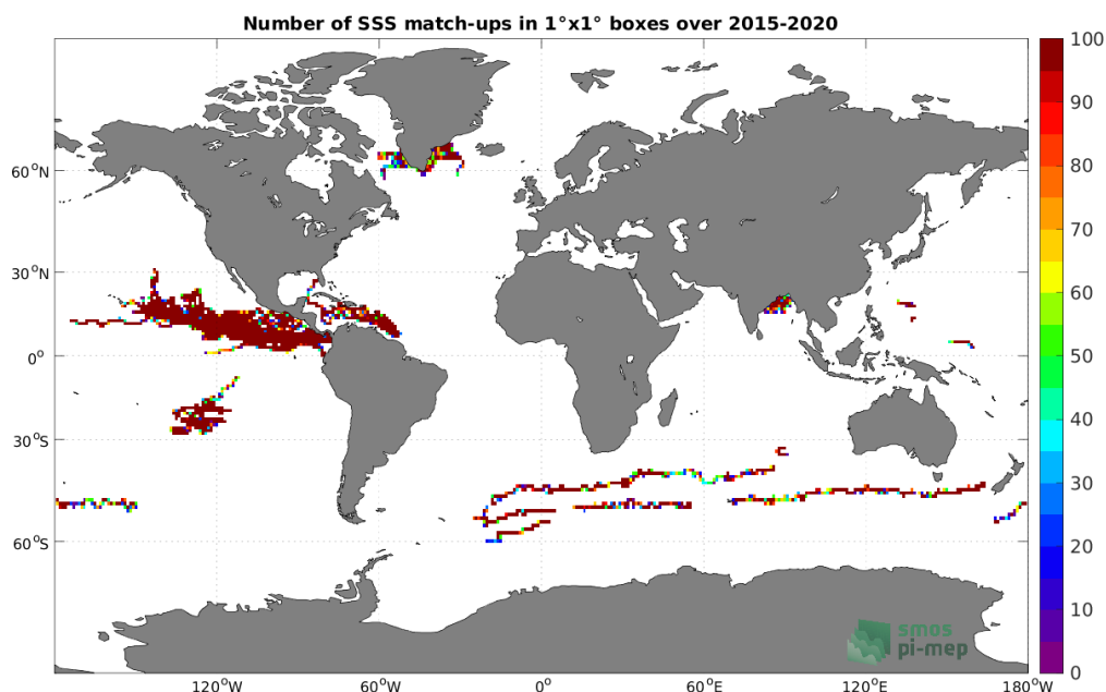
Figure 3: Number of SSS match-ups between Surface drifters SSS and the SMAP SSS L3 v5.0 - 8-Day running (JPL) SSS product for the Global Ocean Pi-MEP region over 1^\circ \times 1^\circ boxes and for the full satellite product period.
