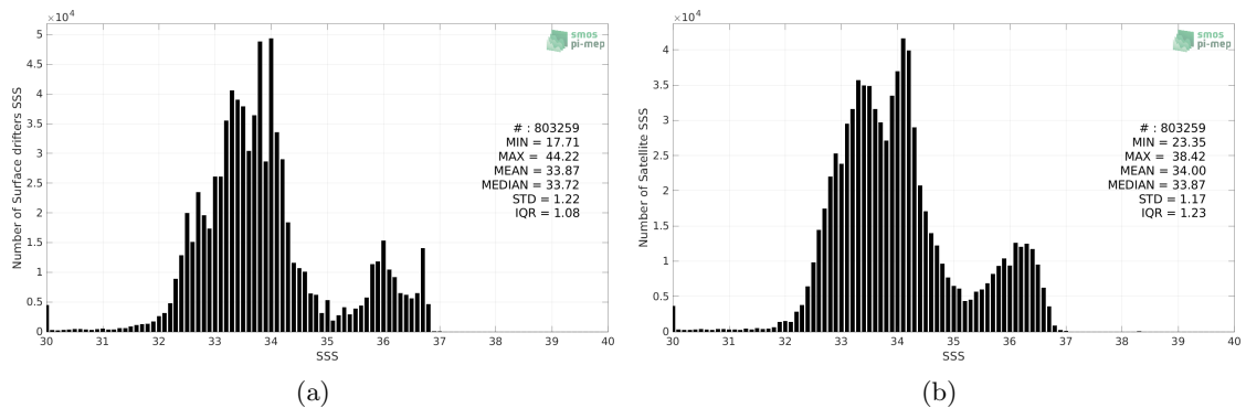
Figure 2: Histograms of SSS from Surface drifters (a) and SMAP SSS L3 v5.0 - 8-Day running (JPL) (b) considering all match-up pairs per bins of 0.1 over the Global Ocean Pi-MEP region and for the full satellite product period.
