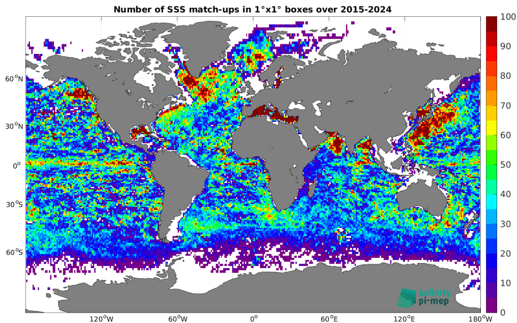
Figure 5: Number of SSS match-ups between Argo SSS and the SMAP SSS L3 v5.0 - 8-Day running (JPL) SSS product for the Global Ocean Pi-MEP region over 1^\circ \times 1^\circ boxes and for the full satellite product period.
