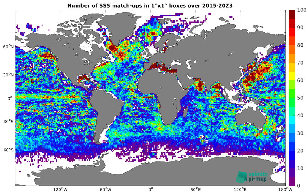
Figure 4: Number of SSS match-ups between Argos SSS and the SMAP SSS L3 v5.0 - 8-Day running (JPL) SSS product for the Global Ocean Pi-MEP region over 1^\circ \times 1^\circ boxes and for the full satellite product period.
