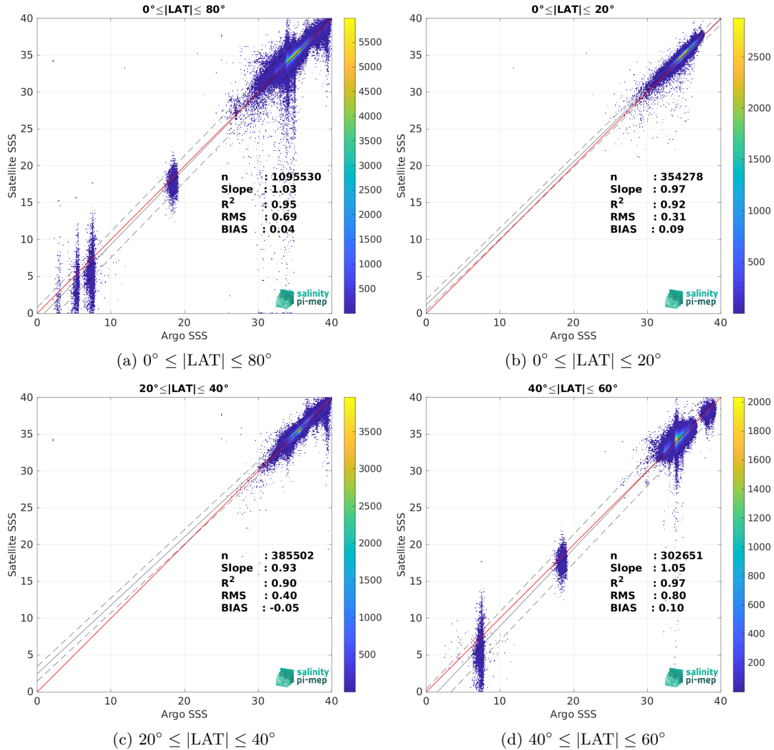
Figure 9: Contour maps of the concentration of SMAP SSS L3 v5.0 - 8-Day running (JPL) SSS (y-axis) versus Argo SSS (x-axis) at match-up pairs for different latitude bands. For each plot, the red line shows x=y . The black thin and dashed lines indicate a linear fit through the data cloud and the \pm 95\% confidence levels, respectively. The number match-up pairs n , the slope and R^2 coefficient of the linear fit, the root mean square (RMS) and the mean bias between satellite and in situ data are indicated for each latitude band in each plot.
