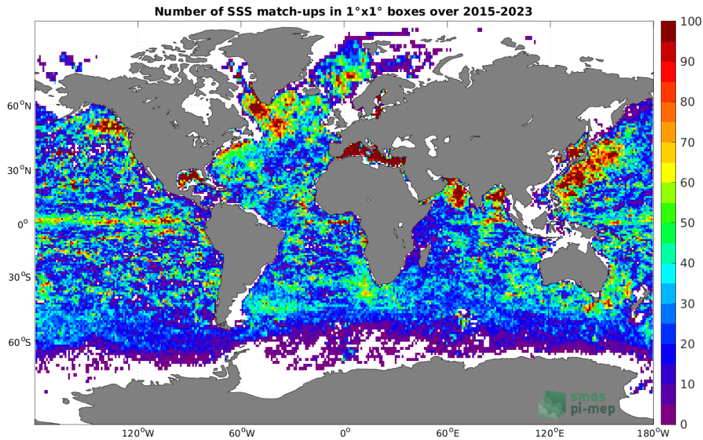
Figure 4: Number of SSS match-ups between Argo SSS and the SMAP SSS L3 v5.0 - 8-Day running (JPL) SSS product for the Global Ocean Pi-MEP region over 1^\circ \times 1^\circ boxes and for the full satellite product period.
