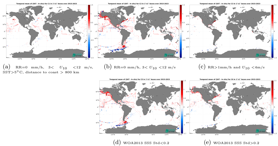
Figure 14: Temporal mean gridded over spatial boxes of size 1^\circ \times 1^\circ of \Delta SSS (SMAP SSS L3 v5.0 - Monthly (JPL) - TSG (SAMOS)) for 5 different subdatasets corresponding to:RR=0 mm/h, 3 < U_{10} < 12 m/s, SST > 5^\circ\text{C} , distance to coast > 800 km (a), RR=0 mm/h, 3 < U_{10} < 12 m/s (b), RR > 1 mm/h and U_{10} < 4 m/s (c), WOA2013 SSS Std < 0.2 (d), WOA2013 SSS Std > 0.2 (e).
