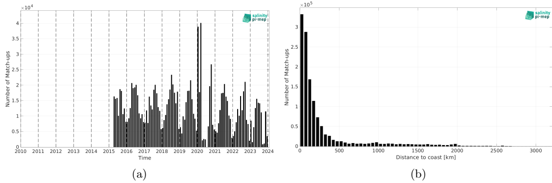
Figure 2: Number of match-ups between TSG (SAMOS) and SMAP SSS L3 v5.0 - Monthly (JPL) SSS as a function of time (a) and as function of the distance to coast (b) over the Global Ocean Pi-MEP region and for the full satellite product period.
