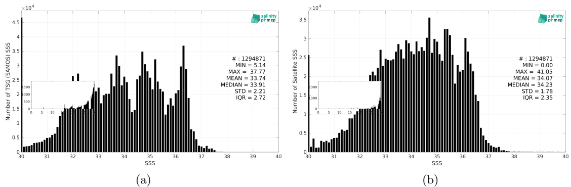
Figure 3: Histograms of SSS from TSG (SAMOS) (a) and SMAP SSS L3 v5.0 - Monthly (JPL) (b) considering all match-up pairs per bins of 0.1 over the Global Ocean Pi-MEP region and for the full satellite product period.
