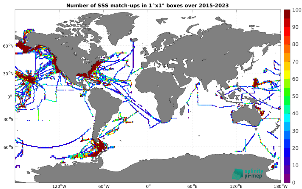
Figure 5: Number of SSS match-ups between TSG (SAMOS) SSS and the SMAP SSS L3 v5.0 - Monthly (JPL) SSS product for the Global Ocean Pi-MEP region over 1^\circ \times 1^\circ boxes and for the full satellite product period.
