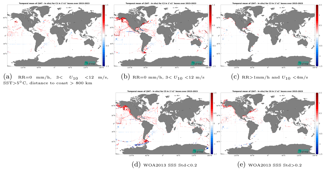
Figure 12: Temporal mean gridded over spatial boxes of size 1^\circ \times 1^\circ of \Delta\text{SSS} (SMAP SSS L3 v5.0 - Monthly (JPL) - TSG (SAMOS)) for 5 different subdatasets corresponding to:RR=0 mm/h, 3 < U_{10} < 12 m/s, SST >5^\circ\text{C} , distance to coast > 800 km (a), RR=0 mm/h, 3 < U_{10} < 12 m/s (b), RR >1 mm/h and U_{10} < 4 m/s (c), WOA2013 SSS Std <0.2 (d), WOA2013 SSS Std >0.2 (e).
