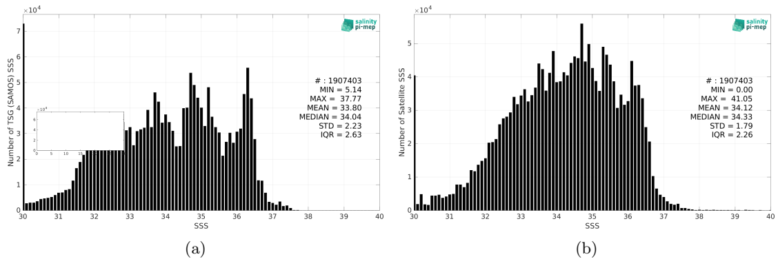
Figure 2: Histograms of SSS from TSG (SAMOS) (a) and SMAP SSS L3 v5.0 - Monthly (JPL) (b) considering all match-up pairs per bins of 0.1 over the Global Ocean Pi-MEP region and for the full satellite product period.
