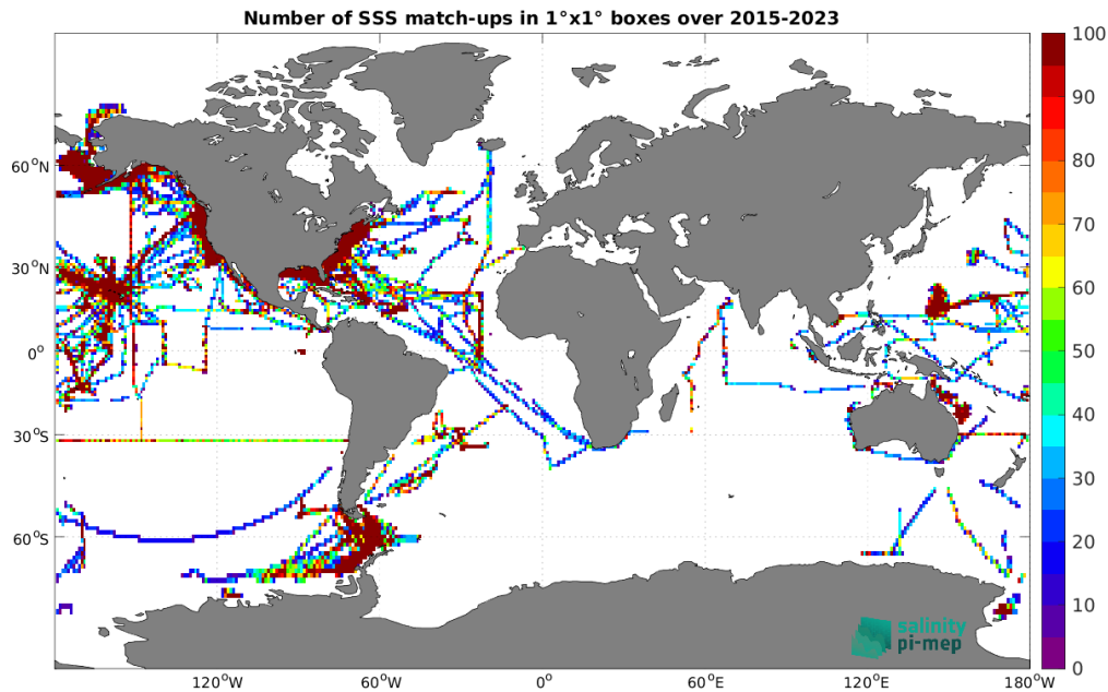
Figure 4: Number of SSS match-ups between TSG (SAMOS) SSS and the SMAP SSS L3 v5.0 - Monthly (JPL) SSS product for the Global Ocean Pi-MEP region over 1^\circ \times 1^\circ boxes and for the full satellite product period.
