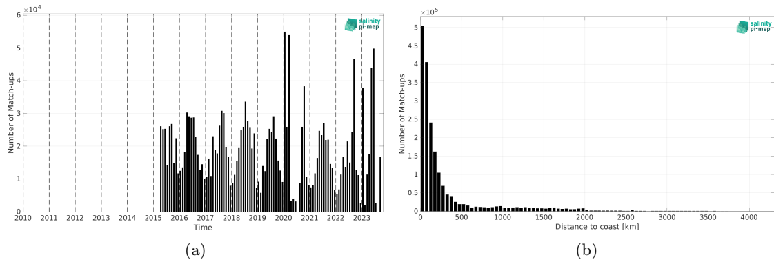
Figure 1: Number of match-ups between TSG (SAMOS) and SMAP SSS L3 v5.0 - Monthly (JPL) SSS as a function of time (a) and as function of the distance to coast (b) over the Global Ocean Pi-MEP region and for the full satellite product period.
