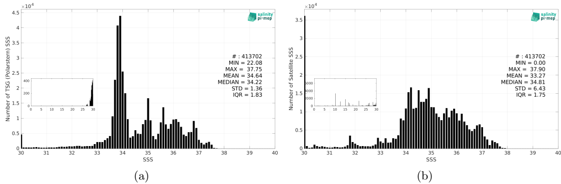
Figure 3: Histograms of SSS from TSG (Polarstern) (a) and SMAP SSS L3 v5.0 - Monthly (JPL) (b) considering all match-up pairs per bins of 0.1 over the Global Ocean Pi-MEP region and for the full satellite product period.
