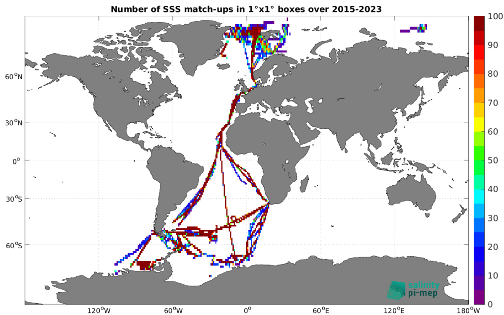
Figure 5: Number of SSS match-ups between TSG (Polarstern) SSS and the SMAP SSS L3 v5.0 - Monthly (JPL) SSS product for the Global Ocean Pi-MEP region over 1^\circ \times 1^\circ boxes and for the full satellite product period.
