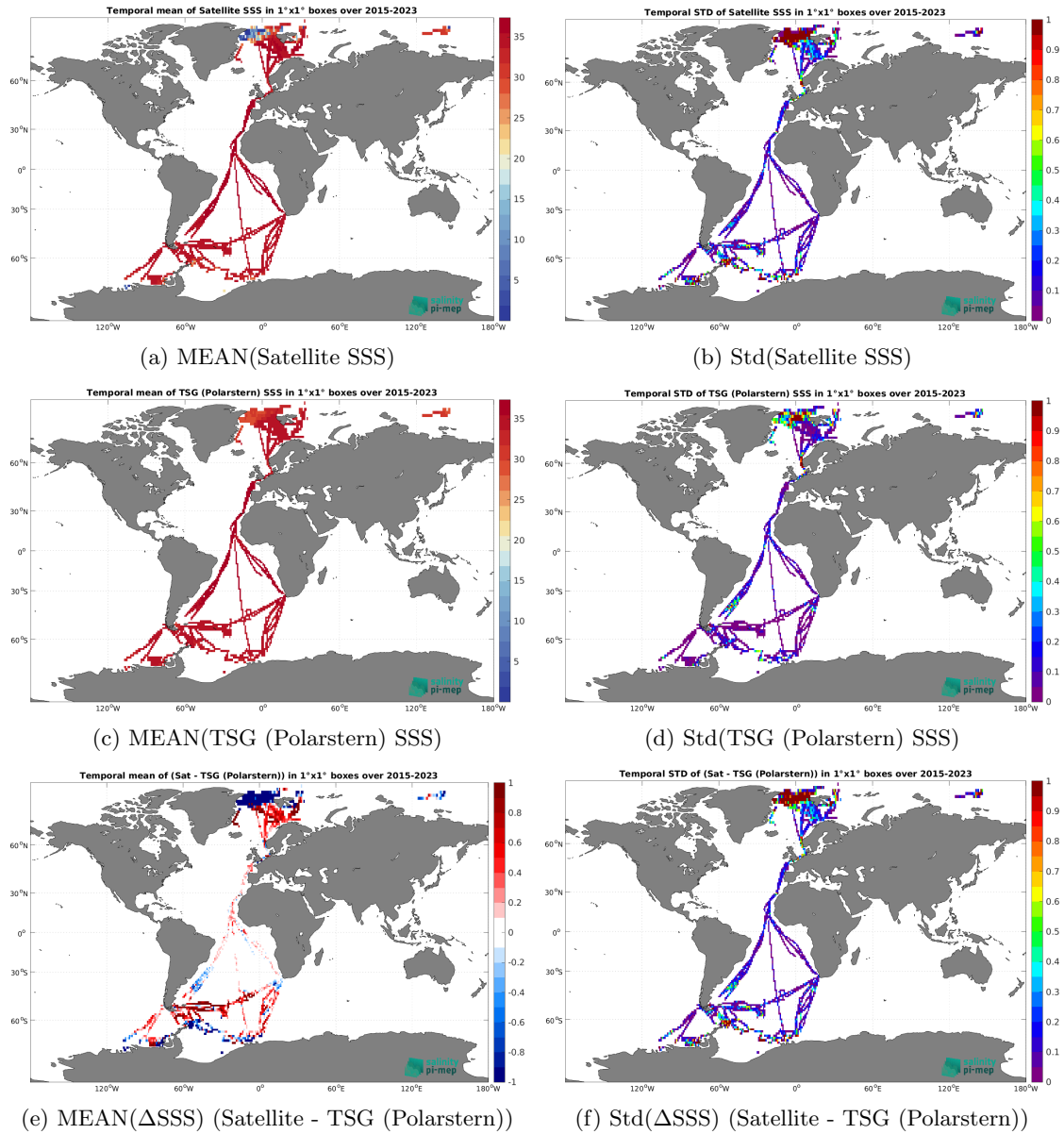
Figure 7: Temporal mean (left) and Std (right) of SSS from SMAP SSS L3 v5.0 - Monthly (JPL) (top), TSG (Polarstern) (middle), and of \Delta SSS (Satellite - TSG (Polarstern)). Only match-up pairs are used to generate these maps.
