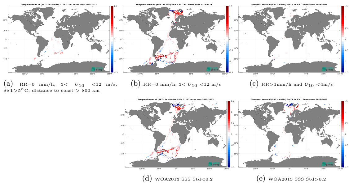
Figure 14: Temporal mean gridded over spatial boxes of size 1^\circ \times 1^\circ of \Delta SSS (SMAP SSS L3 v5.0 - Monthly (JPL) - TSG (Polarstern)) for 5 different subdatasets corresponding to:RR=0 mm/h, 3 < U_{10} < 12 m/s, SST > 5^\circ\text{C} , distance to coast > 800 km (a), RR=0 mm/h, 3 < U_{10} < 12 m/s (b), RR > 1 mm/h and U_{10} < 4 m/s (c), WOA2013 SSS Std < 0.2 (d), WOA2013 SSS Std > 0.2 (e).
