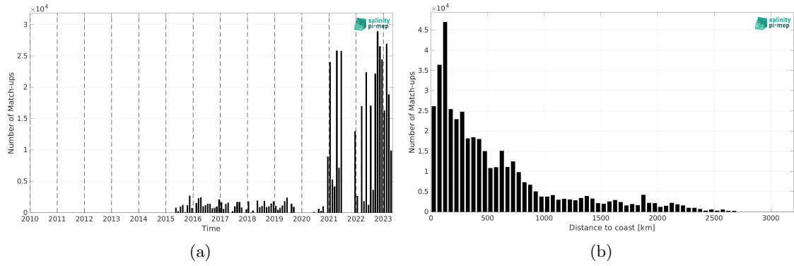
Figure 2: Number of match-ups between TSG (Polarstern) and SMAP SSS L3 v5.0 - Monthly (JPL) SSS as a function of time (a) and as function of the distance to coast (b) over the Global Ocean Pi-MEP region and for the full satellite product period.
