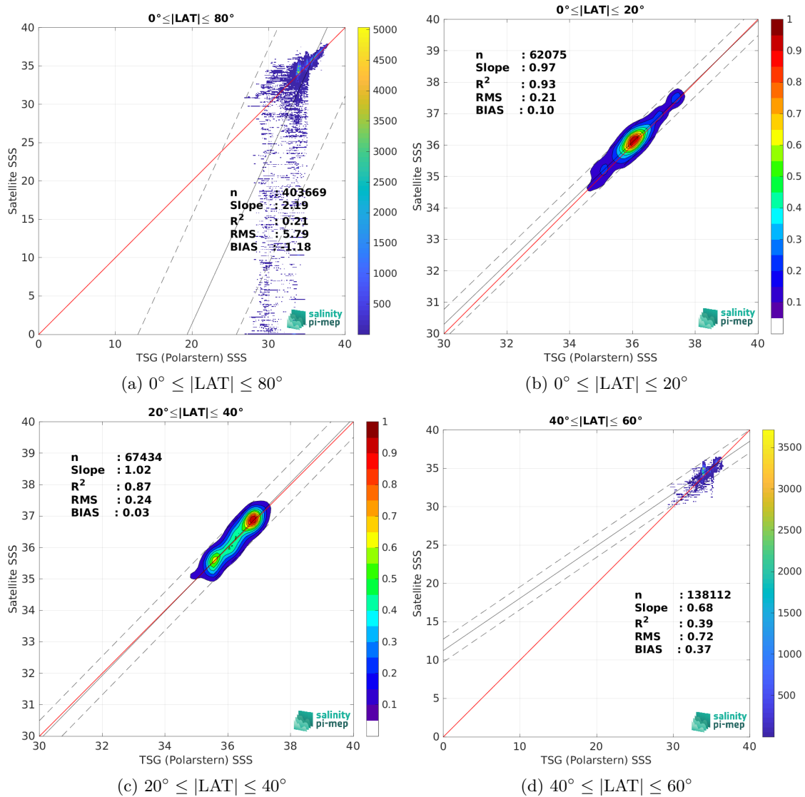
Figure 10: Contour maps of the concentration of SMAP SSS L3 v5.0 - Monthly (JPL) SSS (y-axis) versus TSG (Polarstern) SSS (x-axis) at match-up pairs for different latitude bands. For each plot, the red line shows x=y . The black thin and dashed lines indicate a linear fit through the data cloud and the \pm 95\% confidence levels, respectively. The number match-up pairs n , the slope and R^2 coefficient of the linear fit, the root mean square (RMS) and the mean bias between satellite and in situ data are indicated for each latitude band in each plots.
