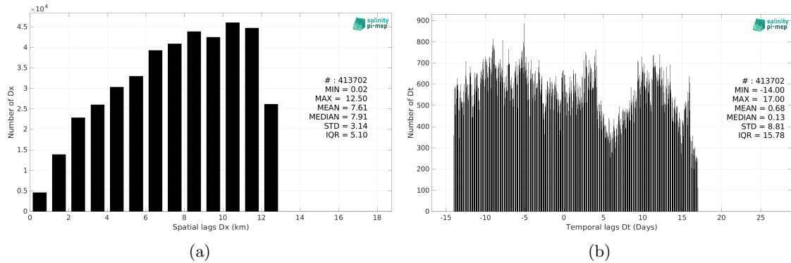
Figure 6: Histograms of the spatial (a) and temporal (b) lags between the location/time of the TSG (Polarstern) measurement and the date of the corresponding SMAP SSS L3 v5.0 - Monthly (JPL) SSS pixel.
