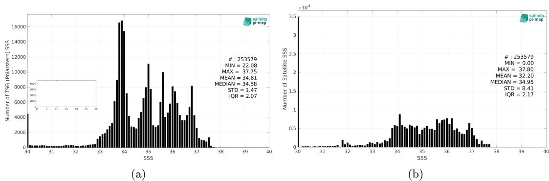
Figure 2: Histograms of SSS from TSG (Polarstern) (a) and SMAP SSS L3 v5.0 - Monthly (JPL) (b) considering all match-up pairs per bins of 0.1 over the Global Ocean Pi-MEP region and for the full satellite product period.
