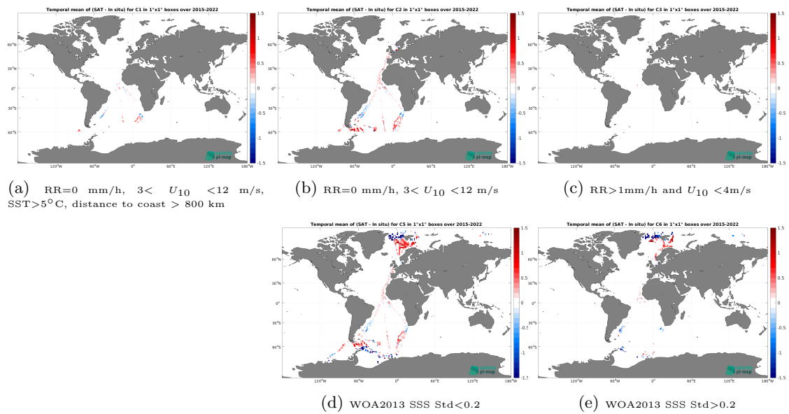
Figure 12: Temporal mean gridded over spatial boxes of size 1^\circ \times 1^\circ of \Delta SSS (SMAP SSS L3 v5.0 - Monthly (JPL) - TSG (Polarstern)) for 5 different subdatasets corresponding to: RR=0 mm/h, 3 < U_{10} < 12 m/s, SST > 5^\circ\text{C} , distance to coast > 800 km (a), RR=0 mm/h, 3 < U_{10} < 12 m/s (b), RR > 1 mm/h and U_{10} < 4 m/s (c), WOA2013 SSS Std < 0.2 (d), WOA2013 SSS Std > 0.2 (e).
