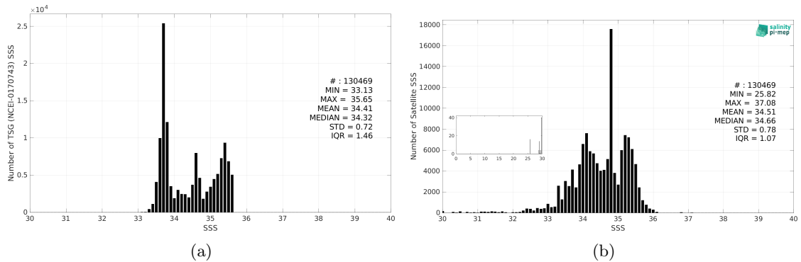
Figure 3: Histograms of SSS from TSG (NCEI-0170743) (a) and SMAP SSS L3 v5.0 - Monthly (JPL) (b) considering all match-up pairs per bins of 0.1 over the Global Ocean Pi-MEP region and for the full satellite product period.
