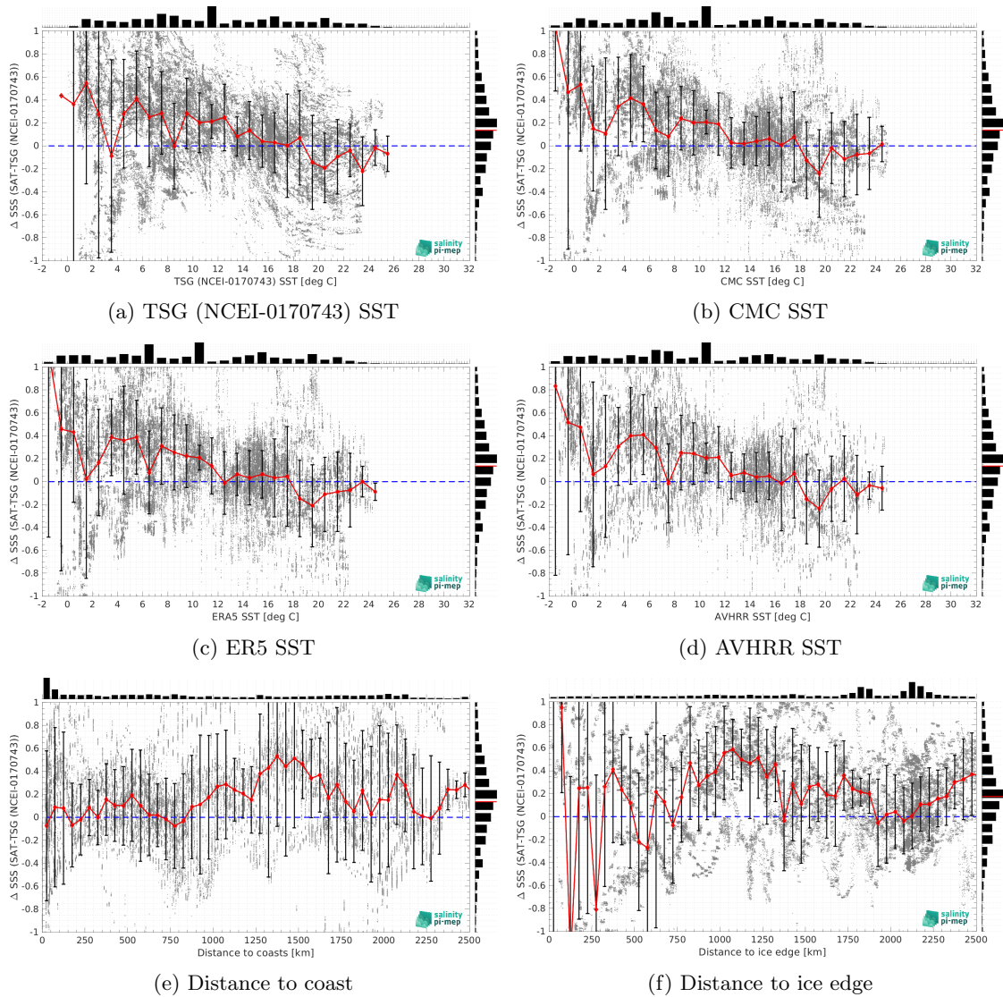
Figure 13: \Delta \text{SSS} (Satellite - TSG (NCEI-0170743)) sorted as function of TSG (NCEI-0170743) SST values (a), CMC SST (b), ERA5 SST (c), AVHRR SST (d), distance to coast (e) and distance to ice edge (f). In all plots the median and Std of \Delta \text{SSS} for each bin is indicated by the red curves and black vertical thick bars ( \pm 1 Std). Links to similar figures sorted as function of Sea ice fraction and in situ measurement depth .
