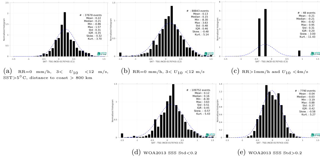
Figure 15: Normalized histogram of \Delta\text{SSS} (SMAP SSS L3 v5.0 - Monthly (JPL) - TSG (NCEI-0170743)) for 5 different subdatasets corresponding to: RR=0 mm/h, 3 < U_{10} < 12 m/s, SST > 5^\circ\text{C} , distance to coast > 800 km (a), RR=0 mm/h, 3 < U_{10} < 12 m/s (b), RR > 1 mm/h and U_{10} < 4 m/s (c), WOA2013 SSS Std < 0.2 (d), WOA2013 SSS Std > 0.2 (e).
