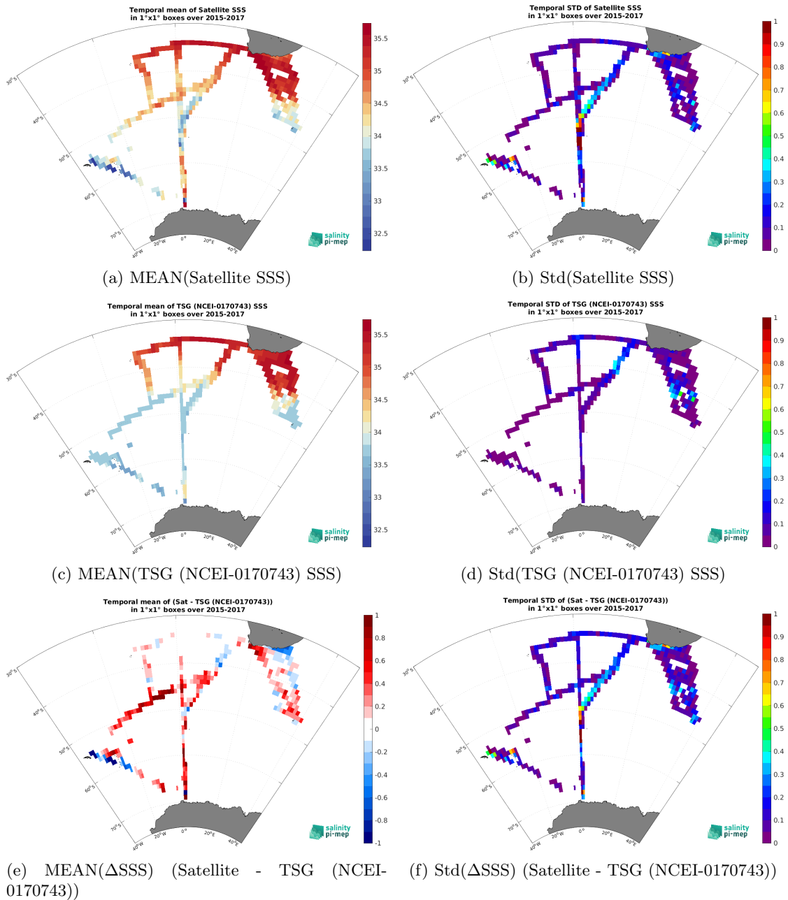
Figure 7: Temporal mean (left) and Std (right) of SSS from SMAP SSS L3 v5.0 - Monthly (JPL) (top), TSG (NCEI-0170743) (middle), and of \Delta SSS (Satellite - TSG (NCEI-0170743)). Only match-up pairs are used to generate these maps.
