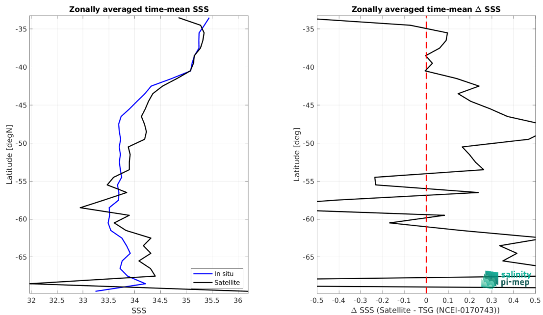
Figure 9: Left panel: Zonal mean SSS from SMAP SSS L3 v5.0 - Monthly (JPL) satellite product (black) and from TSG (NCEI-0170743) (blue). Right panel: Zonal mean of \Delta SSS (Satellite - TSG (NCEI-0170743)) for all the collected Pi-MEP match-up pairs estimated over the full satellite product period.
