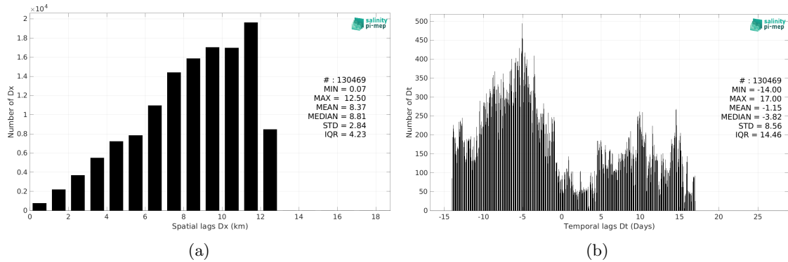
Figure 6: Histograms of the spatial (a) and temporal (b) lags between the location/time of the TSG (NCEI-0170743) measurement and the date of the corresponding SMAP SSS L3 v5.0 - Monthly (JPL) SSS pixel.
