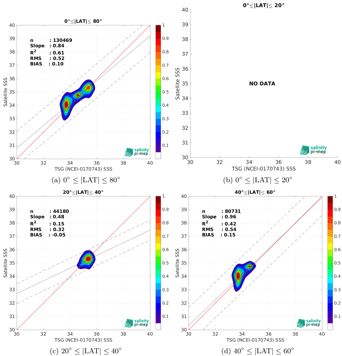
Figure 10: Contour maps of the concentration of SMAP SSS L3 v5.0 - Monthly (JPL) SSS (y-axis) versus TSG (NCEI-0170743) SSS (x-axis) at match-up pairs for different latitude bands. For each plot, the red line shows x=y . The black thin and dashed lines indicate a linear fit through the data cloud and the \pm 95\% confidence levels, respectively. The number match-up pairs n , the slope and R^2 coefficient of the linear fit, the root mean square (RMS) and the mean bias between satellite and in situ data are indicated for each latitude band in each plots.
