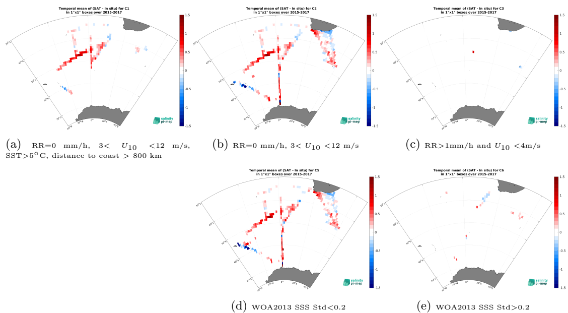
Figure 14: Temporal mean gridded over spatial boxes of size 1^\circ \times 1^\circ of \Delta SSS (SMAP SSS L3 v5.0 - Monthly (JPL) - TSG (NCEI-0170743)) for 5 different subdatasets corresponding to:RR=0 mm/h, 3 < U_{10} < 12 m/s, SST >5^\circ\text{C} , distance to coast > 800 km (a), RR=0 mm/h, 3 < U_{10} < 12 m/s (b), RR >1 mm/h and U_{10} < 4 m/s (c), WOA2013 SSS Std <0.2 (d), WOA2013 SSS Std >0.2 (e).
