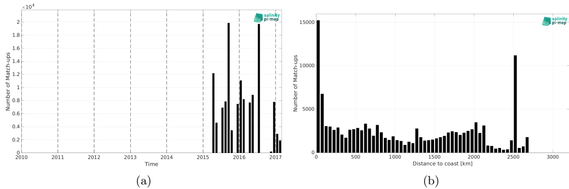
Figure 2: Number of match-ups between TSG (NCEI-0170743) and SMAP SSS L3 v5.0 - Monthly (JPL) SSS as a function of time (a) and as function of the distance to coast (b) over the Global Ocean Pi-MEP region and for the full satellite product period.
