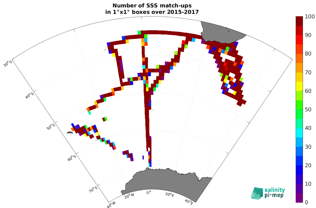
Figure 5: Number of SSS match-ups between TSG (NCEI-0170743) SSS and the SMAP SSS L3 v5.0 - Monthly (JPL) SSS product for the Global Ocean Pi-MEP region over 1^\circ \times 1^\circ boxes and for the full satellite product period.
