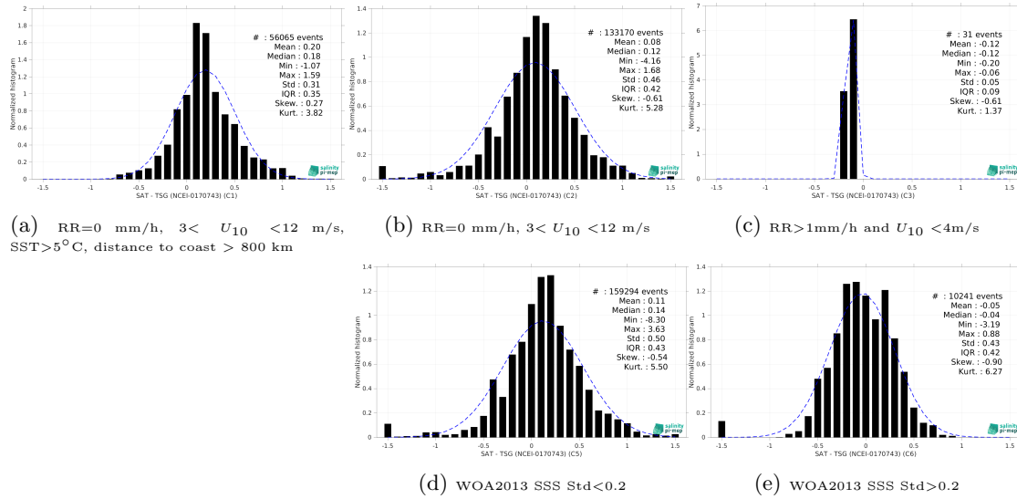
Figure 13: Normalized histogram of \Delta SSS (SMAP SSS L3 v5.0 - Monthly (JPL) - TSG (NCEI-0170743)) for 5 different subdatasets corresponding to: RR=0 mm/h, 3 < U_{10} < 12 m/s, SST>5°C, distance to coast > 800 km (a), RR=0 mm/h, 3 < U_{10} < 12 m/s (b), RR>1mm/h and U_{10} < 4 m/s (c), WOA2013 SSS Std<0.2 (d), WOA2013 SSS Std>0.2 (e).
