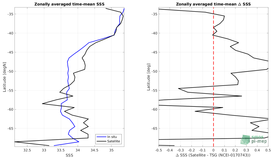
Figure 8: Left panel: Zonal mean SSS from SMAP SSS L3 v5.0 - Monthly (JPL) satellite product (black) and from TSG (NCEI-0170743) (blue). Right panel: Zonal mean of \Delta SSS (Satellite - TSG (NCEI-0170743)) for all the collected Pi-MEP match-up pairs estimated over the full satellite product period.
