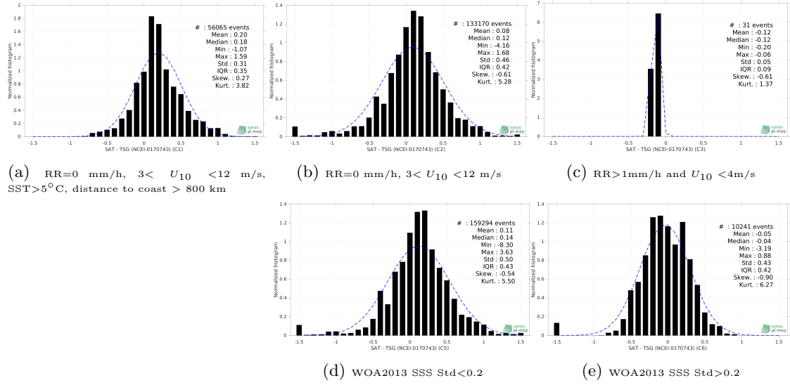
Figure 13: Normalized histogram of \Delta SSS (SMAP SSS L3 v5.0 - Monthly (JPL) - TSG (NCEI-0170743)) for 5 different subdatasets corresponding to: RR=0 mm/h, 3 < U_{10} < 12 m/s, SST > 5°C, distance to coast > 800 km (a), RR=0 mm/h, 3 < U_{10} < 12 m/s (b), RR > 1mm/h and U_{10} < 4 m/s (c), WOA2013 SSS Std < 0.2 (d), WOA2013 SSS Std > 0.2 (e).
