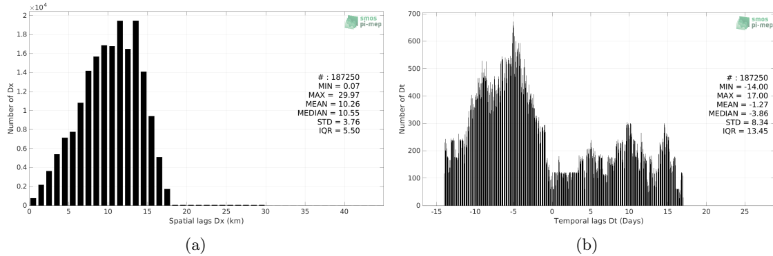
Figure 5: Histograms of the spatial (a) and temporal (b) lags between the location/time of the TSG (NCEI-0170743) measurement and the date of the corresponding SMAP SSS L3 v5.0 - Monthly (JPL) SSS pixel.
