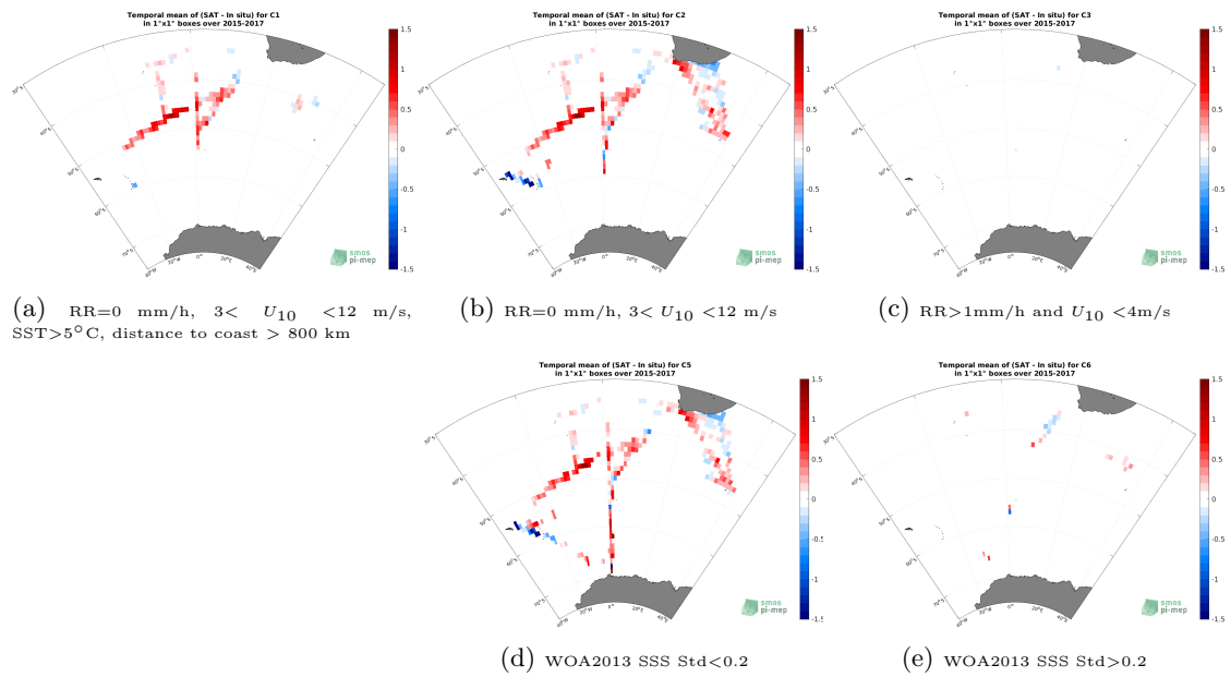
Figure 12: Temporal mean gridded over spatial boxes of size 1^\circ \times 1^\circ of \Delta SSS (SMAP SSS L3 v5.0 - Monthly (JPL) - TSG (NCEI-0170743)) for 5 different subdatasets corresponding to:RR=0 mm/h, 3 < U_{10} < 12 m/s, SST >5^\circ C, distance to coast > 800 km (a), RR=0 mm/h, 3 < U_{10} < 12 m/s (b), RR >1 mm/h and U_{10} < 4 m/s (c), WOA2013 SSS Std <0.2 (d), WOA2013 SSS Std >0.2 (e).
