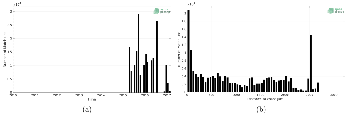
Figure 1: Number of match-ups between TSG (NCEI-0170743) and SMAP SSS L3 v5.0 - Monthly (JPL) SSS as a function of time (a) and as function of the distance to coast (b) over the Global Ocean Pi-MEP region and for the full satellite product period.
