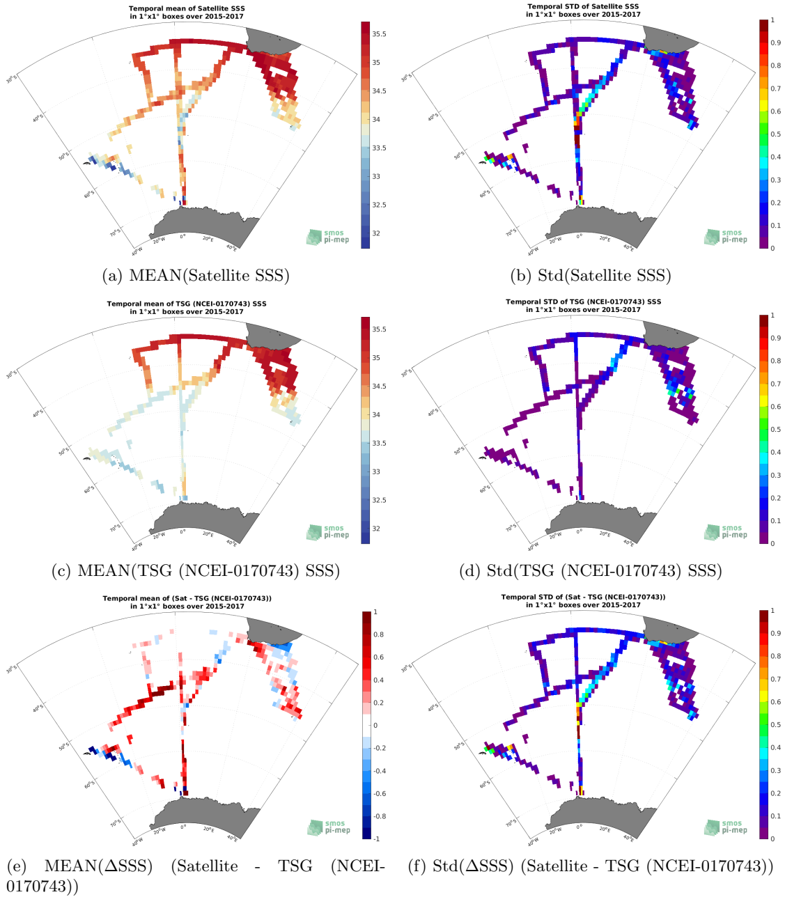
Figure 6: Temporal mean (left) and Std (right) of SSS from SMAP SSS L3 v5.0 - Monthly (JPL) (top), TSG (NCEI-0170743) (middle), and of \Delta SSS (Satellite - TSG (NCEI-0170743)). Only match-up pairs are used to generate these maps.
