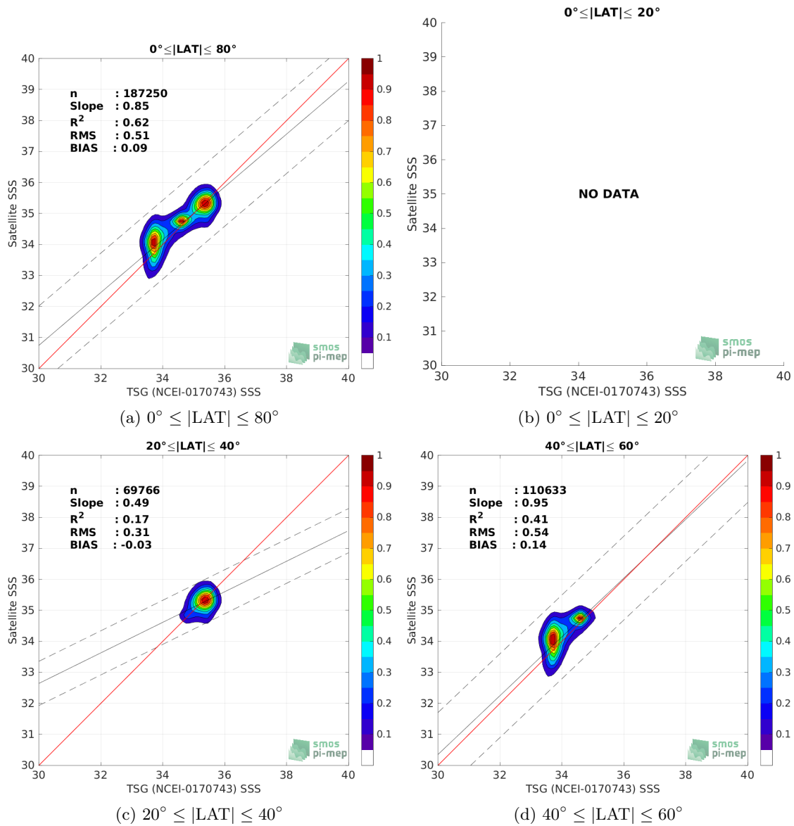
Figure 9: Contour maps of the concentration of SMAP SSS L3 v5.0 - Monthly (JPL) SSS (y-axis) versus TSG (NCEI-0170743) SSS (x-axis) at match-up pairs for different latitude bands. For each plot, the red line shows x=y . The black thin and dashed lines indicate a linear fit through the data cloud and the \pm 95\% confidence levels, respectively. The number match-up pairs n , the slope and R^2 coefficient of the linear fit, the root mean square (RMS) and the mean bias between satellite and in situ data are indicated for each latitude band in each plots.
