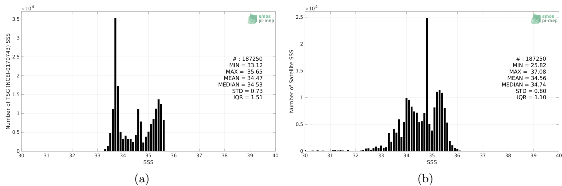
Figure 2: Histograms of SSS from TSG (NCEI-0170743) (a) and SMAP SSS L3 v5.0 - Monthly (JPL) (b) considering all match-up pairs per bins of 0.1 over the Global Ocean Pi-MEP region and for the full satellite product period.
