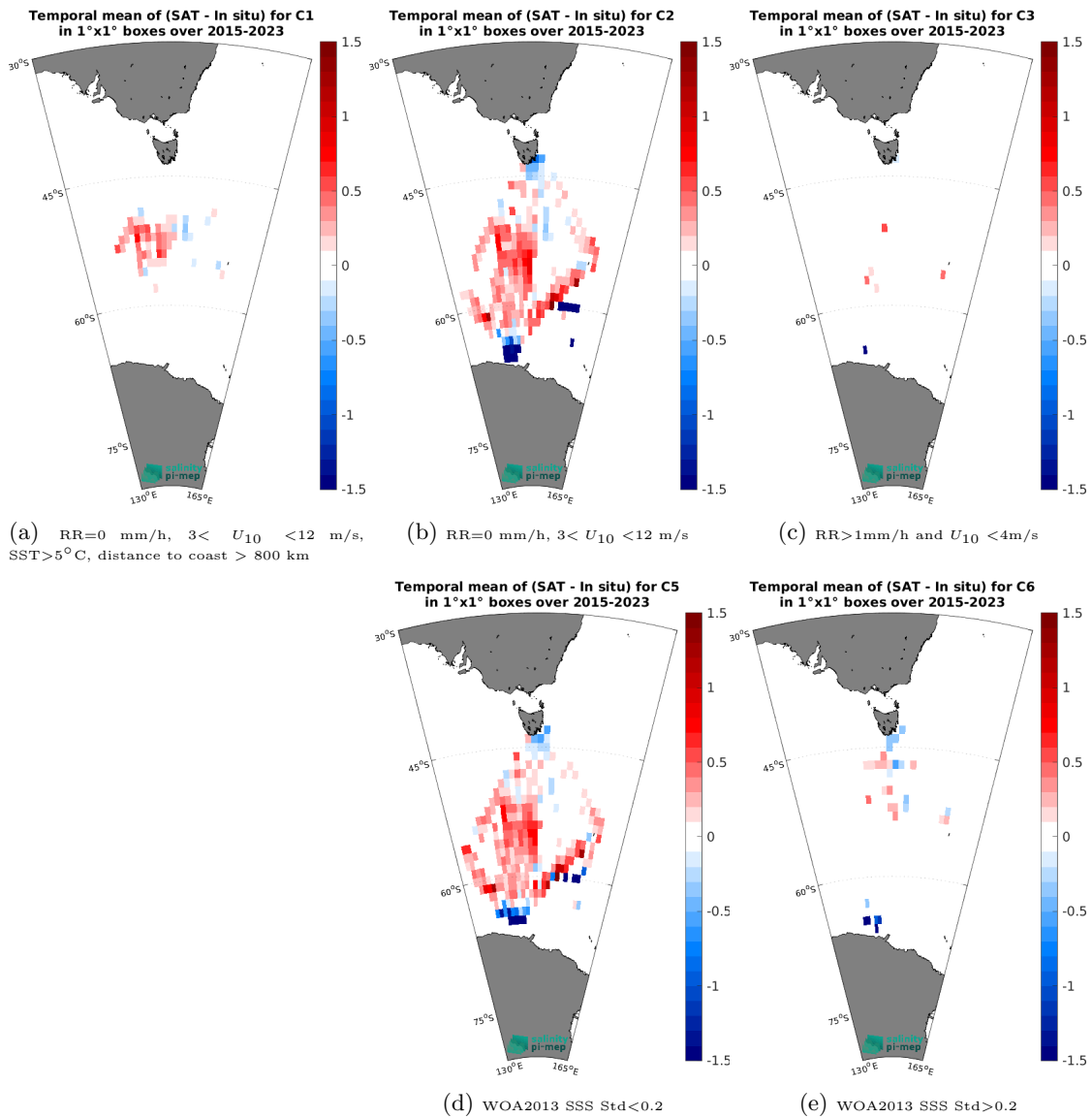
Figure 14: Temporal mean gridded over spatial boxes of size 1^\circ \times 1^\circ of \Delta\text{SSS} (SMAP SSS L3 v5.0 - Monthly (JPL) - TSG (LEGOS-Survostral)) for 5 different subdatasets corresponding to: RR=0 mm/h, 3 < U_{10} < 12 m/s, SST > 5^\circ\text{C} , distance to coast > 800 km (a), RR=0 mm/h, 3 < U_{10} < 12 m/s (b), RR > 1\text{mm/h} and U_{10} < 4\text{m/s} (c), WOA2013 SSS Std < 0.2 (d), WOA2013 SSS Std > 0.2 (e).
