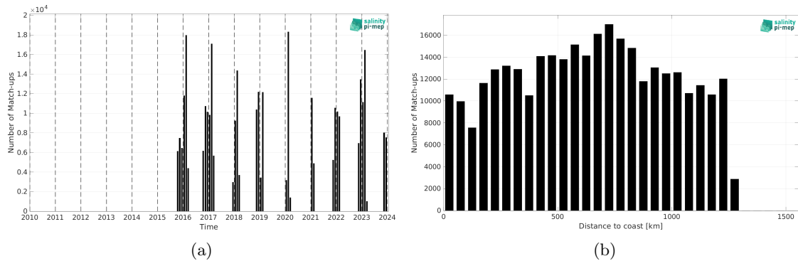
Figure 2: Number of match-ups between TSG (LEGOS-Survostral) and SMAP SSS L3 v5.0 - Monthly (JPL) SSS as a function of time (a) and as function of the distance to coast (b) over the Global Ocean Pi-MEP region and for the full satellite product period.
