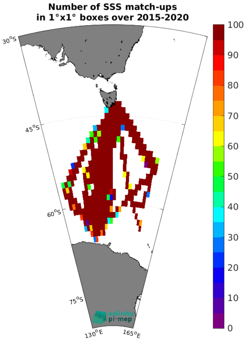
Figure 5: Number of SSS match-ups between TSG (LEGOS-Survostral) SSS and the SMAP SSS L3 v5.0 - Monthly (JPL) SSS product for the Global Ocean Pi-MEP region over 1°x1° boxes and for the full satellite product period.
