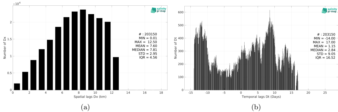
Figure 6: Histograms of the spatial (a) and temporal (b) lags between the location/time of the TSG (LEGOS-Survostral) measurement and the date of the corresponding SMAP SSS L3 v5.0 - Monthly (JPL) SSS pixel.
