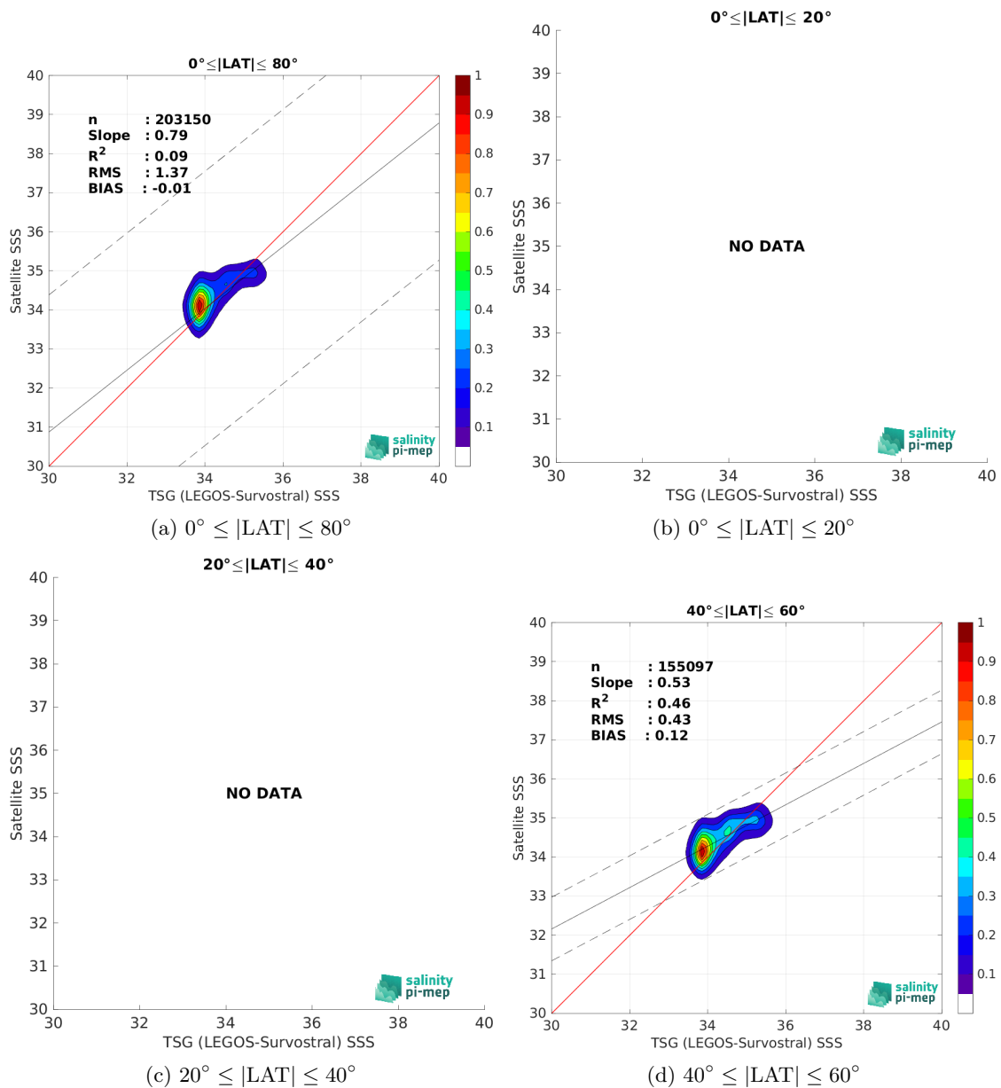
Figure 10: Contour maps of the concentration of SMAP SSS L3 v5.0 - Monthly (JPL) SSS (y-axis) versus TSG (LEGOS-Survostral) SSS (x-axis) at match-up pairs for different latitude bands. For each plot, the red line shows x=y . The black thin and dashed lines indicate a linear fit through the data cloud and the \pm 95\% confidence levels, respectively. The number match-up pairs n , the slope and R^2 coefficient of the linear fit, the root mean square (RMS) and the mean bias between satellite and in situ data are indicated for each latitude band in each plots.
