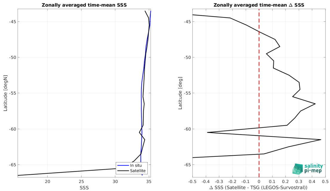
Figure 9: Left panel: Zonal mean SSS from SMAP SSS L3 v5.0 - Monthly (JPL) satellite product (black) and from TSG (LEGOS-Survostral) (blue). Right panel: Zonal mean of \Delta SSS (Satellite - TSG (LEGOS-Survostral)) for all the collected Pi-MEP match-up pairs estimated over the full satellite product period.
