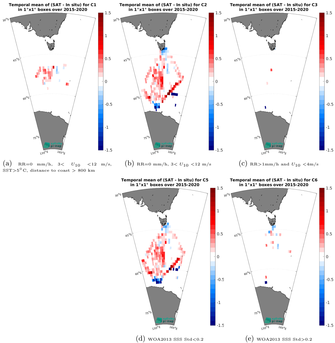
Figure 14: Temporal mean gridded over spatial boxes of size 1^\circ \times 1^\circ of \Delta SSS (SMAP SSS L3 v5.0 - Monthly (JPL) - TSG (LEGOS-Survostral)) for 5 different subdatasets corresponding to: RR=0 mm/h, 3 < U_{10} < 12 m/s, SST > 5°C, distance to coast > 800 km (a), RR=0 mm/h, 3 < U_{10} < 12 m/s (b), RR > 1mm/h and U_{10} < 4 m/s (c), WOA2013 SSS Std < 0.2 (d), WOA2013 SSS Std > 0.2 (e).
