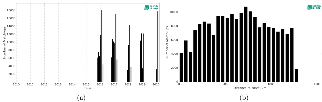
Figure 2: Number of match-ups between TSG (LEGOS-Survostral) and SMAP SSS L3 v5.0 - Monthly (JPL) SSS as a function of time (a) and as function of the distance to coast (b) over the Global Ocean Pi-MEP region and for the full satellite product period.
