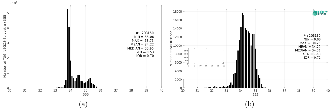
Figure 3: Histograms of SSS from TSG (LEGOS-Survostral) (a) and SMAP SSS L3 v5.0 - Monthly (JPL) (b) considering all match-up pairs per bins of 0.1 over the Global Ocean Pi-MEP region and for the full satellite product period.
