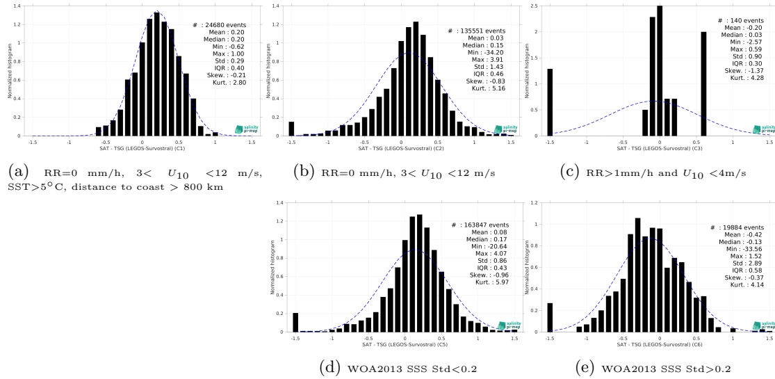
Figure 15: Normalized histogram of \Delta SSS (SMAP SSS L3 v5.0 - Monthly (JPL) - TSG (LEGOS-Survostral)) for 5 different subdatasets corresponding to: RR=0 mm/h, 3 < U_{10} < 12 m/s, SST>5°C, distance to coast > 800 km (a), RR=0 mm/h, 3 < U_{10} < 12 m/s (b), RR>1mm/h and U_{10} < 4 m/s (c), WOA2013 SSS Std<0.2 (d), WOA2013 SSS Std>0.2 (e).
