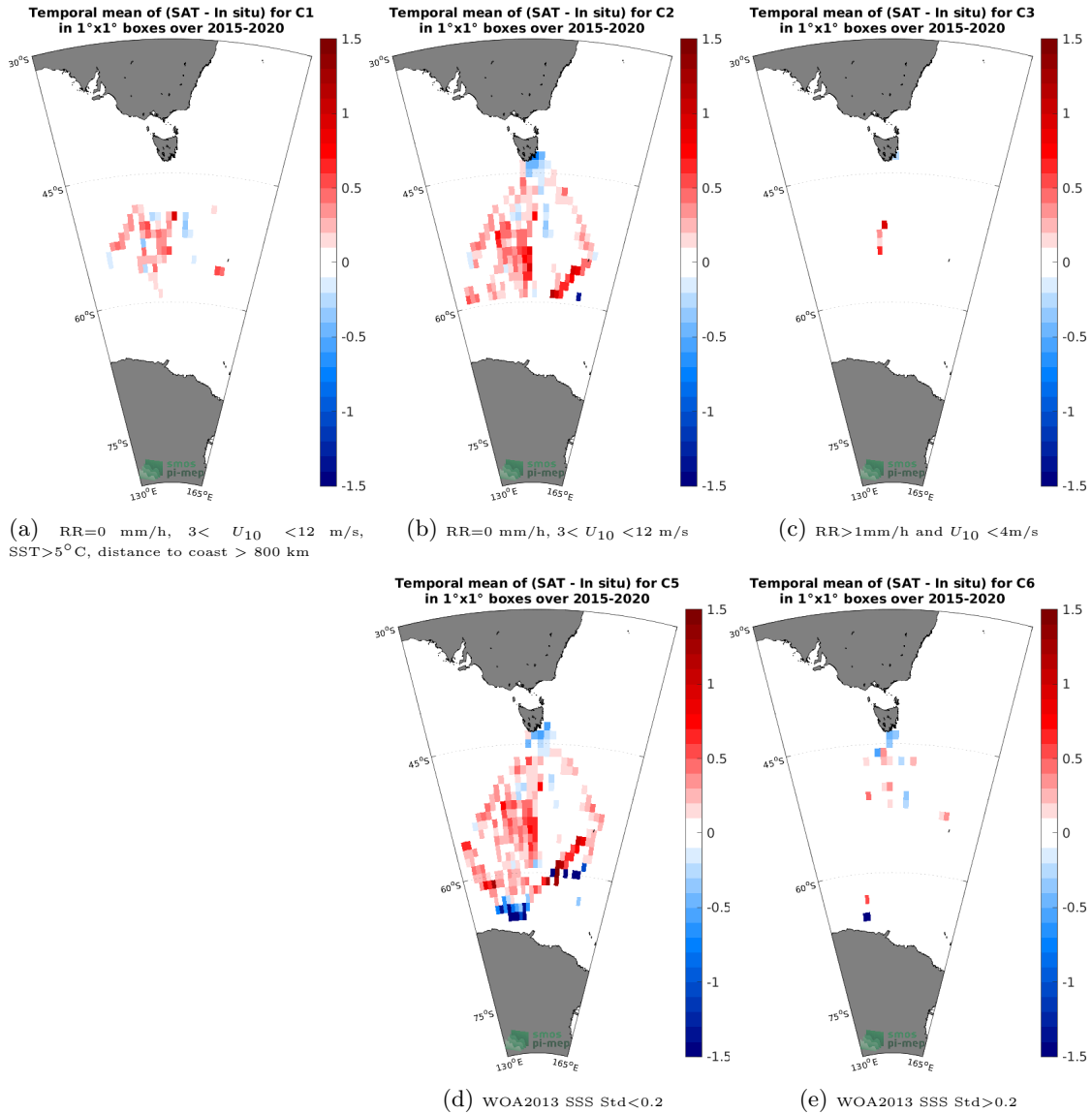
Figure 12: Temporal mean gridded over spatial boxes of size 1^\circ \times 1^\circ of \Delta SSS (SMAP SSS L3 v5.0 - Monthly (JPL) - TSG (LEGOS-Survostral)) for 5 different subdatasets corresponding to:RR=0 mm/h, 3 < U_{10} < 12 m/s, SST>5°C, distance to coast > 800 km (a), RR=0 mm/h, 3 < U_{10} < 12 m/s (b), RR>1mm/h and U_{10} < 4 m/s (c), WOA2013 SSS Std<0.2 (d), WOA2013 SSS Std>0.2 (e).
