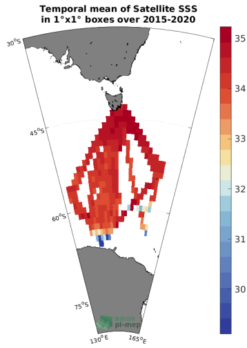
(a) MEAN(Satellite SSS)
