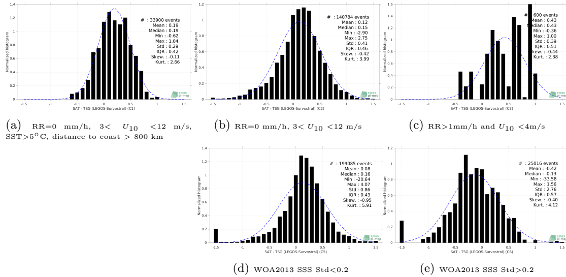
Figure 13: Normalized histogram of \Delta SSS (SMAP SSS L3 v5.0 - Monthly (JPL) - TSG (LEGOS-Survostral)) for 5 different subdatasets corresponding to: RR=0 mm/h, 3 < U_{10} < 12 m/s, SST > 5°C, distance to coast > 800 km (a), RR=0 mm/h, 3 < U_{10} < 12 m/s (b), RR > 1mm/h and U_{10} < 4 m/s (c), WOA2013 SSS Std < 0.2 (d), WOA2013 SSS Std > 0.2 (e).
