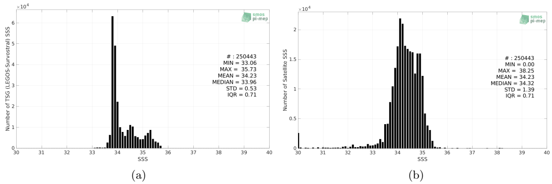
Figure 2: Histograms of SSS from TSG (LEGOS-Survostral) (a) and SMAP SSS L3 v5.0 - Monthly (JPL) (b) considering all match-up pairs per bins of 0.1 over the Global Ocean Pi-MEP region and for the full satellite product period.
