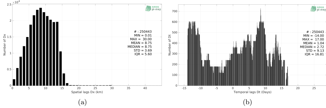
Figure 5: Histograms of the spatial (a) and temporal (b) lags between the location/time of the TSG (LEGOS-Survostral) measurement and the date of the corresponding SMAP SSS L3 v5.0 - Monthly (JPL) SSS pixel.
