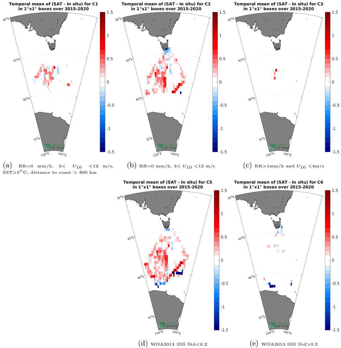
Figure 12: Temporal mean gridded over spatial boxes of size 1^\circ \times 1^\circ of \Delta\text{SSS} (SMAP SSS L3 v5.0 - Monthly (JPL) - TSG (LEGOS-Survostral)) for 5 different subdatasets corresponding to: RR=0 mm/h, 3 < U_{10} < 12 m/s, SST > 5^\circ\text{C} , distance to coast > 800 km (a), RR=0 mm/h, 3 < U_{10} < 12 m/s (b), RR > 1\text{mm/h} and U_{10} < 4\text{m/s} (c), WOA2013 SSS Std < 0.2 (d), WOA2013 SSS Std > 0.2 (e).
