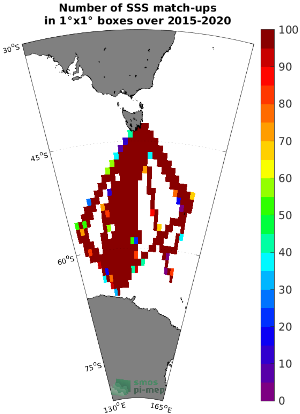
Figure 4: Number of SSS match-ups between TSG (LEGOS-Survostral) SSS and the SMAP SSS L3 v5.0 - Monthly (JPL) SSS product for the Global Ocean Pi-MEP region over 1°x1° boxes and for the full satellite product period.
