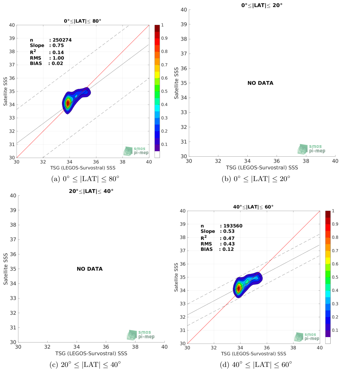
Figure 9: Contour maps of the concentration of SMAP SSS L3 v5.0 - Monthly (JPL) SSS (y-axis) versus TSG (LEGOS-Survostral) SSS (x-axis) at match-up pairs for different latitude bands. For each plot, the red line shows x=y . The black thin and dashed lines indicate a linear fit through the data cloud and the \pm 95\% confidence levels, respectively. The number match-up pairs n , the slope and R^2 coefficient of the linear fit, the root mean square (RMS) and the mean bias between satellite and in situ data are indicated for each latitude band in each plots.
