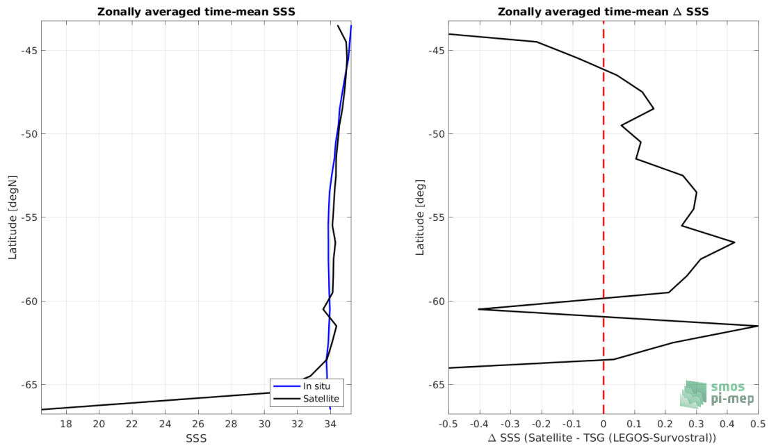
Figure 8: Left panel: Zonal mean SSS from SMAP SSS L3 v5.0 - Monthly (JPL) satellite product (black) and from TSG (LEGOS-Survostral) (blue). Right panel: Zonal mean of \Delta SSS (Satellite - TSG (LEGOS-Survostral)) for all the collected Pi-MEP match-up pairs estimated over the full satellite product period.
