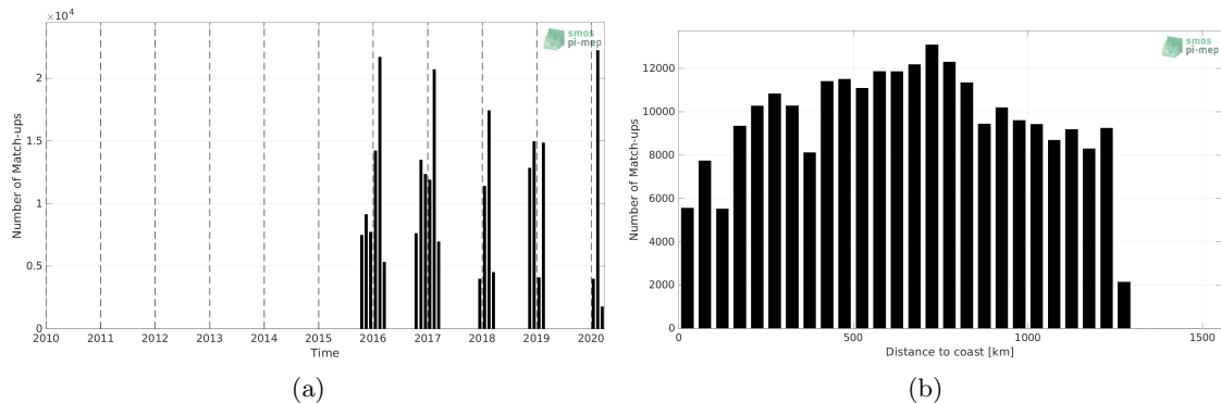
Figure 1: Number of match-ups between TSG (LEGOS-Survostral) and SMAP SSS L3 v5.0 - Monthly (JPL) SSS as a function of time (a) and as function of the distance to coast (b) over the Global Ocean Pi-MEP region and for the full satellite product period.
