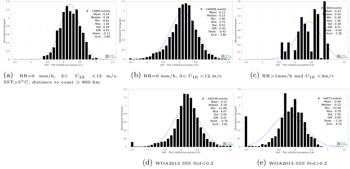
Figure 13: Normalized histogram of \Delta SSS (SMAP SSS L3 v5.0 - Monthly (JPL) - TSG (LEGOS-Survostral)) for 5 different subdatasets corresponding to: RR=0 mm/h, 3 < U_{10} < 12 m/s, SST > 5°C, distance to coast > 800 km (a), RR=0 mm/h, 3 < U_{10} < 12 m/s (b), RR > 1mm/h and U_{10} < 4 m/s (c), WOA2013 SSS Std < 0.2 (d), WOA2013 SSS Std > 0.2 (e).
