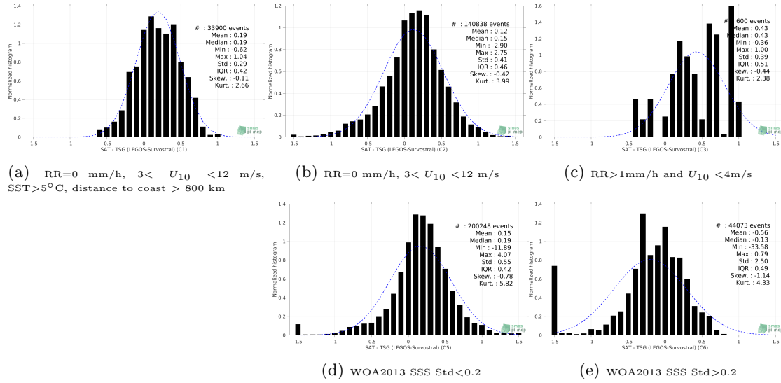
Figure 13: Normalized histogram of \Delta SSS (SMAP SSS L3 v5.0 - Monthly (JPL) - TSG (LEGOS-Survostral)) for 5 different subdatasets corresponding to: RR=0 mm/h, 3 < U_{10} < 12 m/s, SST>5°C, distance to coast > 800 km (a), RR=0 mm/h, 3 < U_{10} < 12 m/s (b), RR>1mm/h and U_{10} < 4 m/s (c), WOA2013 SSS Std<0.2 (d), WOA2013 SSS Std>0.2 (e).
