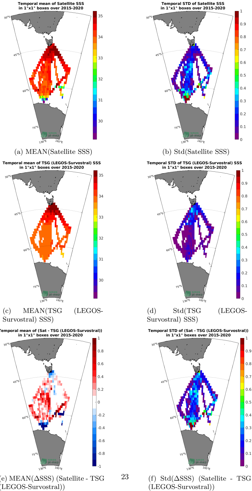
Figure 6: Temporal mean (left) and Std (right) of SSS from SMAP SSS L3 v5.0 - Monthly (JPL) (top), TSG (LEGOS-Survostral) (middle), and of \Delta SSS (Satellite - TSG (LEGOS-Survostral)). Only match-up pairs are used to generate these maps.
