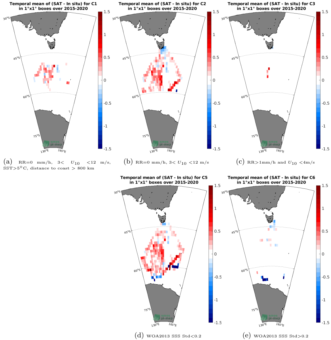
Figure 12: Temporal mean gridded over spatial boxes of size 1^\circ \times 1^\circ of \Delta\text{SSS} (SMAP SSS L3 v5.0 - Monthly (JPL) - TSG (LEGOS-Survostral)) for 5 different subdatasets corresponding to: RR=0 mm/h, 3 < U_{10} < 12 m/s, SST > 5^\circ\text{C} , distance to coast > 800 km (a), RR=0 mm/h, 3 < U_{10} < 12 m/s (b), RR > 1 mm/h and U_{10} < 4 m/s (c), WOA2013 SSS Std < 0.2 (d), WOA2013 SSS Std > 0.2 (e).
