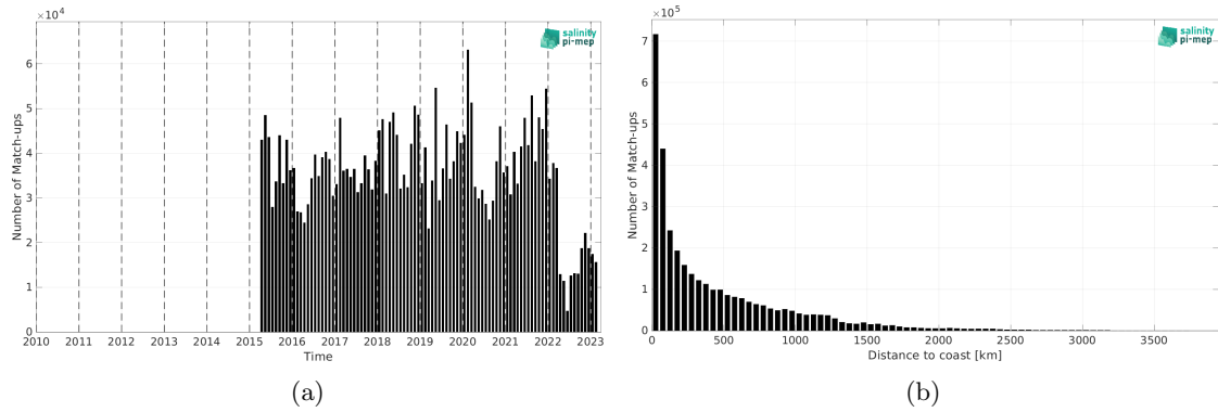
Figure 2: Number of match-ups between TSG (LEGOS-DM) and SMAP SSS L3 v5.0 - Monthly (JPL) SSS as a function of time (a) and as function of the distance to coast (b) over the Global Ocean Pi-MEP region and for the full satellite product period.
