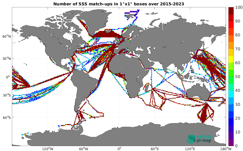
Figure 5: Number of SSS match-ups between TSG (LEGOS-DM) SSS and the SMAP SSS L3 v5.0 - Monthly (JPL) SSS product for the Global Ocean Pi-MEP region over 1^\circ \times 1^\circ boxes and for the full satellite product period.
