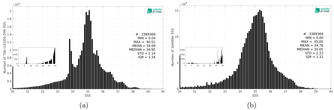
Figure 3: Histograms of SSS from TSG (LEGOS-DM) (a) and SMAP SSS L3 v5.0 - Monthly (JPL) (b) considering all match-up pairs per bins of 0.1 over the Global Ocean Pi-MEP region and for the full satellite product period.
