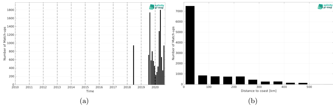
Figure 2: Number of match-ups between TSG (Lauge-Koch) and SMAP SSS L3 v5.0 - Monthly (JPL) SSS as a function of time (a) and as function of the distance to coast (b) over the Global Ocean Pi-MEP region and for the full satellite product period.
