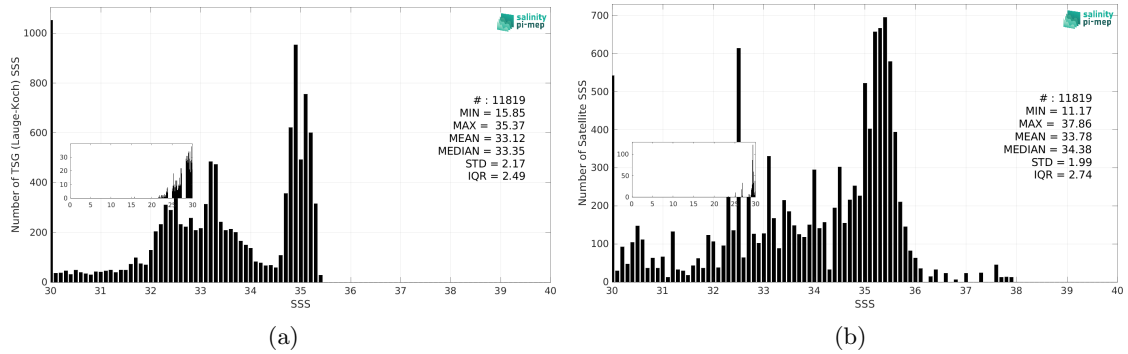
Figure 3: Histograms of SSS from TSG (Lauge-Koch) (a) and SMAP SSS L3 v5.0 - Monthly (JPL) (b) considering all match-up pairs per bins of 0.1 over the Global Ocean Pi-MEP region and for the full satellite product period.
