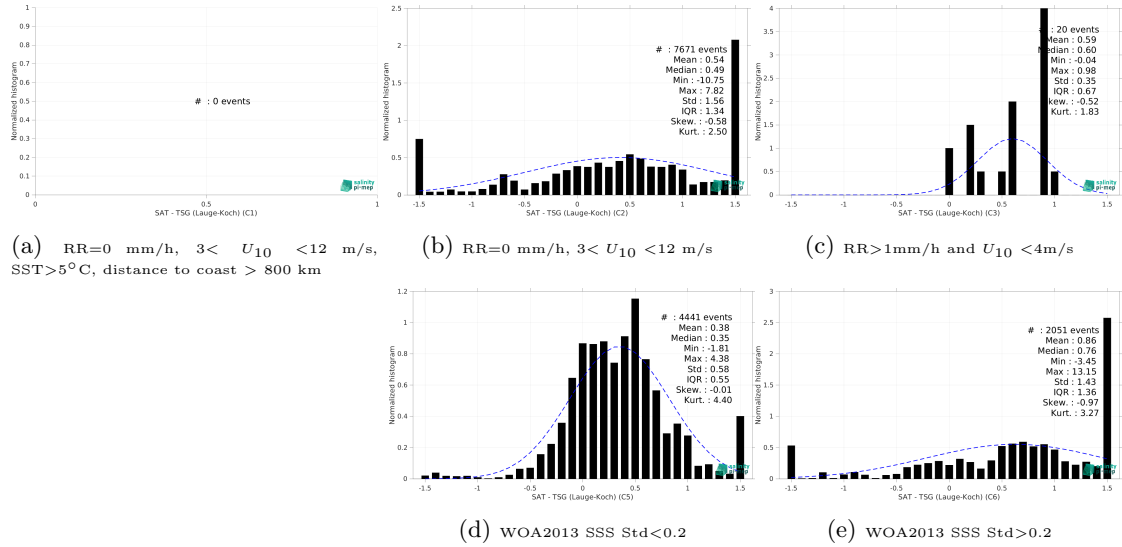
Figure 15: Normalized histogram of \Delta SSS (SMAP SSS L3 v5.0 - Monthly (JPL) - TSG (Lauge-Koch)) for 5 different subdatasets corresponding to: RR=0 mm/h, 3 < U_{10} < 12 m/s, SST > 5°C, distance to coast > 800 km (a), RR=0 mm/h, 3 < U_{10} < 12 m/s (b), RR > 1mm/h and U_{10} < 4 m/s (c), WOA2013 SSS Std < 0.2 (d), WOA2013 SSS Std > 0.2 (e).
