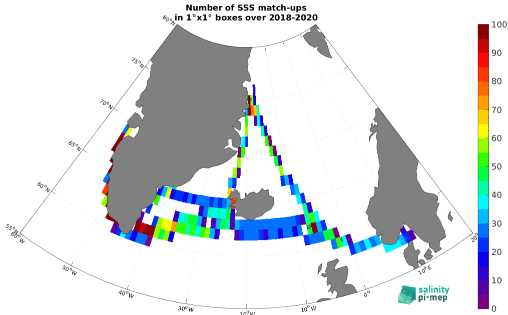
Figure 5: Number of SSS match-ups between TSG (Lauge-Koch) SSS and the SMAP SSS L3 v5.0 - Monthly (JPL) SSS product for the Global Ocean Pi-MEP region over 1^\circ \times 1^\circ boxes and for the full satellite product period.
