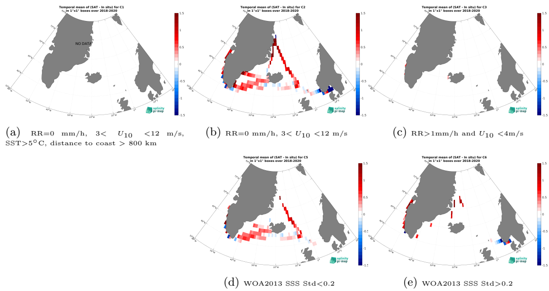
Figure 14: Temporal mean gridded over spatial boxes of size 1^\circ \times 1^\circ of \Delta SSS (SMAP SSS L3 v5.0 - Monthly (JPL) - TSG (Lauge-Koch)) for 5 different subdatasets corresponding to: RR=0 mm/h, 3 < U_{10} < 12 m/s, SST > 5^\circ\text{C} , distance to coast > 800 km (a), RR=0 mm/h, 3 < U_{10} < 12 m/s (b), RR > 1 mm/h and U_{10} < 4 m/s (c), WOA2013 SSS Std < 0.2 (d), WOA2013 SSS Std > 0.2 (e).
