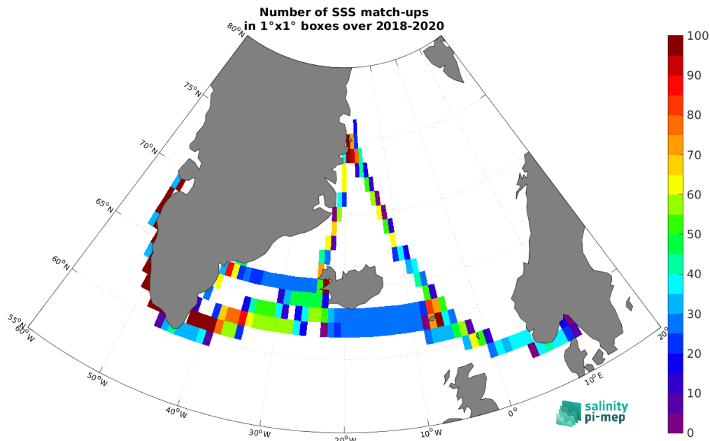
Figure 4: Number of SSS match-ups between TSG (Lauge-Koch) SSS and the SMAP SSS L3 v5.0 - Monthly (JPL) SSS product for the Global Ocean Pi-MEP region over 1^\circ \times 1^\circ boxes and for the full satellite product period.
