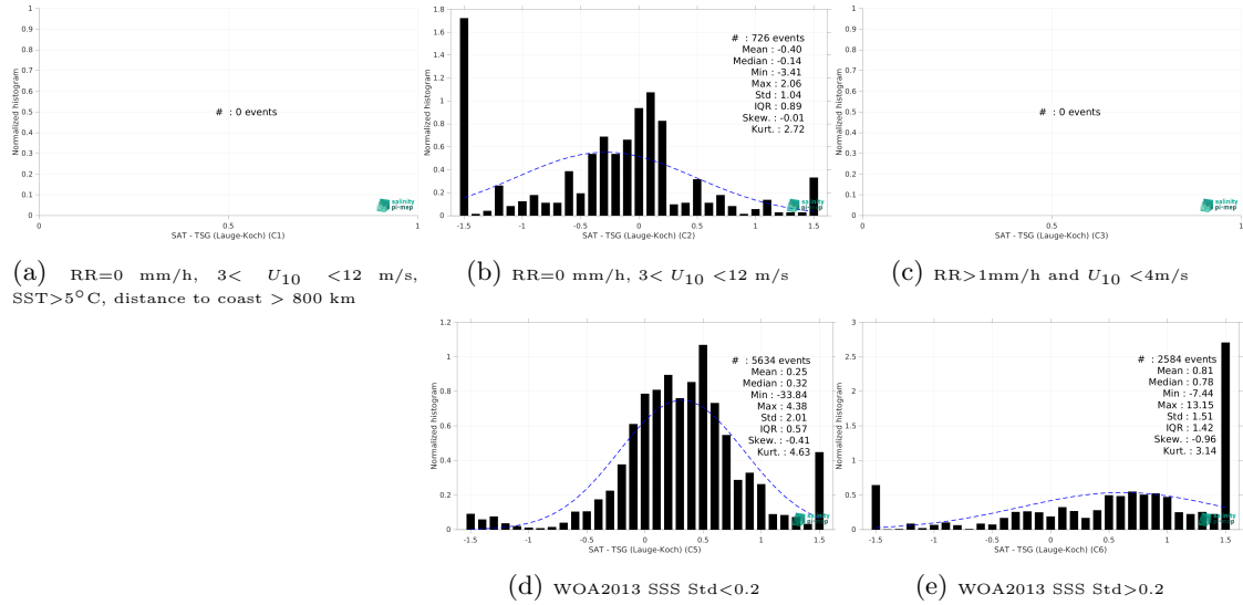
Figure 13: Normalized histogram of \Delta SSS (SMAP SSS L3 v5.0 - Monthly (JPL) - TSG (Lauge-Koch)) for 5 different subdatasets corresponding to: RR=0 mm/h, 3 < U_{10} < 12 m/s, SST > 5°C, distance to coast > 800 km (a), RR=0 mm/h, 3 < U_{10} < 12 m/s (b), RR > 1mm/h and U_{10} < 4 m/s (c), WOA2013 SSS Std < 0.2 (d), WOA2013 SSS Std > 0.2 (e).
