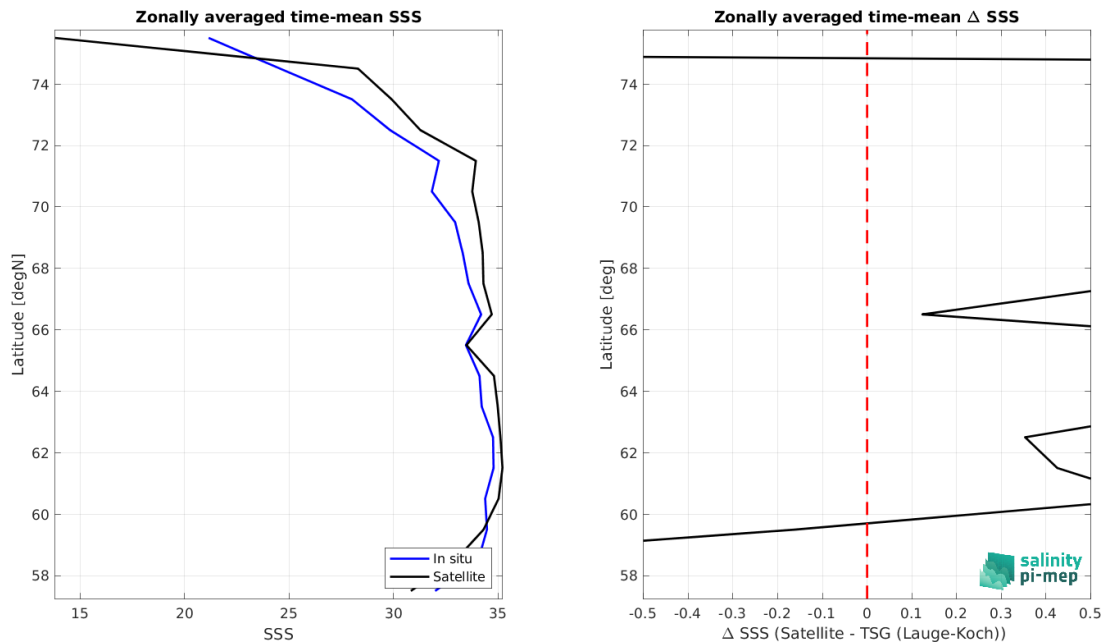
Figure 8: Left panel: Zonal mean SSS from SMAP SSS L3 v5.0 - Monthly (JPL) satellite product (black) and from TSG (Lauge-Koch) (blue). Right panel: Zonal mean of \Delta SSS (Satellite - TSG (Lauge-Koch)) for all the collected Pi-MEP match-up pairs estimated over the full satellite product period.
