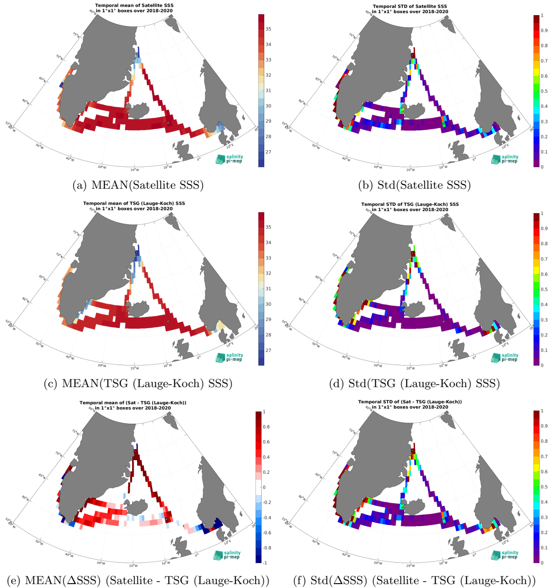
Figure 6: Temporal mean (left) and Std (right) of SSS from SMAP SSS L3 v5.0 - Monthly (JPL) (top), TSG (Lauge-Koch) (middle), and of \Delta SSS (Satellite - TSG (Lauge-Koch)). Only match-up pairs are used to generate these maps.
