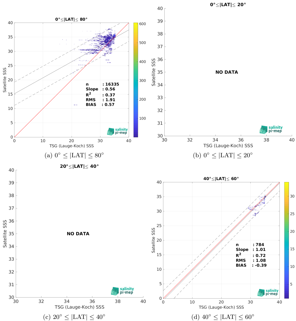
Figure 9: Contour maps of the concentration of SMAP SSS L3 v5.0 - Monthly (JPL) SSS (y-axis) versus TSG (Lauge-Koch) SSS (x-axis) at match-up pairs for different latitude bands. For each plot, the red line shows x=y . The black thin and dashed lines indicate a linear fit through the data cloud and the \pm 95\% confidence levels, respectively. The number match-up pairs n , the slope and R^2 coefficient of the linear fit, the root mean square (RMS) and the mean bias between satellite and in situ data are indicated for each latitude band in each plots.
