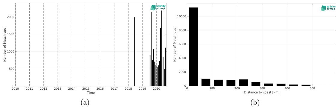
Figure 1: Number of match-ups between TSG (Lauge-Koch) and SMAP SSS L3 v5.0 - Monthly (JPL) SSS as a function of time (a) and as function of the distance to coast (b) over the Global Ocean Pi-MEP region and for the full satellite product period.
