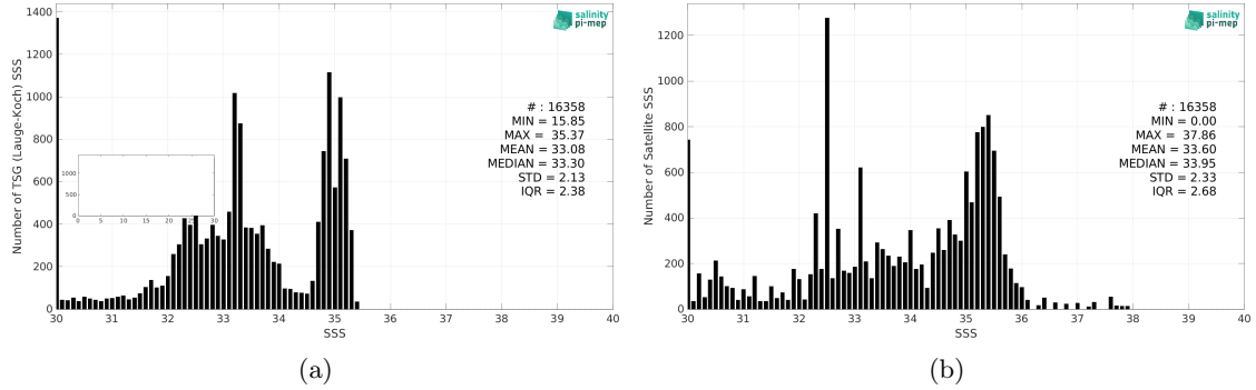
Figure 2: Histograms of SSS from TSG (Lauge-Koch) (a) and SMAP SSS L3 v5.0 - Monthly (JPL) (b) considering all match-up pairs per bins of 0.1 over the Global Ocean Pi-MEP region and for the full satellite product period.
