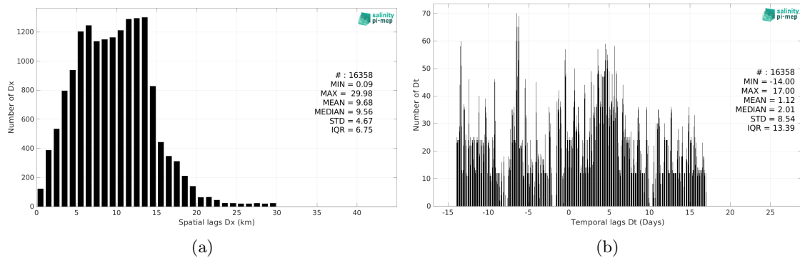
Figure 5: Histograms of the spatial (a) and temporal (b) lags between the location/time of the TSG (Lauge-Koch) measurement and the date of the corresponding SMAP SSS L3 v5.0 - Monthly (JPL) SSS pixel.
