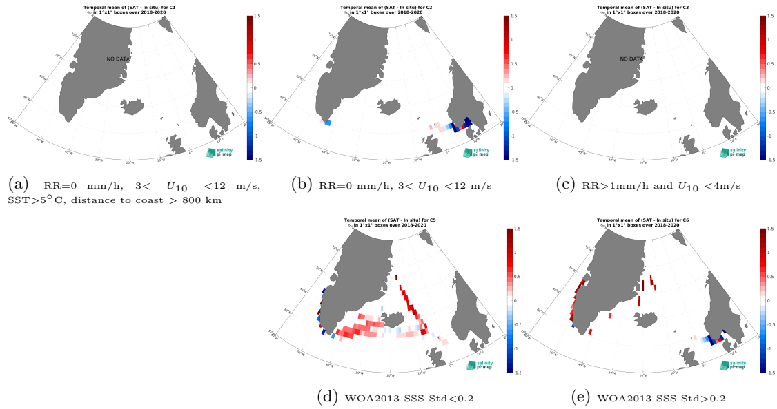
Figure 12: Temporal mean gridded over spatial boxes of size 1^{\circ}\times 1^{\circ} of \Delta\text{SSS} (SMAP SSS L3 v5.0 - Monthly (JPL) - TSG (Lauge-Koch)) for 5 different subdatasets corresponding to:RR=0 mm/h, 3 < U_{10} < 12 m/s, SST > 5^{\circ}\text{C} , distance to coast > 800 km (a), RR=0 mm/h, 3 < U_{10} < 12 m/s (b), RR > 1 mm/h and U_{10} < 4 m/s (c), WOA2013 SSS Std < 0.2 (d), WOA2013 SSS Std > 0.2 (e).
