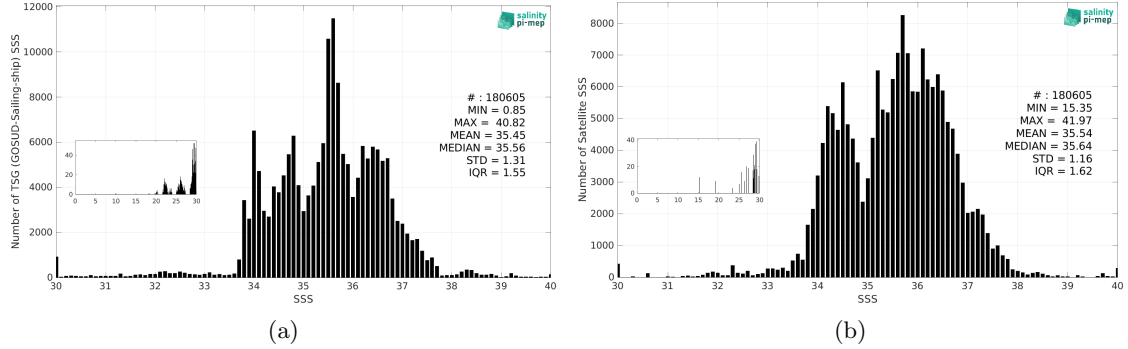
Figure 3: Histograms of SSS from TSG (GOSUD-Sailing-ship) (a) and SMAP SSS L3 v5.0 - Monthly (JPL) (b) considering all match-up pairs per bins of 0.1 over the Global Ocean Pi-MEP region and for the full satellite product period.
