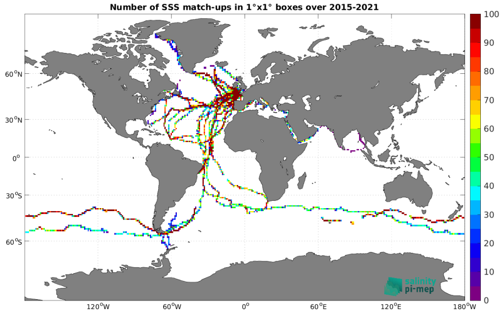
Figure 5: Number of SSS match-ups between TSG (GOSUD-Sailing-ship) SSS and the SMAP SSS L3 v5.0 - Monthly (JPL) SSS product for the Global Ocean Pi-MEP region over 1^\circ \times 1^\circ boxes and for the full satellite product period.
