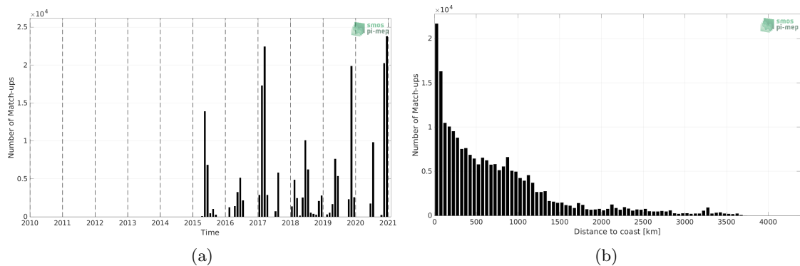
Figure 1: Number of match-ups between TSG (GOSUD-Sailing-ship) and SMAP SSS L3 v5.0 - Monthly (JPL) SSS as a function of time (a) and as function of the distance to coast (b) over the Global Ocean Pi-MEP region and for the full satellite product period.
