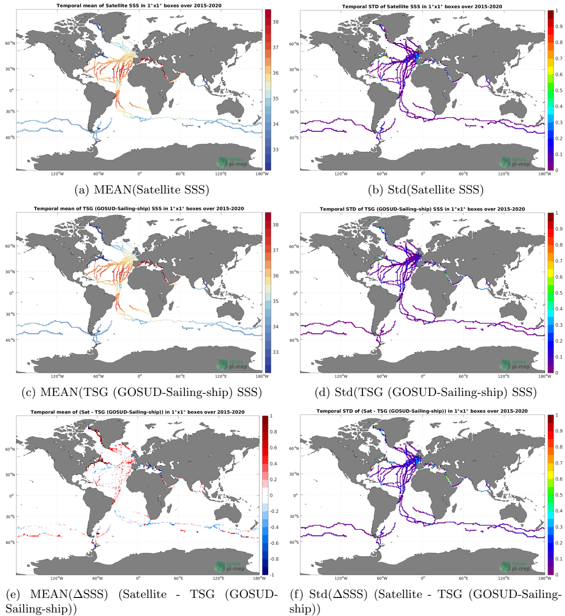
Figure 6: Temporal mean (left) and Std (right) of SSS from SMAP SSS L3 v5.0 - Monthly (JPL) (top), TSG (GOSUD-Sailing-ship) (middle), and of \Delta SSS (Satellite - TSG (GOSUD-Sailing-ship)). Only match-up pairs are used to generate these maps.
