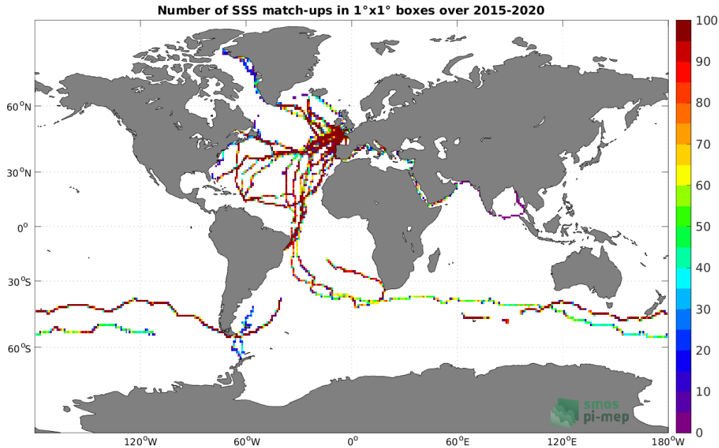
Figure 4: Number of SSS match-ups between TSG (GOSUD-Sailing-ship) SSS and the SMAP SSS L3 v5.0 - Monthly (JPL) SSS product for the Global Ocean Pi-MEP region over 1^\circ \times 1^\circ boxes and for the full satellite product period.
