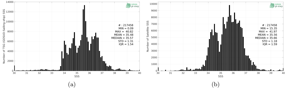
Figure 2: Histograms of SSS from TSG (GOSUD-Sailing-ship) (a) and SMAP SSS L3 v5.0 - Monthly (JPL) (b) considering all match-up pairs per bins of 0.1 over the Global Ocean Pi-MEP region and for the full satellite product period.
