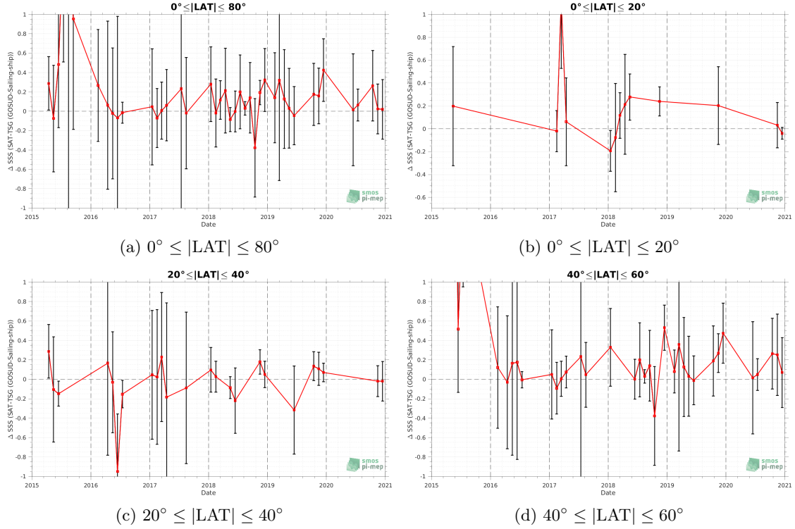
Figure 10: Monthly median (red curves) of \Delta \text{SSS} (Satellite - TSG (GOSUD-Sailing-ship)) and \pm 1 Std (black vertical thick bars) as function of time for all the collected Pi-MEP match-up pairs estimated over the Global Ocean Pi-MEP region and for the full satellite product period are shown for different latitude bands: (a) 80°S-80°N, (b) 20°S-20°N, (c) 40°S-20°S and 20°N-40°N and (d) 60°S-40°S and 40°N-60°N.
