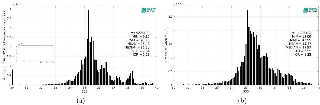
Figure 2: Histograms of SSS from TSG (GOSUD-Research-vessel) (a) and SMAP SSS L3 v5.0 - Monthly (JPL) (b) considering all match-up pairs per bins of 0.1 over the Global Ocean Pi-MEP region and for the full satellite product period.
