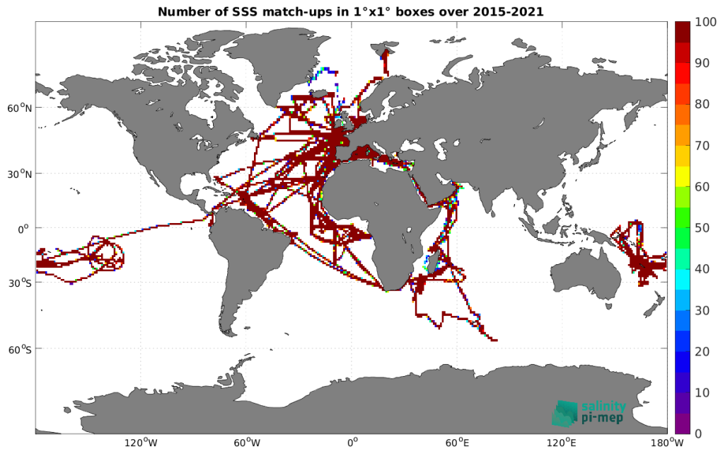
Figure 4: Number of SSS match-ups between TSG (GOSUD-Research-vessel) SSS and the SMAP SSS L3 v5.0 - Monthly (JPL) SSS product for the Global Ocean Pi-MEP region over 1^\circ \times 1^\circ boxes and for the full satellite product period.
