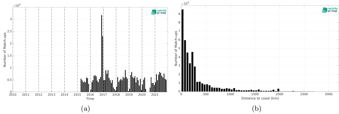
Figure 1: Number of match-ups between TSG (GOSUD-Research-vessel) and SMAP SSS L3 v5.0 - Monthly (JPL) SSS as a function of time (a) and as function of the distance to coast (b) over the Global Ocean Pi-MEP region and for the full satellite product period.
