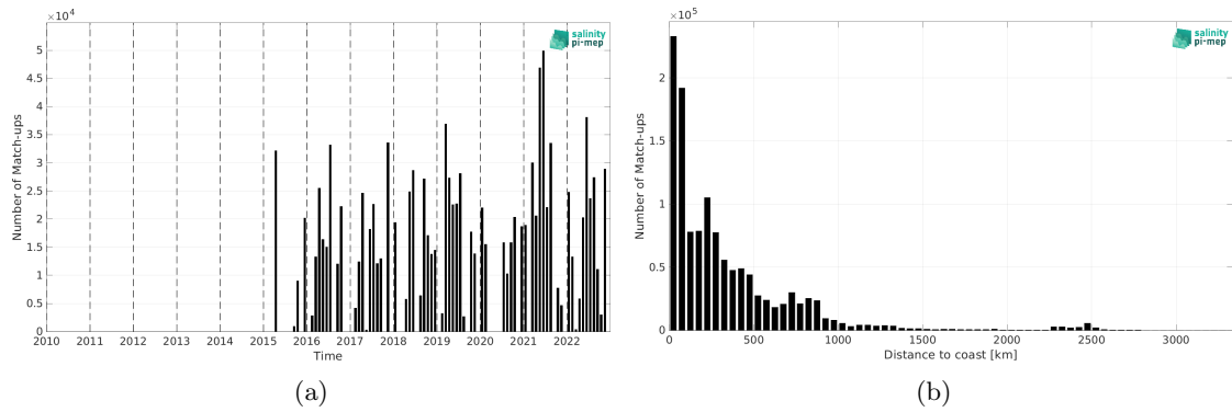
Figure 1: Number of match-ups between TSG (CSIC-UTM) and SMAP SSS L3 v5.0 - Monthly (JPL) SSS as a function of time (a) and as function of the distance to coast (b) over the Global Ocean Pi-MEP region and for the full satellite product period.
