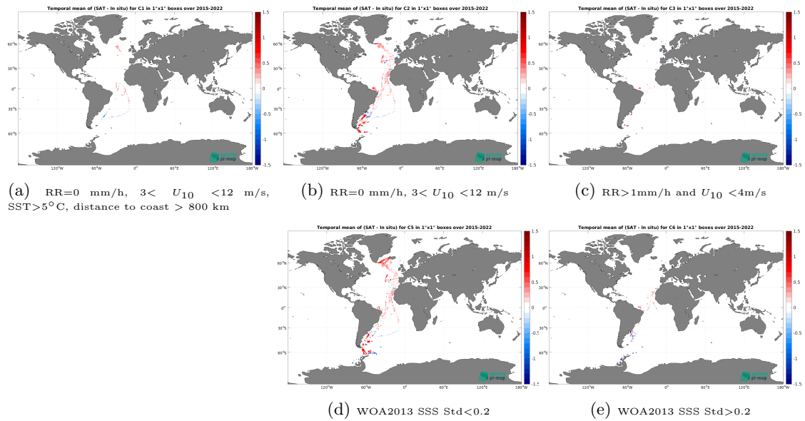
Figure 12: Temporal mean gridded over spatial boxes of size 1^\circ \times 1^\circ of \Delta SSS (SMAP SSS L3 v5.0 - Monthly (JPL) - TSG (CSIC-UTM)) for 5 different subdatasets corresponding to:RR=0 mm/h, 3 < U_{10} < 12 m/s, SST > 5^\circ\text{C} , distance to coast > 800 km (a), RR=0 mm/h, 3 < U_{10} < 12 m/s (b), RR > 1 mm/h and U_{10} < 4 m/s (c), WOA2013 SSS Std < 0.2 (d), WOA2013 SSS Std > 0.2 (e).
