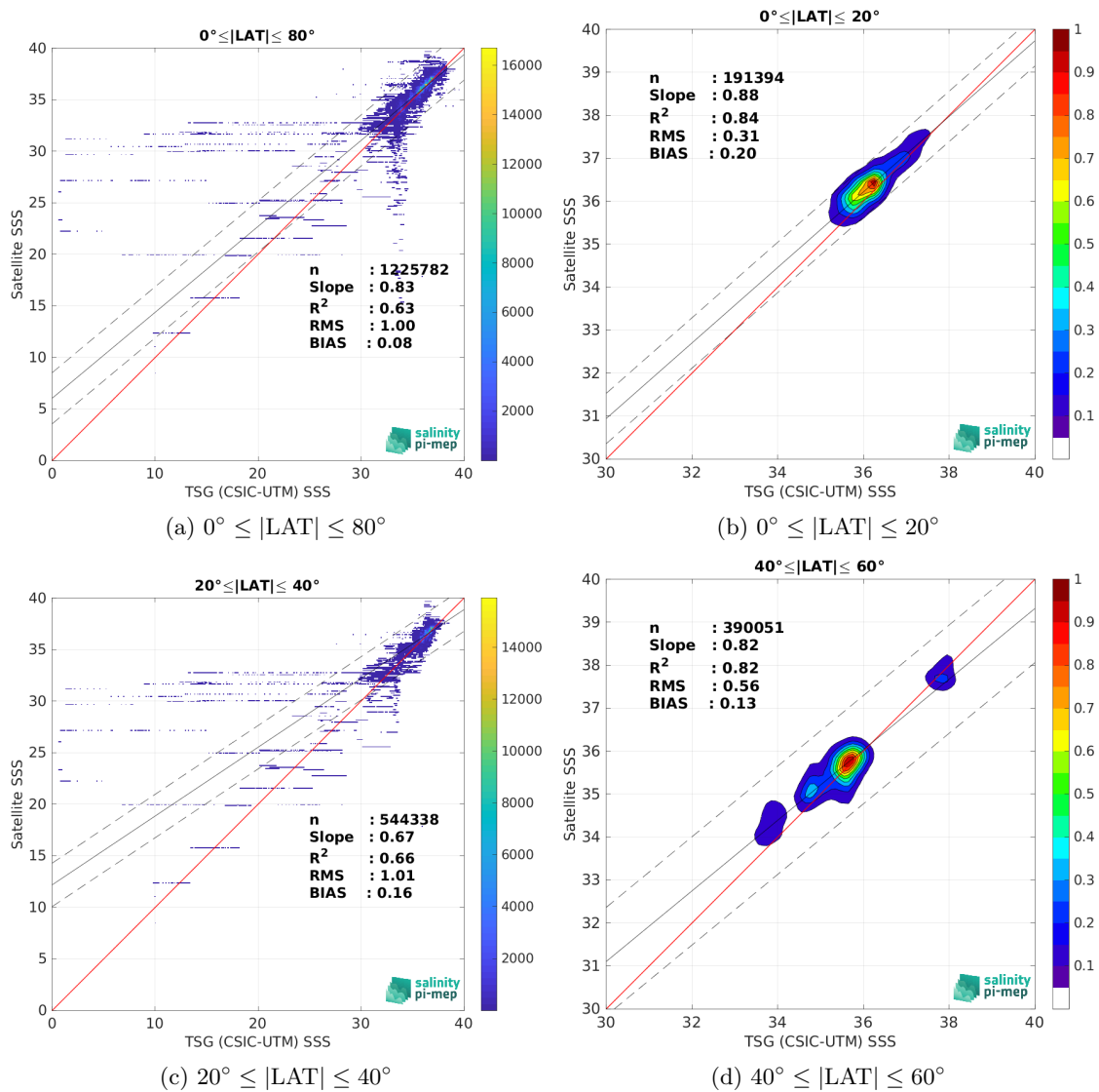
Figure 9: Contour maps of the concentration of SMAP SSS L3 v5.0 - Monthly (JPL) SSS (y-axis) versus TSG (CSIC-UTM) SSS (x-axis) at match-up pairs for different latitude bands. For each plot, the red line shows x=y . The black thin and dashed lines indicate a linear fit through the data cloud and the \pm 95\% confidence levels, respectively. The number match-up pairs n , the slope and R^2 coefficient of the linear fit, the root mean square (RMS) and the mean bias between satellite and in situ data are indicated for each latitude band in each plots.
