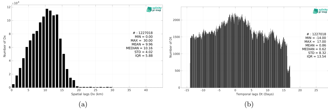
Figure 5: Histograms of the spatial (a) and temporal (b) lags between the location/time of the TSG (CSIC-UTM) measurement and the date of the corresponding SMAP SSS L3 v5.0 - Monthly (JPL) SSS pixel.
