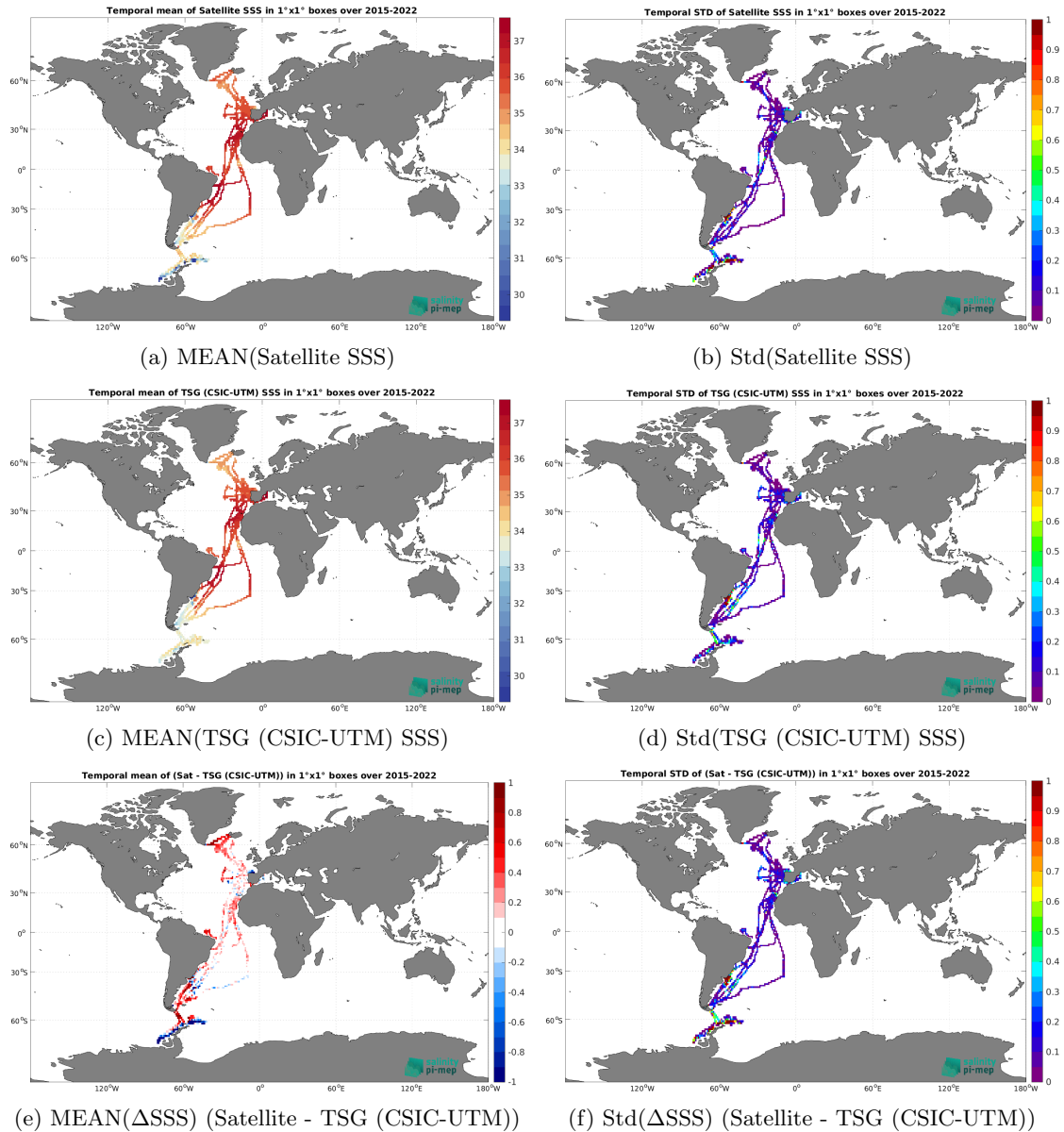
Figure 6: Temporal mean (left) and Std (right) of SSS from SMAP SSS L3 v5.0 - Monthly (JPL) (top), TSG (CSIC-UTM) (middle), and of \Delta SSS (Satellite - TSG (CSIC-UTM)). Only match-up pairs are used to generate these maps.
