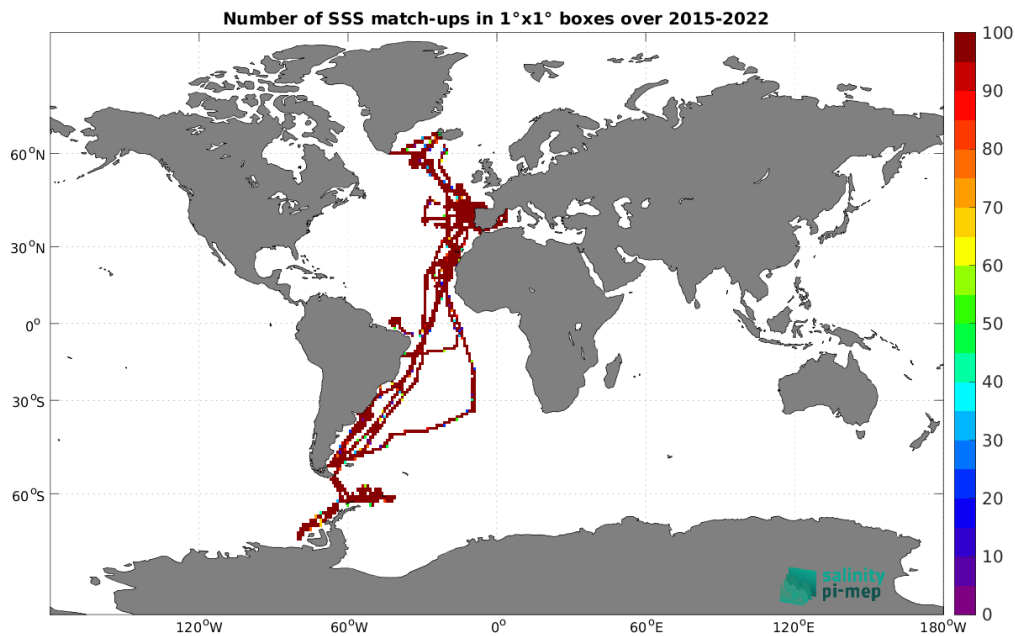
Figure 4: Number of SSS match-ups between TSG (CSIC-UTM) SSS and the SMAP SSS L3 v5.0 - Monthly (JPL) SSS product for the Global Ocean Pi-MEP region over 1^\circ \times 1^\circ boxes and for the full satellite product period.
