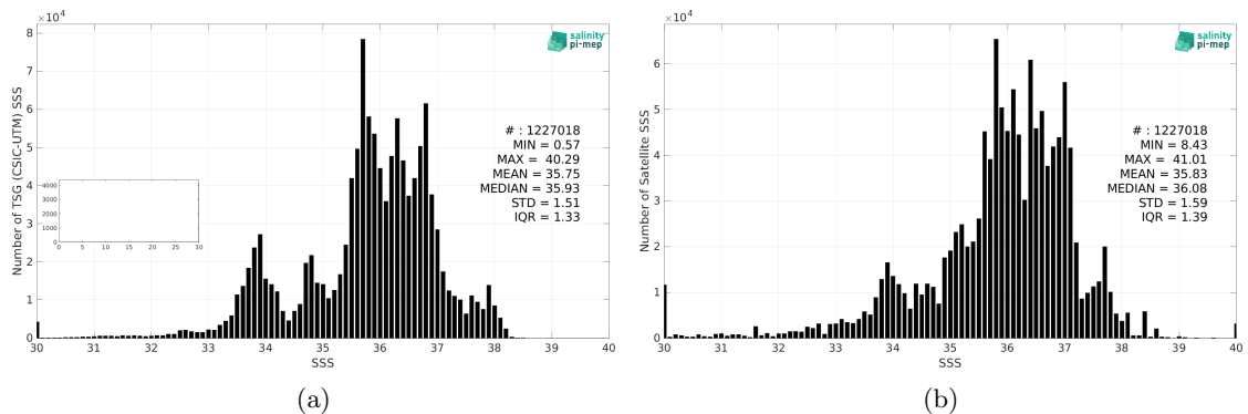
Figure 2: Histograms of SSS from TSG (CSIC-UTM) (a) and SMAP SSS L3 v5.0 - Monthly (JPL) (b) considering all match-up pairs per bins of 0.1 over the Global Ocean Pi-MEP region and for the full satellite product period.
