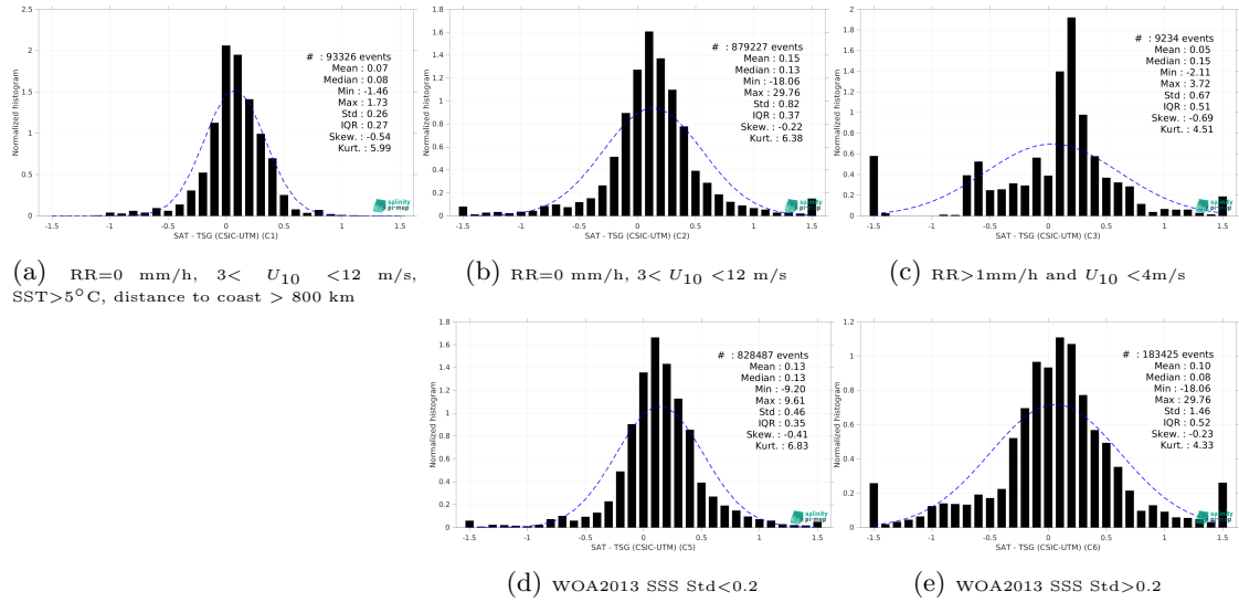
Figure 13: Normalized histogram of \Delta SSS (SMAP SSS L3 v5.0 - Monthly (JPL) - TSG (CSIC-UTM)) for 5 different subdatasets corresponding to: RR=0 mm/h, 3 < U_{10} < 12 m/s, SST>5°C, distance to coast > 800 km (a), RR=0 mm/h, 3 < U_{10} < 12 m/s (b), RR>1mm/h and U_{10} < 4 m/s (c), WOA2013 SSS Std<0.2 (d), WOA2013 SSS Std>0.2 (e).
