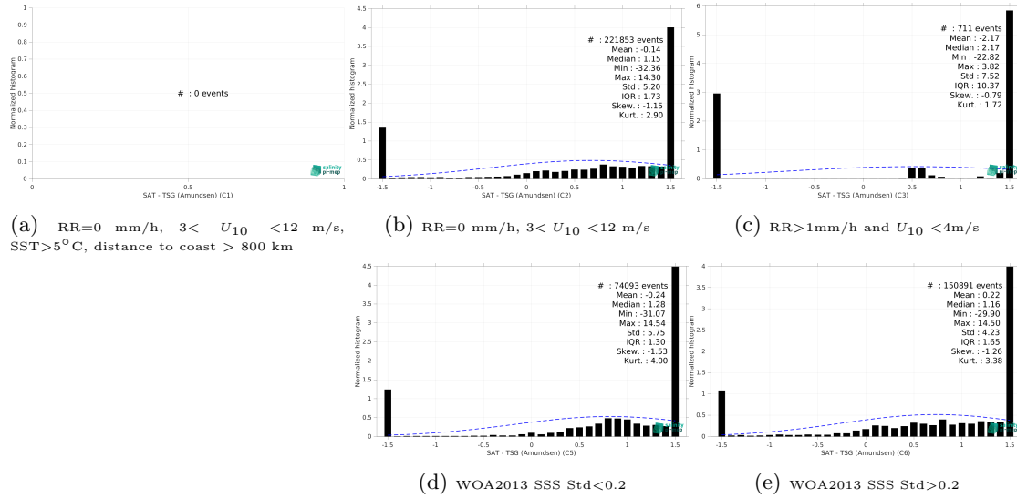
Figure 15: Normalized histogram of \Delta SSS (SMAP SSS L3 v5.0 - Monthly (JPL) - TSG (Amundsen)) for 5 different subdatasets corresponding to: RR=0 mm/h, 3 < U_{10} < 12 m/s, SST>5°C, distance to coast > 800 km (a), RR=0 mm/h, 3 < U_{10} < 12 m/s (b), RR>1mm/h and U_{10} < 4 m/s (c), WOA2013 SSS Std<0.2 (d), WOA2013 SSS Std>0.2 (e).
