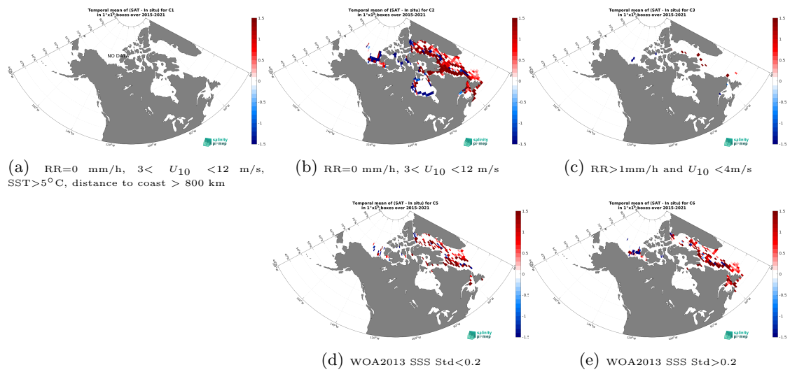
Figure 14: Temporal mean gridded over spatial boxes of size 1^\circ \times 1^\circ of \Delta SSS (SMAP SSS L3 v5.0 - Monthly (JPL) - TSG (Amundsen)) for 5 different subdatasets corresponding to: RR=0 mm/h, 3 < U_{10} < 12 m/s, SST > 5°C, distance to coast > 800 km (a), RR=0 mm/h, 3 < U_{10} < 12 m/s (b), RR > 1mm/h and U_{10} < 4 m/s (c), WOA2013 SSS Std < 0.2 (d), WOA2013 SSS Std > 0.2 (e).
