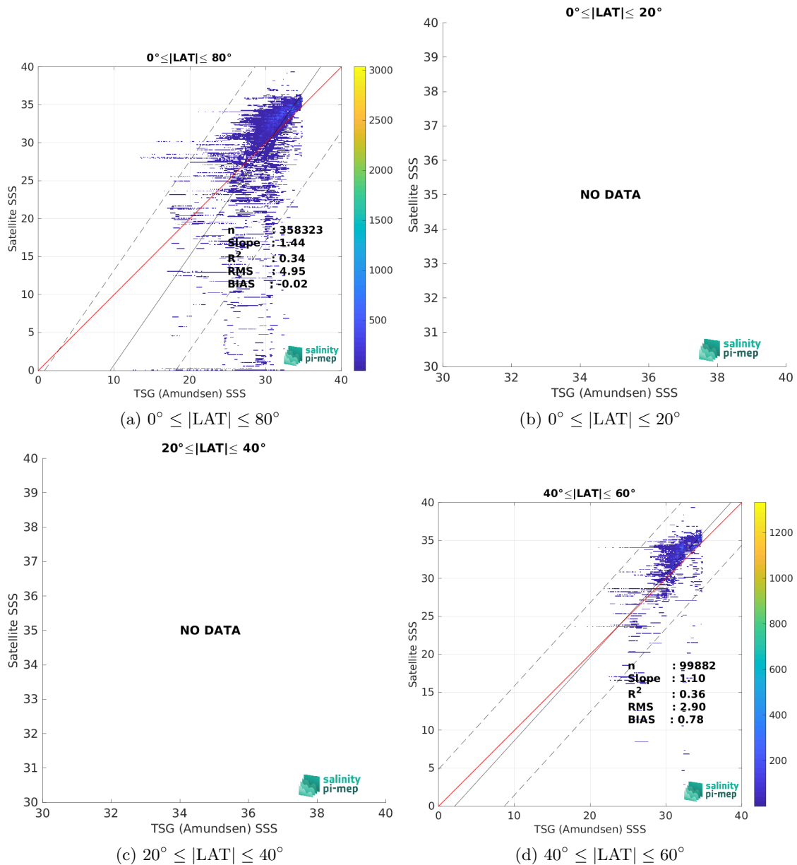
Figure 10: Contour maps of the concentration of SMAP SSS L3 v5.0 - Monthly (JPL) SSS (y-axis) versus TSG (Amundsen) SSS (x-axis) at match-up pairs for different latitude bands. For each plot, the red line shows x=y . The black thin and dashed lines indicate a linear fit through the data cloud and the \pm 95\% confidence levels, respectively. The number match-up pairs n , the slope and R^2 coefficient of the linear fit, the root mean square (RMS) and the mean bias between satellite and in situ data are indicated for each latitude band in each plots.
