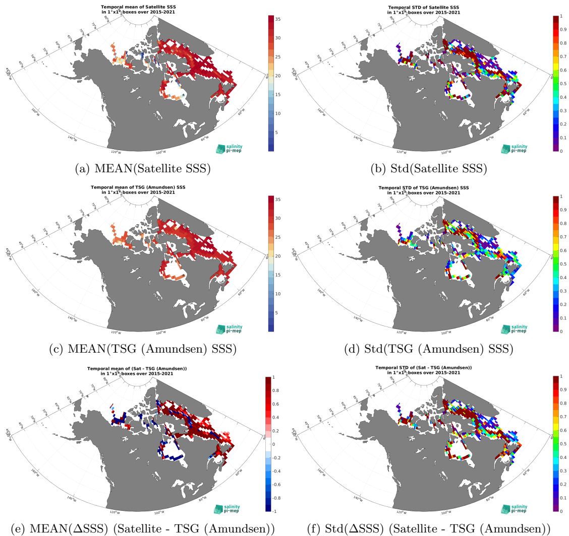
Figure 7: Temporal mean (left) and Std (right) of SSS from SMAP SSS L3 v5.0 - Monthly (JPL) (top), TSG (Amundsen) (middle), and of \Delta SSS (Satellite - TSG (Amundsen)). Only match-up pairs are used to generate these maps.
