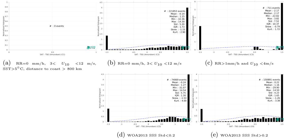
Figure 15: Normalized histogram of \Delta SSS (SMAP SSS L3 v5.0 - Monthly (JPL) - TSG (Amundsen)) for 5 different subdatasets corresponding to: RR=0 mm/h, 3 < U_{10} < 12 m/s, SST > 5°C, distance to coast > 800 km (a), RR=0 mm/h, 3 < U_{10} < 12 m/s (b), RR > 1mm/h and U_{10} < 4 m/s (c), WOA2013 SSS Std < 0.2 (d), WOA2013 SSS Std > 0.2 (e).
