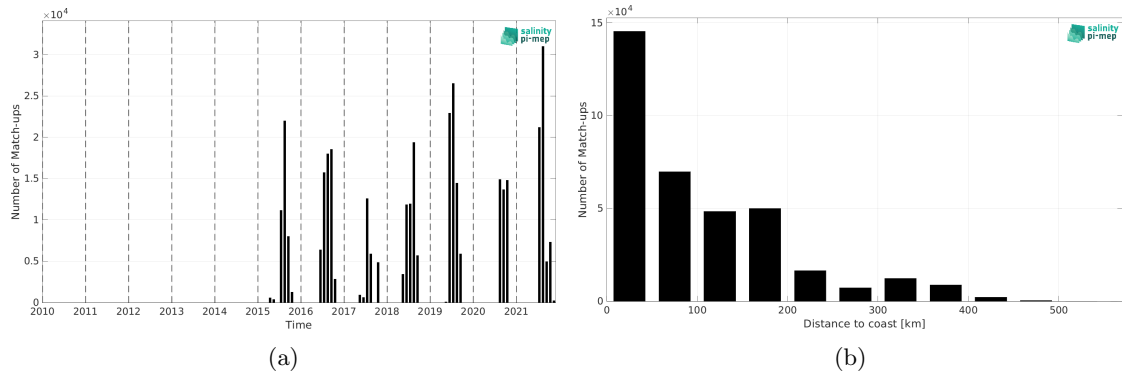
Figure 2: Number of match-ups between TSG (Amundsen) and SMAP SSS L3 v5.0 - Monthly (JPL) SSS as a function of time (a) and as function of the distance to coast (b) over the Global Ocean Pi-MEP region and for the full satellite product period.
