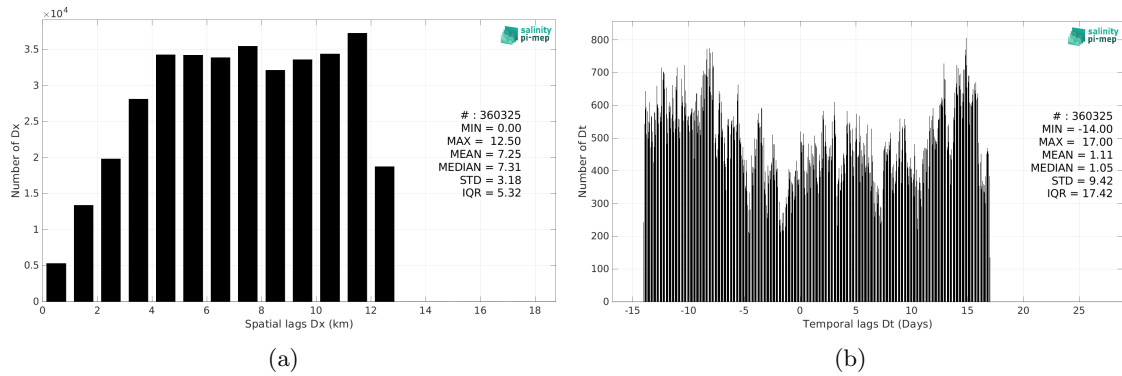
Figure 6: Histograms of the spatial (a) and temporal (b) lags between the location/time of the TSG (Amundsen) measurement and the date of the corresponding SMAP SSS L3 v5.0 - Monthly (JPL) SSS pixel.
