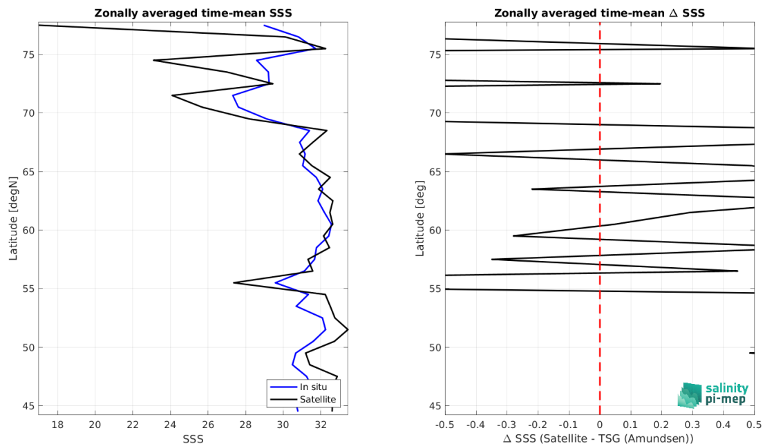
Figure 9: Left panel: Zonal mean SSS from SMAP SSS L3 v5.0 - Monthly (JPL) satellite product (black) and from TSG (Amundsen) (blue). Right panel: Zonal mean of \Delta SSS (Satellite - TSG (Amundsen)) for all the collected Pi-MEP match-up pairs estimated over the full satellite product period.
