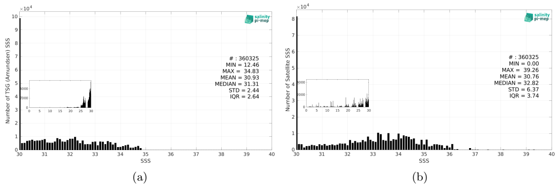
Figure 3: Histograms of SSS from TSG (Amundsen) (a) and SMAP SSS L3 v5.0 - Monthly (JPL) (b) considering all match-up pairs per bins of 0.1 over the Global Ocean Pi-MEP region and for the full satellite product period.
