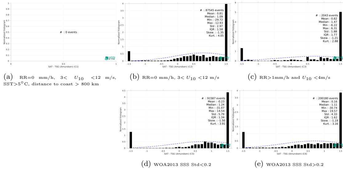
Figure 13: Normalized histogram of \Delta\text{SSS} (SMAP SSS L3 v5.0 - Monthly (JPL) - TSG (Amundsen)) for 5 different subdatasets corresponding to: RR=0 mm/h, 3 < U_{10} < 12 m/s, SST > 5^\circ\text{C} , distance to coast > 800 km (a), RR=0 mm/h, 3 < U_{10} < 12 m/s (b), RR > 1\text{mm/h} and U_{10} < 4\text{m/s} (c), WOA2013 SSS Std < 0.2 (d), WOA2013 SSS Std > 0.2 (e).
