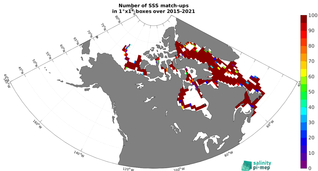
Figure 4: Number of SSS match-ups between TSG (Amundsen) SSS and the SMAP SSS L3 v5.0 - Monthly (JPL) SSS product for the Global Ocean Pi-MEP region over 1^\circ \times 1^\circ boxes and for the full satellite product period.
