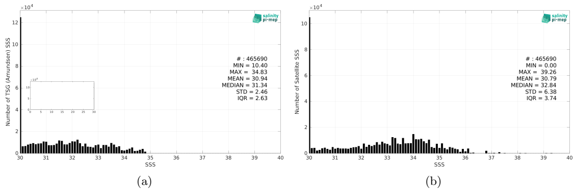
Figure 2: Histograms of SSS from TSG (Amundsen) (a) and SMAP SSS L3 v5.0 - Monthly (JPL) (b) considering all match-up pairs per bins of 0.1 over the Global Ocean Pi-MEP region and for the full satellite product period.
