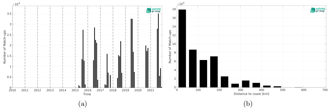
Figure 1: Number of match-ups between TSG (Amundsen) and SMAP SSS L3 v5.0 - Monthly (JPL) SSS as a function of time (a) and as function of the distance to coast (b) over the Global Ocean Pi-MEP region and for the full satellite product period.
